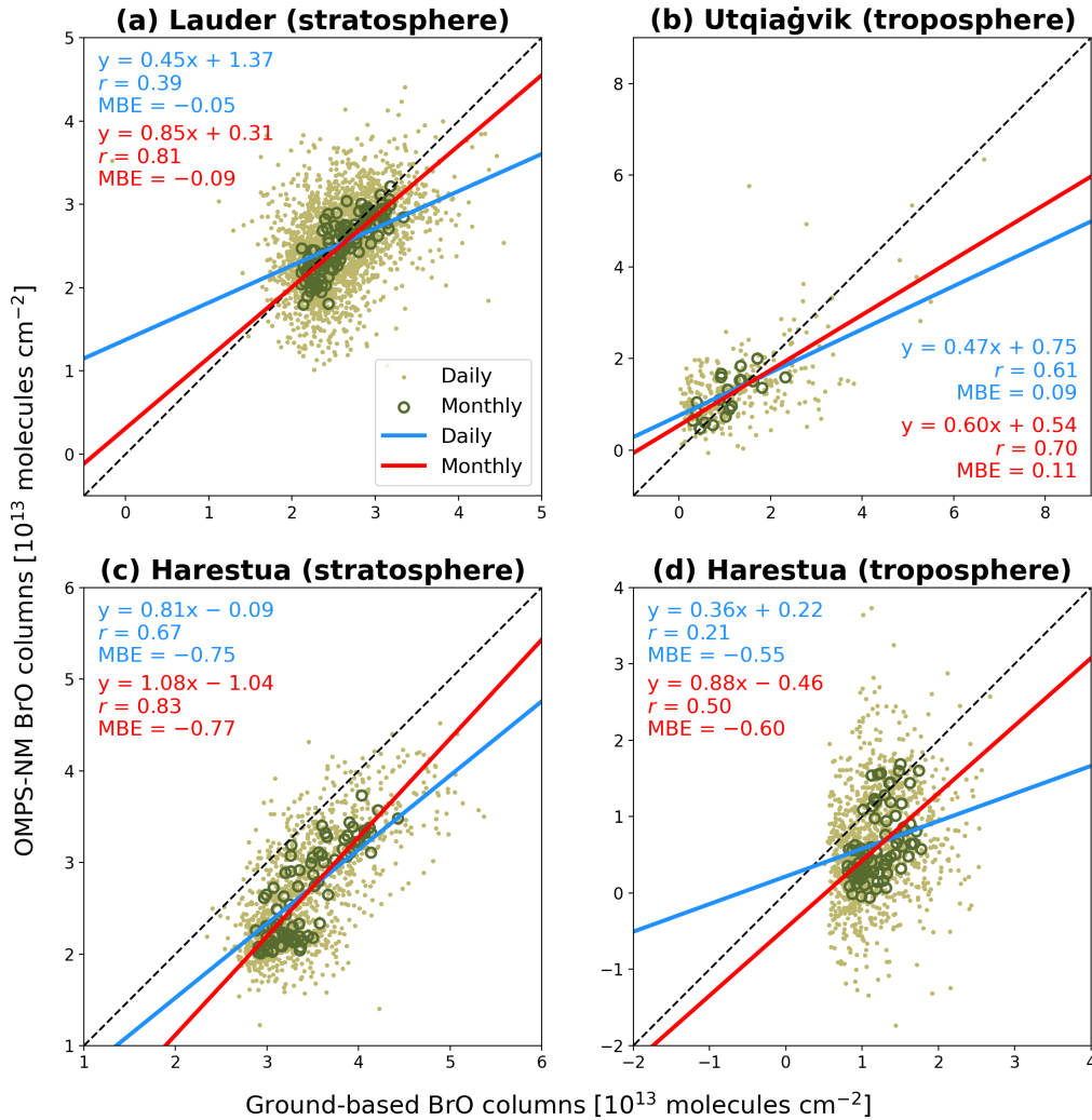
Figure 9. Scatter plots of ground-based versus OMPS-NM BrO retrievals. The station name and the target column (stratosphere or troposphere) are indicated above each panel. Monthly and daily data and their regression lines are overlaid (see the legend for description). Slopes and intercepts of regression lines, correlation coefficients ( r ), and mean bias errors (MBEs) are also indicated.
