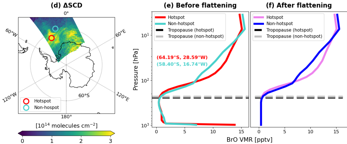
Figure 4. BrO profiles before and after flattening. Four OMPS-NM pixels are selected from sea ice locations in the Northern Hemisphere (o7594, 15 April 2013) and Southern Hemisphere (o9765, 15 September 2013). Panels (a) and (d) show the locations of these pixels overlaid on BrO \Delta SCDs retrieved from the two orbits. Red and blue (cyan) circles on the maps represent hotspots and non-hotspots, respectively. Their BrO vertical profiles before flattening are presented in panels (b) and (e), using the same color code as in panels (a) and (d). The profiles after flattening are shown in panels (c) and (f). Tropopause pressures are indicated in black and gray dashed lines. The description of each line is shown in the legend. Latitudes and longitudes of the selected pixels are also indicated.
