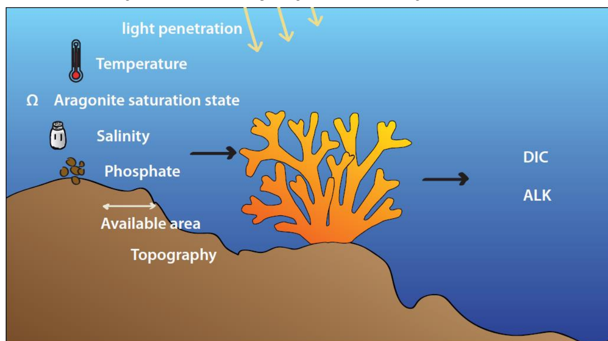
Figure 1. Summary of all variables governing carbonate production in the iCORAL coral reef module (left) and the variables that are impacted by carbonate production (right).
