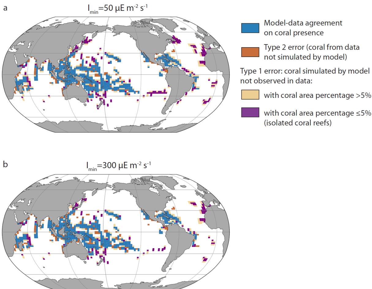
325 Figure 5. Coral location in the model and data for the minimum and maximum I_{\min} (the minimum light intensity necessary for reef growth) values. Blue cells indicate the presence of corals in both model and observational data, brown cells indicate the presence of corals in observational data but not in the model simulation, beige and purple indicate the presence of corals in the model simulation
