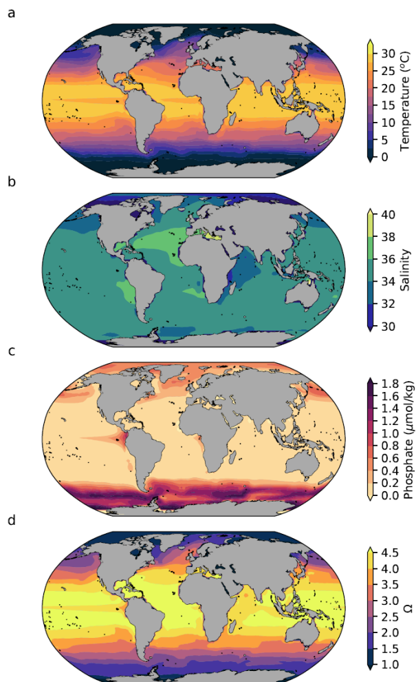
Figure 3. Surface ocean (a) temperature (°C), (b) salinity, (c) phosphate concentration ( \mu\text{mol kg}^{-1} ) and (d) aragonite saturation state ( \Omega ) simulated by iLOVECLIM in pre-industrial conditions. The model outputs are 100-year averages at the end of the equilibrium pre-industrial simulation.
