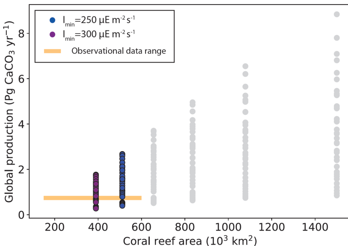
Figure 8. Global carbonate production ( \text{Pg CaCO}_3 \text{ yr}^{-1} ) as a function of global coral reef area ( 10^3 \text{ km}^2 ).
