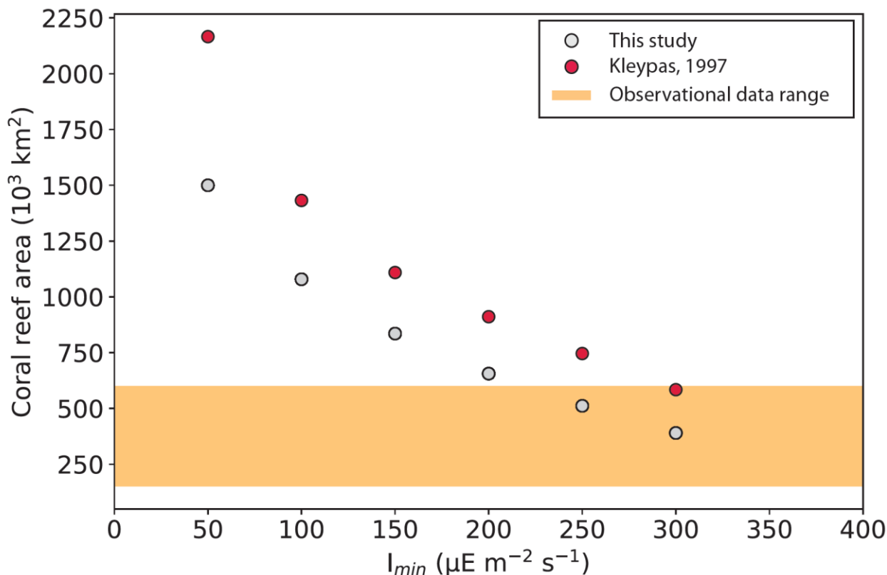
Figure 6. Global coral reef area ( 10^3 \text{ km}^2 ) simulated in this study and in Kleypas (1997) as a function of I_{min} (the minimum light intensity necessary for reef growth, \mu\text{E m}^{-2} \text{s}^{-1} ). The range of observational data for the global coral reef area (section 2.4) is shown with the yellow bar.
