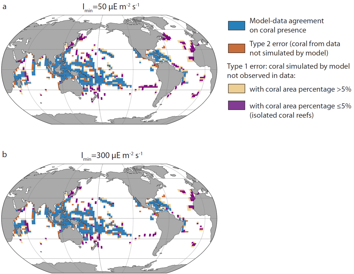
365 Figure 4. Coral location in the model and data for the minimum and maximum I_{min} (the minimum light intensity necessary for reef growth) values. Blue cells indicate the presence of corals in both model and observational data, brown cells indicate the presence of corals in observational data but not in the model simulation, beige and purple indicate the presence of corals in the model simulation but not in observations. Some locations correspond to places with very small surface areas (purple, due to small islands for example) but as we plot the presence of corals in the relatively large oceanic grid cells (the horizontal ocean resolution is 3^{\circ} \times 3^{\circ} ) it might give the impression of large coral coverage.
