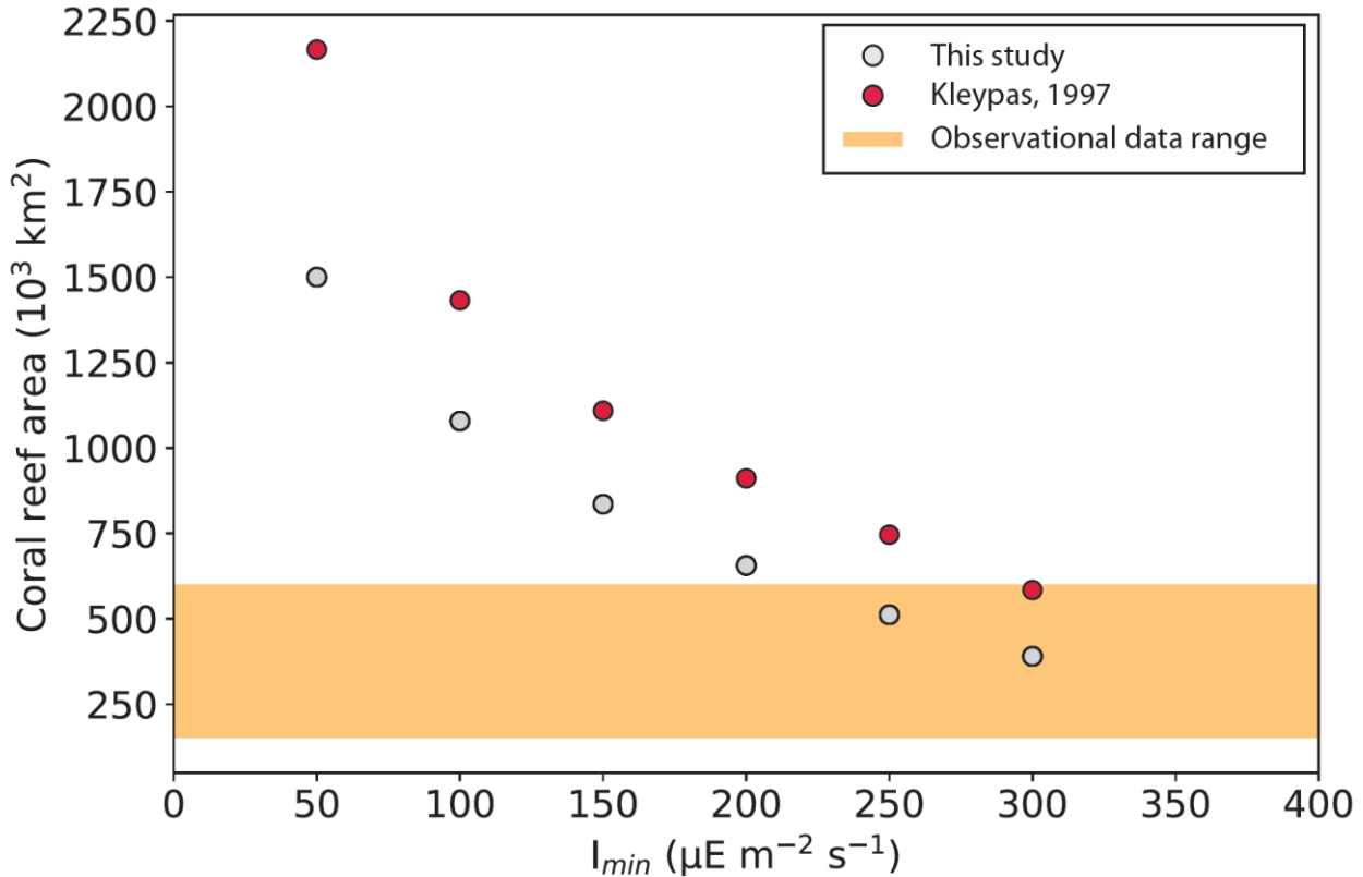
390 Figure 5. Global coral reef area ( 10^3 \text{ km}^2 ) simulated in this study and in Kleypas (1997) as a function of I_{min} (the minimum light intensity necessary for reef growth, \mu\text{E m}^{-2} \text{s}^{-1} ). The range of observational data for the global coral reef area (section 2.4) is shown with the yellow bar.
