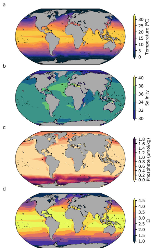
335 Figure 2. Surface (5m depth) ocean (a) temperature ( ^{\circ}\text{C} ), (b) salinity, (c) phosphate concentration ( \mu\text{mol kg}^{-1} ) and (d) aragonite saturation state ( \Omega ) simulated by iLOVECLIM in pre-industrial conditions. The model outputs are 100-year averages at the end of the equilibrium pre-industrial simulation.
