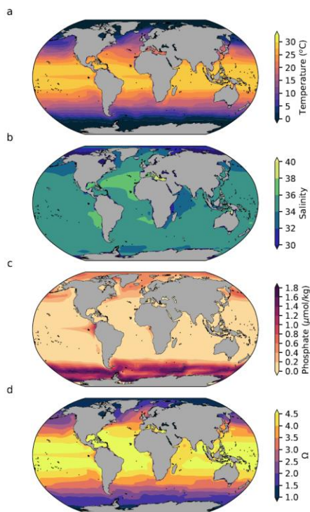
340 Figure 23. Surface (5m depth) ocean (a) temperature (°C), (b) salinity, (c) phosphate concentration ( \mu\text{mol kg}^{-1} ) and (d) aragonite saturation state ( \Omega ) simulated by iLOVECLIM in pre-industrial conditions. The model outputs are 100-year averages at the end of the equilibrium pre-industrial simulation.
