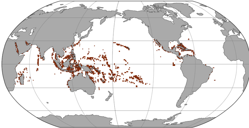
330 Figure 12: Coral location from UNEP-WCMC (2018) dataset. Brown cells indicate the presence of coral reefs in these cells. In white grid cells no coral reef has been detected.
