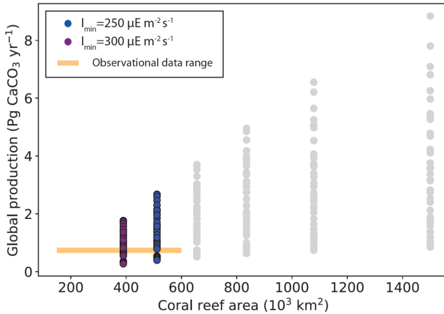
Figure 78. Global carbonate production ( \text{Pg CaCO}_3 \text{ yr}^{-1} ) as a function of global coral reef area ( 10^3 \text{ km}^2 ).
