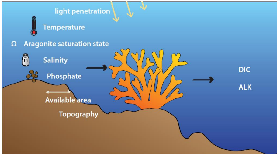
115 Figure 1. Summary of all variables governing carbonate production in the iLOVECLIM coral module (left) and the variables that are impacted by carbonate production (right).
