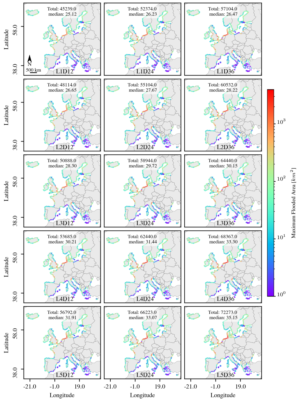
Figure 4. Maximum flooded areas for each coastal sector in km 2 .
