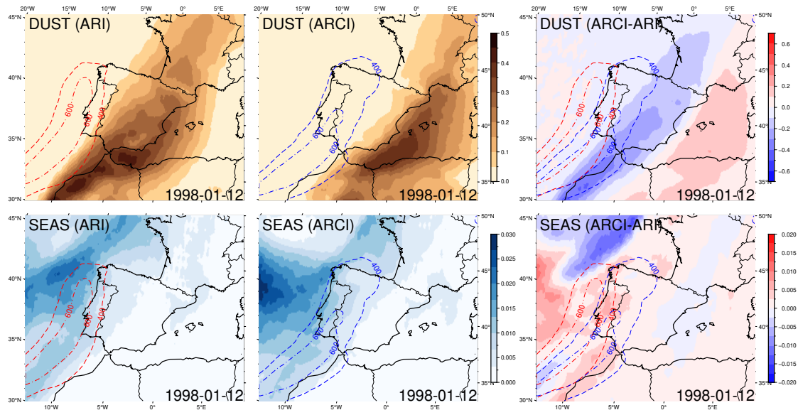
Figure 17. 09:00 h, 12 January 1998. ARI and ARCI dust (top) and sea salt (bottom) AOD at 550 nm and ARCI-ARI AOD differences. Red and blue contours show ARI and ARCI ARs respectively (400 and 600 \text{kg m}^{-1} \text{s}^{-1} IVT levels).
