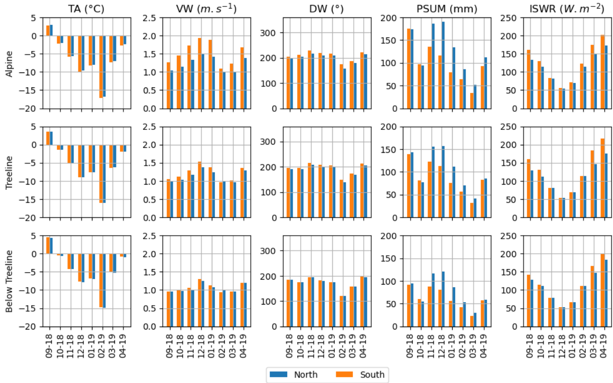
Figure 7. Intra-cell spatial variability of subgridded atmospheric parameters for season 2018–2019. Each row represents monthly averages for each atmospheric variable and cumulative precipitations, for each elevation band. Blue bars correspond to the North aspect, orange bars correspond to the South aspect.
