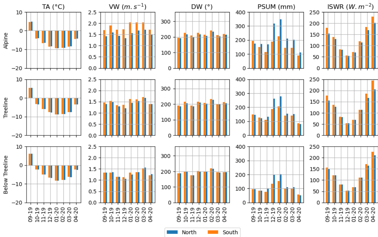
Figure A1. Intra-cell spatial variability of subgridded atmospheric parameters for season 2019-2020. Each row represents monthly averages for each atmospheric variable and cumulative precipitations, for each elevation band. Blue bars correspond to the North aspect, orange bars correspond to the South aspect.
