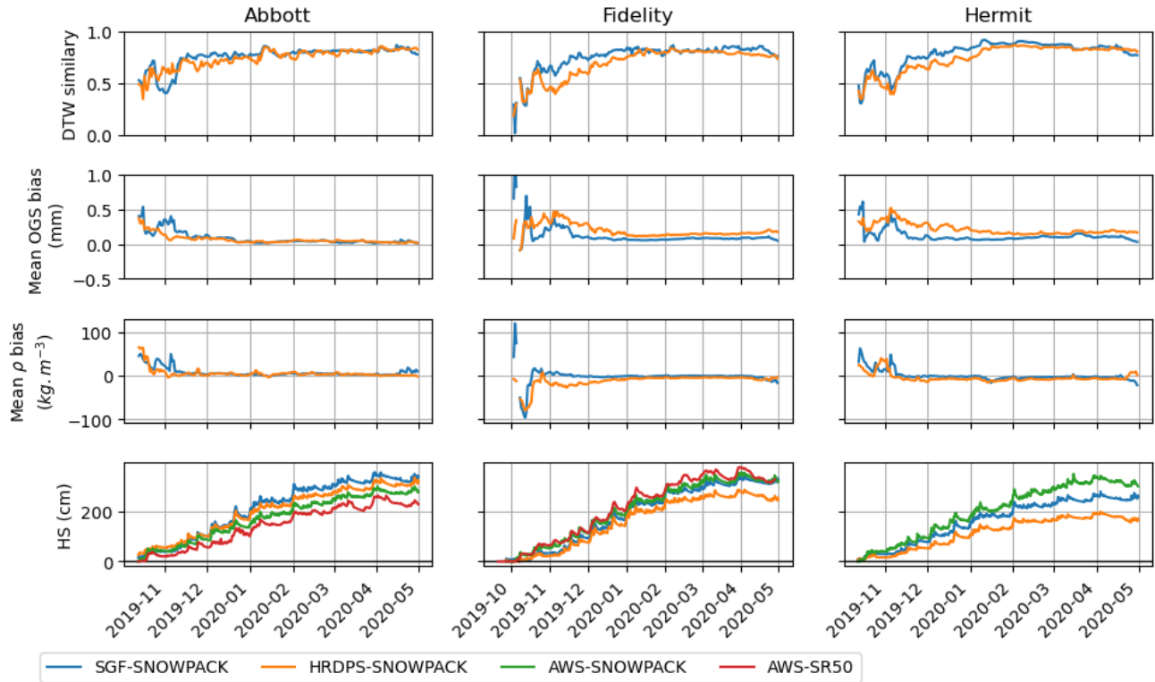
Figure 5. Snowpack similarity assessment for season 2019-2020. The first row shows DTW similarity for each station, the second shows bias in OGS with respect AWS-SNOWPACK, the third shows density bias with respect to AWS-SNOWPACK, and the last row shows simulated HS (and measured when available). The blue curves refer to SGF-SNOWPACK, the orange curves to HRDPS-SNOWPACK, and the green curves to AWS-SNOWPACK. In the HS plots for Abbott and Fidelity, the red curves refer to SR50 measurements at the station plot.
