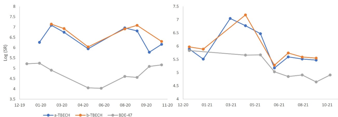
Figure S18 The seasonal variation of the logarithmic water (precipitation)-air fugacity ratios of \alpha - and \beta -TBECH and BDE-47 in Saturna Island (left) and Tadoussac (right).
