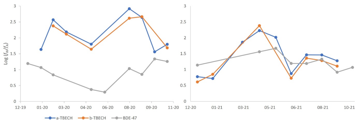
Figure S17 The seasonal variation of the logarithmic scavenging ratios (SRs) of \alpha - and \beta -TBECH and BDE-47 in Saturna Island (left) and Tadoussac (right).
