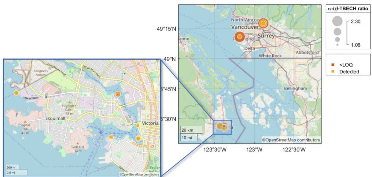
Figure S11 The spatial distribution of the \alpha/\beta -TBECH ratios at the PWS sites in British Columbia. A close-up map of the Victoria is shown (left) for a detailed view of the clustered sites. To calculate the ratios, only measurements that were above the LOD for both isomers were used, including measurements that were above the LOD but below the LOQ. To distinguish their certainty, ratios that were calculated using quantifiable measurements and ratios that were calculated using at least one measurement below the LOQ are marked in yellow and orange, respectively.
