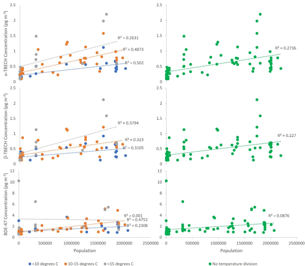
Figure S5 The relationship between the air concentration of \alpha -TBECH (top), \beta -TBECH (middle), and BDE-47 (bottom) in the British Columbia PAS sites and the population in a 20-km radius around the sites. Sites were divided based on the average air temperature during their deployment length (left) and compared to the overall sample set (right) for each chemical.
