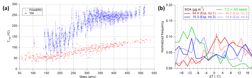
Figure 7. (a) T_{\text{max}} for \alpha -pinene SOA measured by the VIA–NO 3 -CIMS system (blue markers for the mean and light blue whiskers for the one standard deviation) and the FIGAERO-iodide-CIMS adapted from Ylisirniö et al. (2020). (b) The normalized distribution of T_{\text{max}} difference ( \Delta T ) between each experiment and the mean of five experiments for HOMs. In panel (b), only the 7.2\ \mu\text{g m}^{-3} SOA experiment was conducted using ammonium sulfate as the seed particles.
