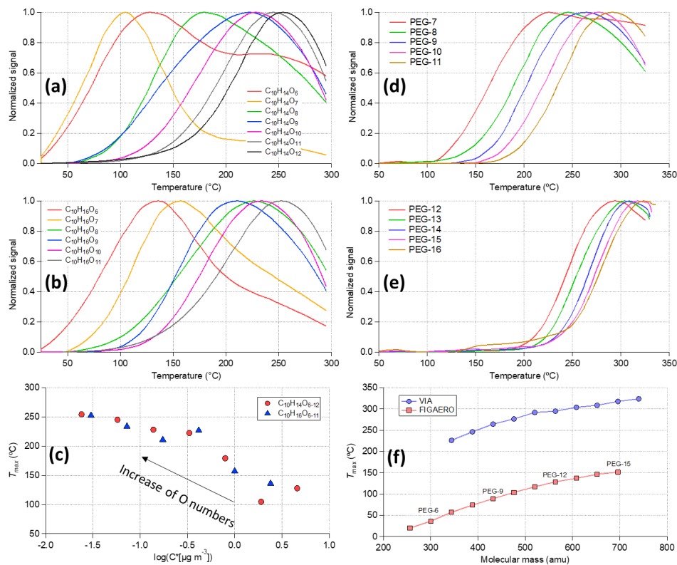
390 Figure 6. Thermogram of (a) C_{10}H_{14}O_{6-12} , (b) C_{10}H_{16}O_{6-11} , and (d, e) polyethylene glycols (PEGs). (c) The scattering plot of T_{max} obtained from panels (a) and (b) vs. the estimated saturation vapor concentration using the composition-determined empirical expression in Peräkylä et al. (2020). (f) T_{max} as a function of molecular mass (atomic mass unit) for PEGs measured by the VIA– NO_3 -CIMS and the FIGAERO-iodide-CIMS (Ylisirniö et al., 2021).
