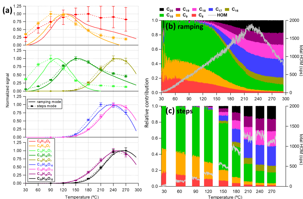
370 Figure 5. Comparison of measurements obtained between the ramping and the steps mode for (a) thermogram of some chosen HOM monomers and dimers, and (b, c) the relative contributions of different C number families to the total HOM signals. In (a), smoothed signals are shown for the ramping mode (“Loess” algorithm with a bandwidth of 0.25 and the second order local polynomial was used), while the mean (diamond markers) and standard deviation (bottom and top whiskers) are shown for the steps mode. The thermograms are normalized to the reagent ions first and then to their maximums. The raw signals of the same dataset are given in Fig. S10. 375
