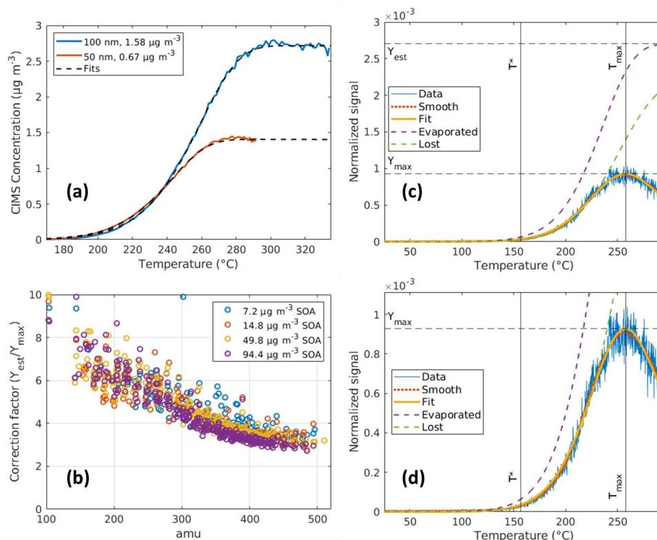
450 Figure 8: Fitting results of the observed thermogram for (a) sulfuric acid and (c) C 20 H 30 O 12 . (b) Summary of the correction factor (CF) for the VIA–NO 3 -CIMS system in terms of particle-phase HOMs measurement, the mass dependency of these curves make sense because heavier HOMs evaporate later, thus smaller correction is needed. (d) The same result as panel (c) but zoomed in on the details to show the agreement between the fit and measurement. In panel (c), the “Data” curve is the measured signal of C 20 H 30 O 12 normalized to the reagent ions. The “Smooth” curve used less smoothing with a bandwidth of 0.25 on the data. The “Evaporated” curve represents the estimated signal without gas phase losses using Eq. 1, which shows the estimated maximum signal (Y est ). The “Lost” curve describes the cumulated diffusional vapor losses (assuming 100% loss once a molecule hit the wall) within the VIA vaporization tube. The “Fit” curve displays the calculated gas-phase signal as the difference between the “Evaporated” and “Lost” curves. More examples of the fitting result for other HOMs and the fitted parameters (T* and k) are shown in Figure S14 and S15, respectively.
