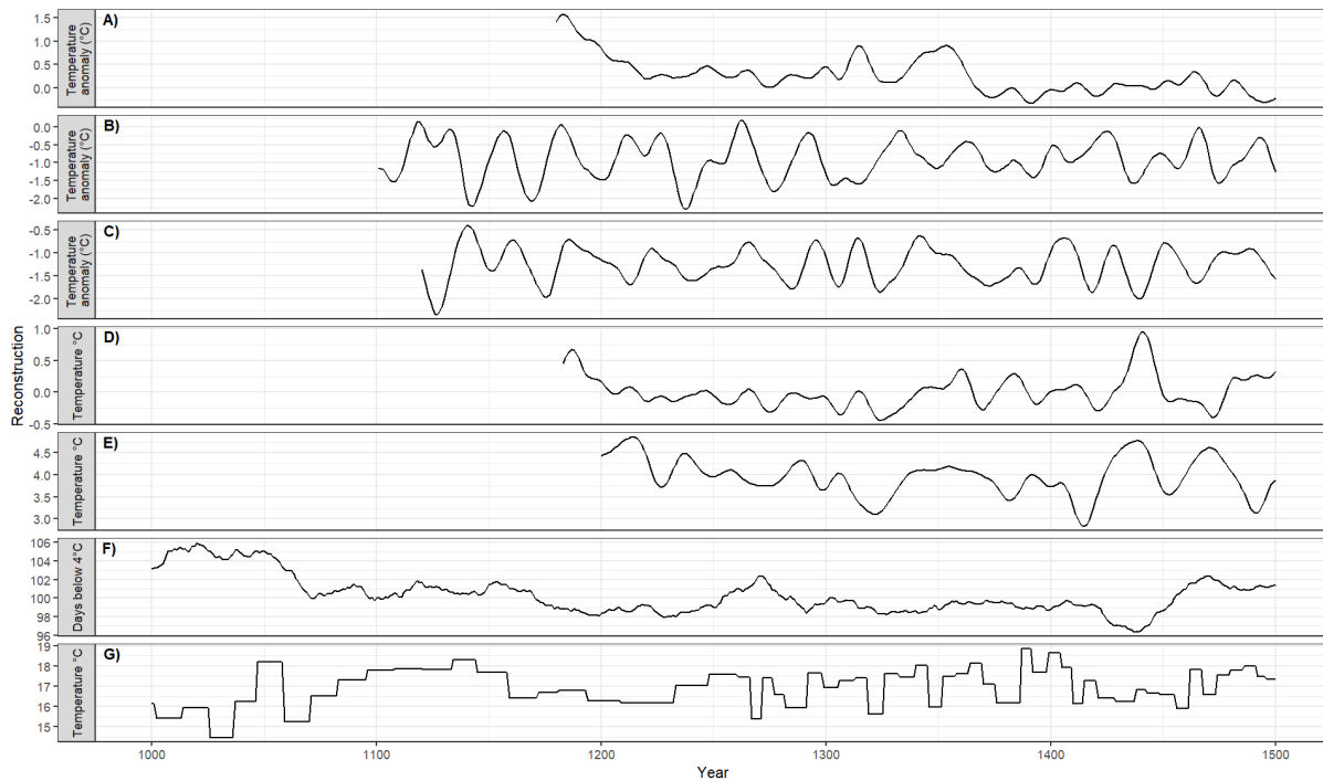
865 Figure 10. Reconstruction of air temperature in Poland in moving windows: A) Feb–Mar temperature anomaly in a Gaussian 20-year moving window for Kuyavia-Pomerania region. B) Feb–Mar temperature anomaly in a Gaussian 20-year moving window for the Lesser Poland region. C) Dec–Mar temperature anomaly in a Gaussian 20-year moving window for the Lesser Poland region. D) Feb–Mar temperature anomaly in a Gaussian 20-year moving window for Kuyavia-Pomerania (modified after Koprowski et al. 2012). E) Nov–Apr temperature anomaly in a Gaussian 20-year moving window for northern Poland (modified after Balanzategui et al. 2017). F) chrysophyte-based reconstruction of number of days below 4 °C (Hernández-Almeida et al. 2015). G) chironomid-based reconstruction of August temperature (Hernández-Almeida et al. 2017)
