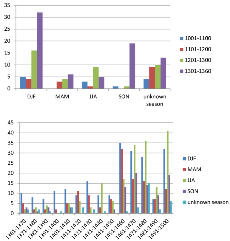
830 Figure 2. Number of weather notes/excerpts for Poland available in historical sources in the periods: above , AD 1001–1360; below , AD 1361–1500
