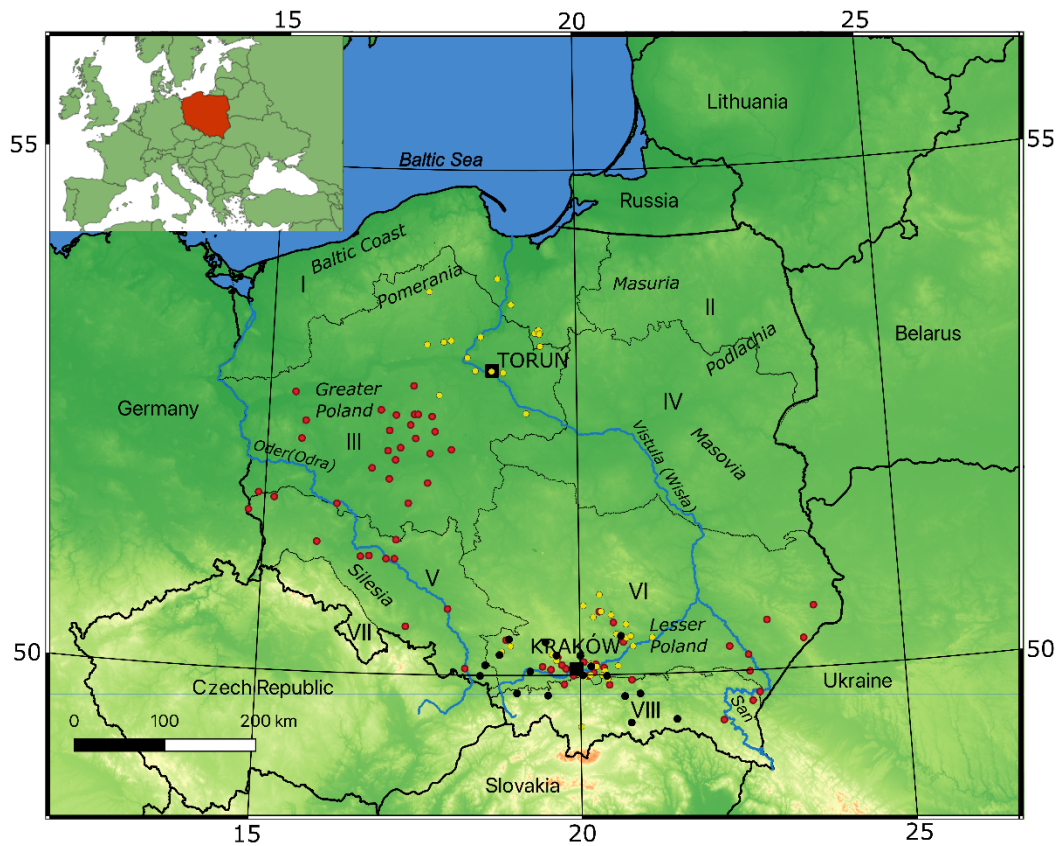
825 Figure 1. Study area with historical and natural-forest regionalisation and location of materials used for research. Natural-Forest Provinces (Zielony and Kliczkowska 2012): I – Baltic Coast province II – Masuria–Podlachia province, III – Greater Poland–Pomerania province, IV – Masovia–Podlachia province, V – Silesia province, VI – Lesser Poland province, VII – Sudetia province, VIII – Carpathia province. Dendrochronological sites: yellow dots – pine, red dots – oak, black dots – fir. Black squares – meteorological stations
