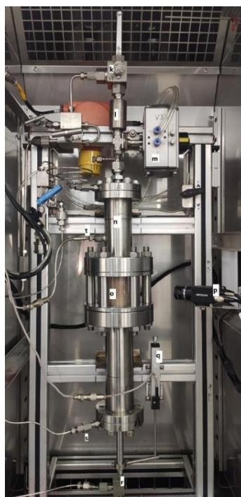
90 Figure 4 The inside-view of the air bath: (k) Hopper valve; (l) Proppant warehouse; (m) Electric valve of proppant warehouse; (n) Up chamber of the sapphire reactor; (o) Sapphire window of the sapphire reactor; (p) Camera; (q) Strain sensor; (r) Pore pressure valve and safety valve; (s) Stress valve; (t) Temperature sensor.
