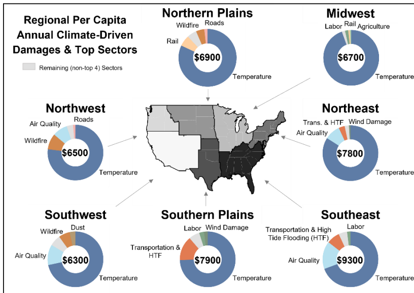
395 Figure 5: Mean per capita annual climate-driven damages across the seven regions in 2090 for the subset of climate impacts included in FrEDI. Donut charts show the annual per capita damages (2020$ per person annually) and the top four sectors with the largest damages in each region. All damages from remaining (non-top four) sectors are shown by the light gray wedges.
