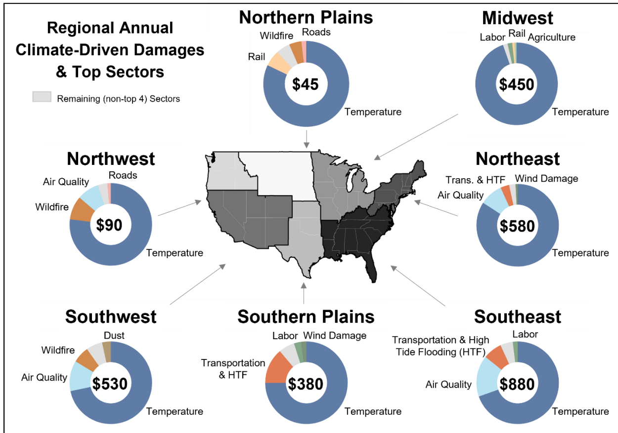
Figure A3. Map of mean annual climate-driven damages for a subset of sectors across 10,000 projections in each of the seven U.S. regions in the year 2090 (undiscounted). Damages are in billions of 2020USD. Donut charts show the absolute damages (in billions) in each region for those sectors included in FrEDI, and the top four sectors with the largest annual climate-driven damages. The share of damages from all remaining sectors are shown by the light gray wedge.
