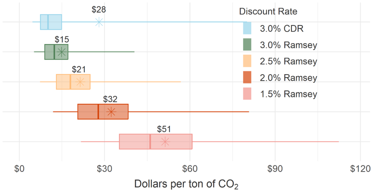
Figure A5. Net present value of future damages from one tonne of CO 2 for damages occurring only within the CONUS. Units are in dollars (2020 USD) per ton of CO 2 emitted. 'CDR' refers to Constant Discount Rate. Whiskers represent the 2.5 th and 97.5 th percentiles, while boxes span the 25 th to 75 th . Mean values (stars and text) along with median values (vertical lines) are also shown.
