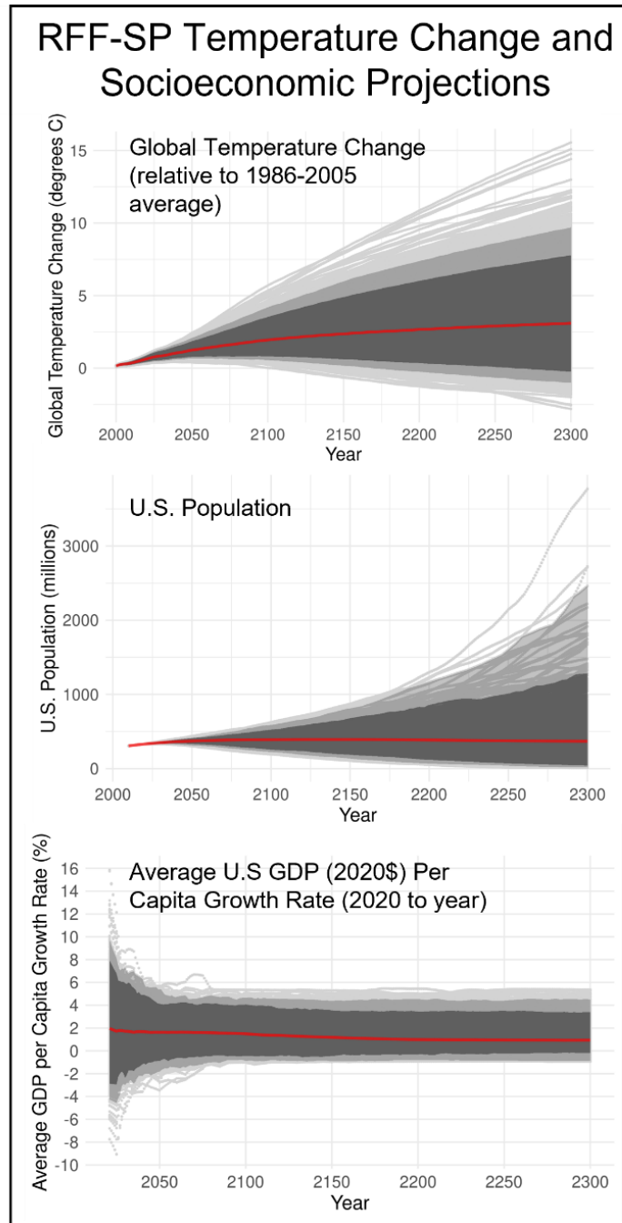
515 Figure A1. Timeseries of global mean temperature (°C) relative to 1986-2005 baseline, U.S. population (millions), and average U.S. GDP per capita growth rate (2020$) for the 10,000 RFF-SP scenarios from 2020-2300. Temperature trajectories are derived from FaIR model runs of the 10,000 RFF-SP emission scenarios. Individual scenarios are shown by light gray lines. Medium and dark gray shaded regions represent the 99 th and 95 th percent confidence intervals, respectively. The red line is the mean value overtime.
