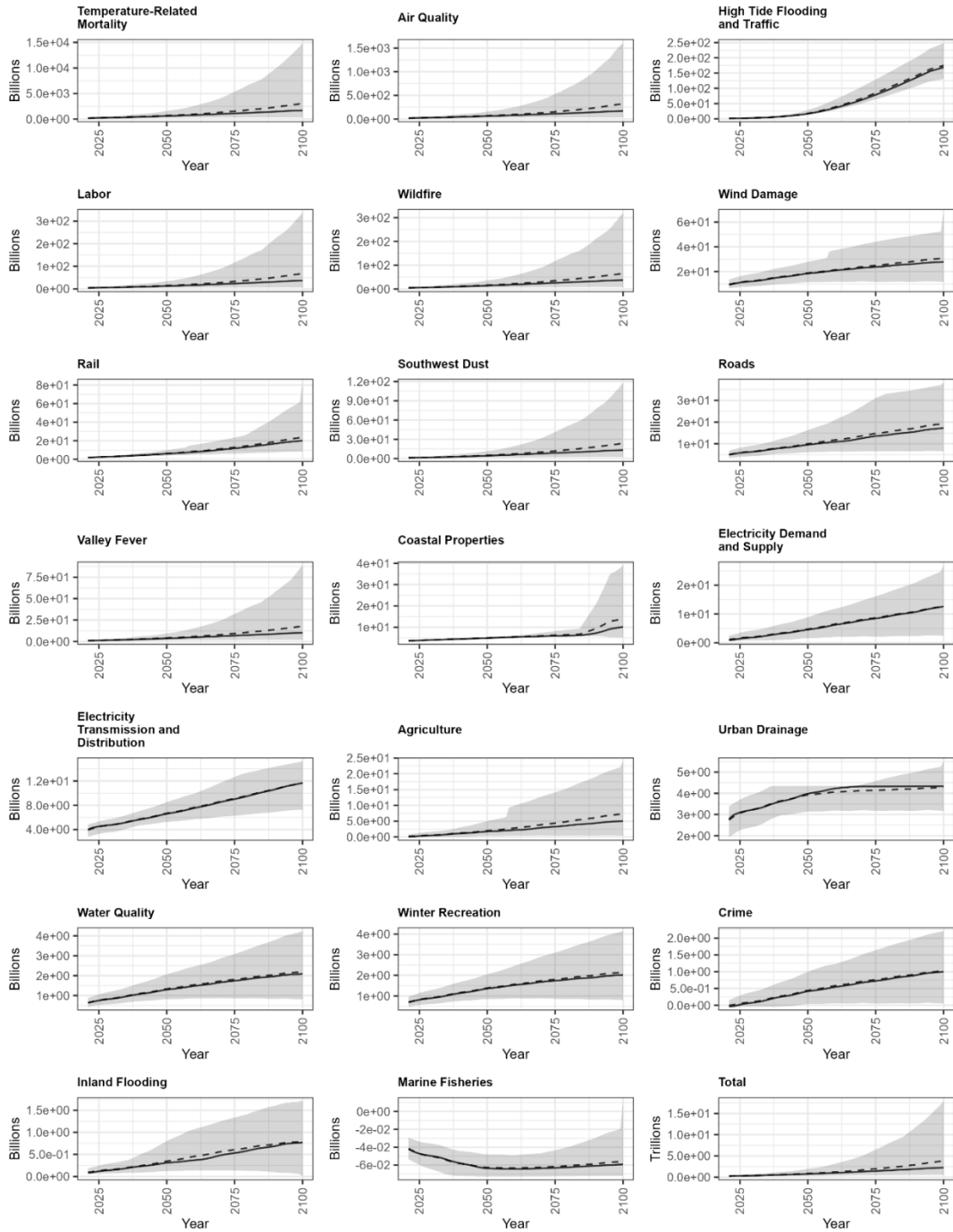
525 Figure A2. Timeseries of sectoral damages in billions of 2020 USD across all 10,000 projections through 2100. Ordered by decreasing mean damages in the year 2090. Total damages (trillions) from all sectors in the lower right panel. Lines show annual mean (dashed) and median (solid) damages. Shaded areas show the 95% CI.. Temporal trends are a function of the underlying temperature (or sea level rise) binned damage functions, as well as sector specific scalars (e.g., per capita income- dependent VSL). Slight discontinuities in some of these sectors (e.g., agriculture) can occur either at the boundary between 530 temperature bins (e.g., for agriculture and wind damage) or due to thresholds in the underlying studies. For example, the sharp increase in damages in the coastal property damage sector after 2080 are correspond to a sharp increase in damages that occur after sea levels breach 100 cm.
