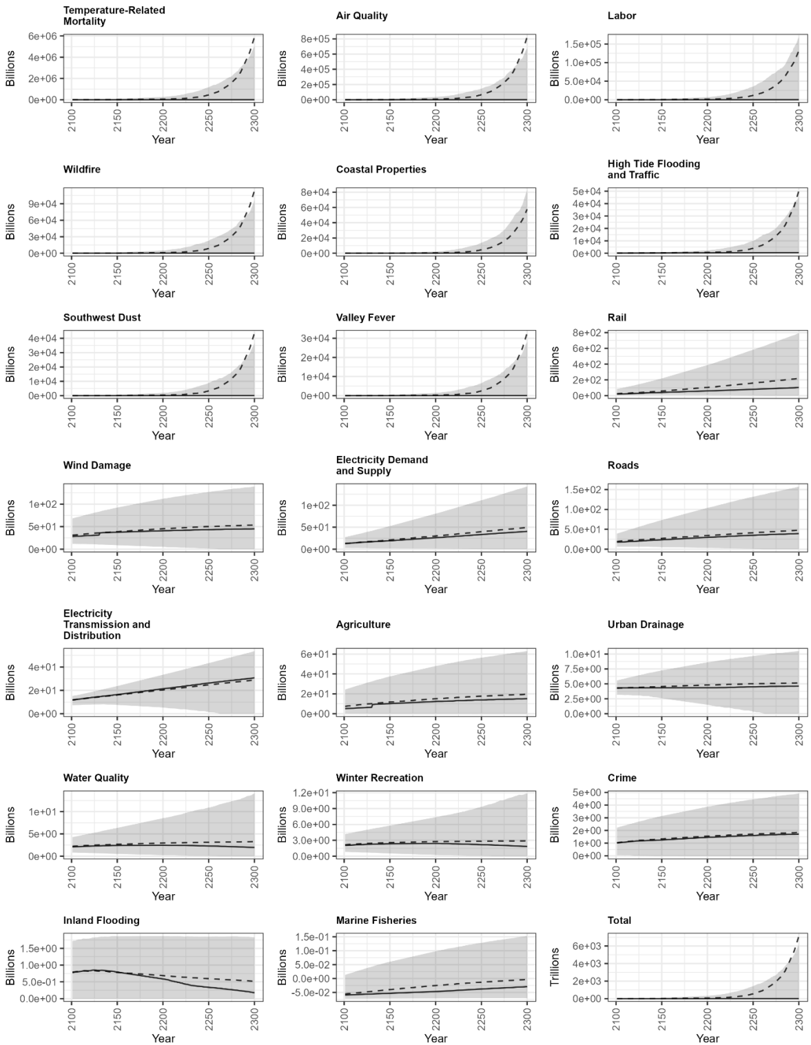
Figure A4. Timeseries of sectoral damages across all 10,000 projections from 2100-2300. Ordered by decreasing mean damages in the year 2300. The lower right panel shows total damages summed across all sectors. Dashed line (solid) shows the mean (median) damages each year. Shaded areas show the 95% CI. Annual damages are in units of billions of 2020USD (trillions for total panel).
