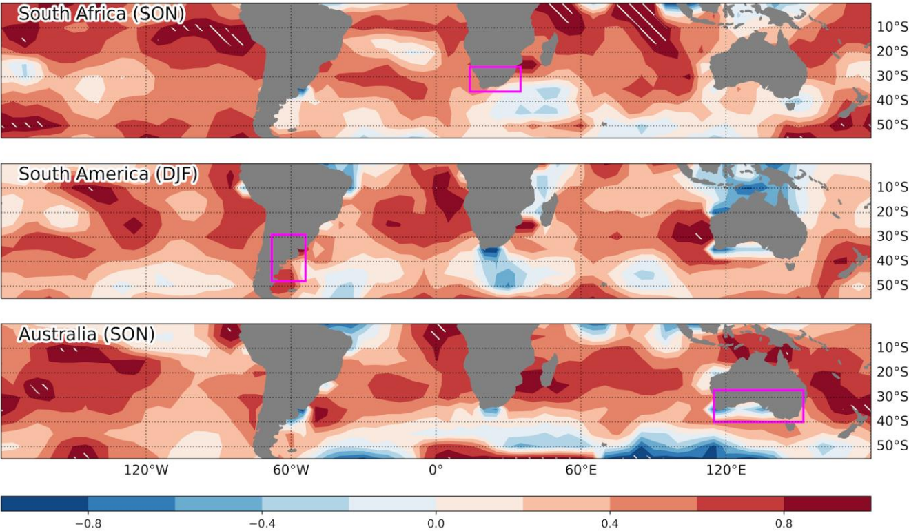
395 396 Figure 11: Same as in Fig. 10, but for SST trends (1980-2010; heterogeneous correlation; shading) based on a subset of reanalyses 397 (ERA5, ERA-Interim, JRA-55, MERRA-2, NCEP-NCAR).
