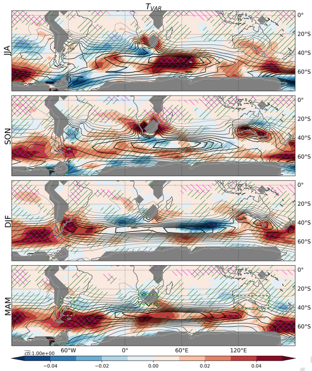
Figure 5. Trends of T_{\text{VAR}} (shading; \text{K}^2 \text{yr}^{-1} ) during 1980–2022 are shown for the REM for the different seasons (rows). The climatology is overlaid with contour lines at 2 \text{K}^2 intervals. Thicker contours indicate larger magnitudes. Significant trends ( p < 0.05 ) are indicated with purple hatching. Areas where more than one third of reanalyses agree on the sign of the trends are hatched in green.
