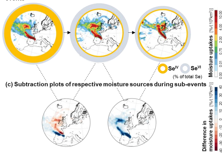
Fig. 6. Inorganic Se speciation in precipitation and cloud water as a function of dominating moisture sources. (a) Proportions of \text{Se}^{\text{IV}} (% total Se) as a function of pH in precipitation (blue circles) and cloud water (grey circles) during the high-resolution campaign in 2019. Size of data points correspond to proportions of Atlantic moisture sources (% total moisture sources). (b) Evolution of proportions of inorganic Se species, \text{Se}^{\text{IV}} (yellow) and \text{Se}^{\text{VI}} (grey) during sub-precipitation events (P17.1: 270 min, P17.2: 380 min, P17.3: 110 min duration) with corresponding moisture source plots (shown in colour scale 0-10 %/ 10^5 \text{ km}^2 ). (c) Subtraction plots of relative moisture source changes (shown in red-blue colour scale from -40 to 40 %/ 10^5 \text{ km}^2 ) during sub-precipitation events shown in (b).
