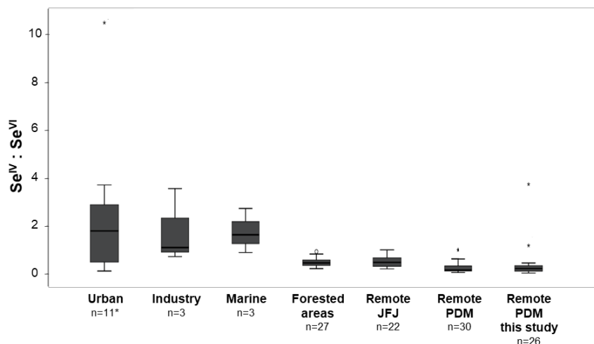
Fig. 7. Previously reported ratios of Se IV to Se VI concentrations classified by sampling sites: urban, industry, marine, forested area, remote. Number of data points indicated for each source class is indicated by n. *Urban data derived from 5 different studies (Cutter, 1978; Cutter and Church, 1986; Wang et al., 1994; Wallschläger and London, 2004; Donner and Siddique, 2018). Other classifications comprise data from industry (De Gregori et al., 2002), marine (Cutter and Church, 1986) and forested areas (Roulier et al., 2021). Remote data refers to this study and previous study by Suess et al. (2019) conducted on two high altitude stations: Jungfraujoeh (JFJ, Switzerland) and Pic du Midi (PDM, France).
