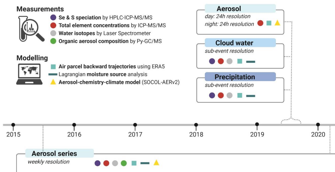
140 Fig. 1. Overview of the measurements and modelling approaches applied to the 2015-2020 aerosol time series and 2019 campaign, in which aerosol, cloud water and precipitation samples were collected. Figure created with BioRender.com.
