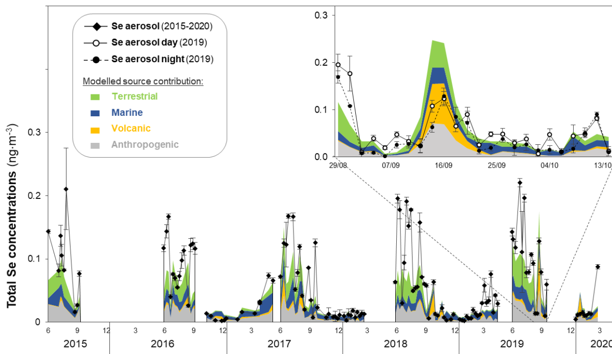
375 Fig. 2. Comparison of Se aerosol measurement with modelled Se data. Data shown for 2015-2020 aerosol time series (filled diamond) as well as day (outlined circles with continuous line) and night (filled circles with dashed line) aerosol measurements in 2019 campaign (campaign period shown in top right corner). Modelled source contributions by SOCOL-AERv2 are shown as stacked areas, including biogenic terrestrial (green), marine (blue), volcanic (yellow) and anthropogenic activities (grey).
