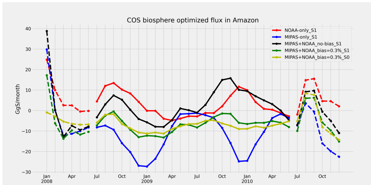
Figure R3. The biosphere COS flux over the Amazon on a monthly time scale after optimization for different inversions in 2008-2010. The dashed lines indicate the spin-up and spin-down periods.
