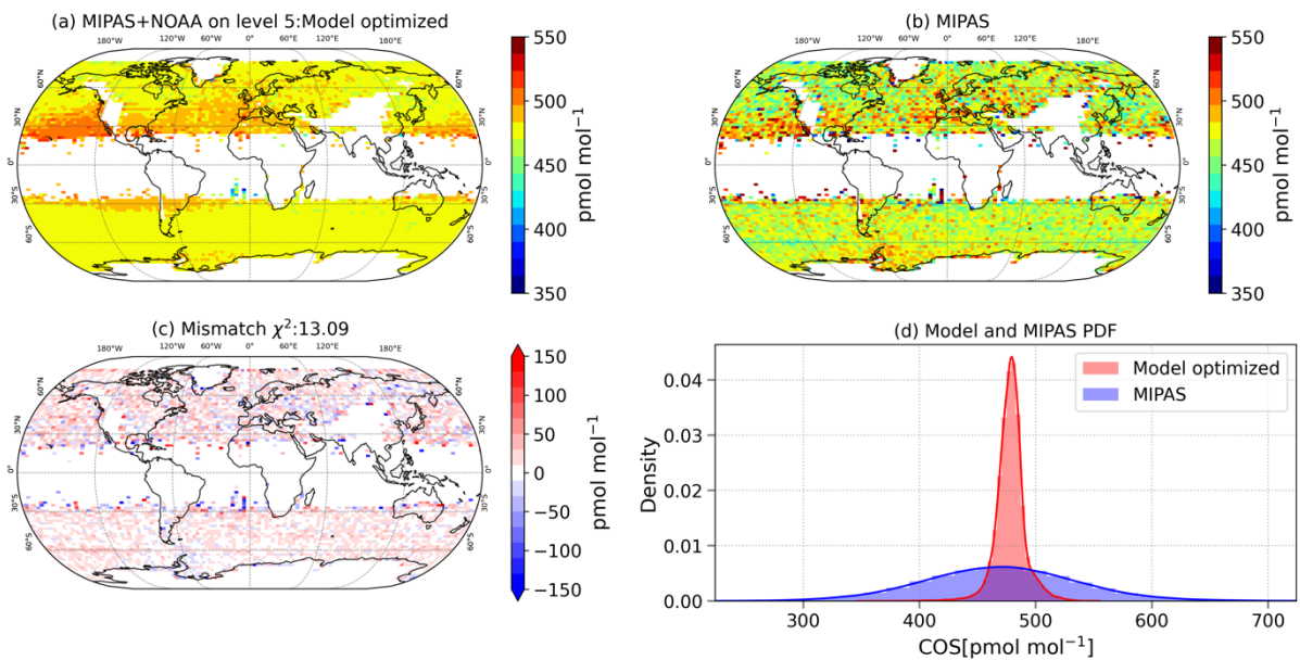
Figure R2. The MIPAS+NOAA S1 inversion using level 5 (numbering starting from 0) of MIPAS.
