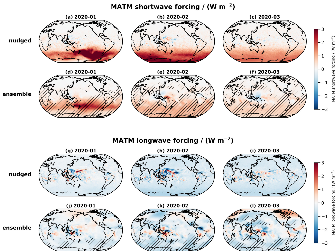
Figure 1. Convergence of monthly average radiative flux perturbations (difference between FIRE1 and FIRE0) between TOA and 200 hPa, abbreviated as middle atmosphere (MATM) forcing. The upper two rows from (a) to (f) present shortwave MATM forcing, the lower two rows from (g) to (l) are longwave MATM forcing. Time is increasing from left to right as indicated in the sub-panel titles, from January to March 2020. Average results from nudged (1st and 3rd row) and ensemble (2nd and 4th row) simulations are compared. Hatching represents areas in which the ensemble mean perturbations are different from zero at 95% confidence level.
