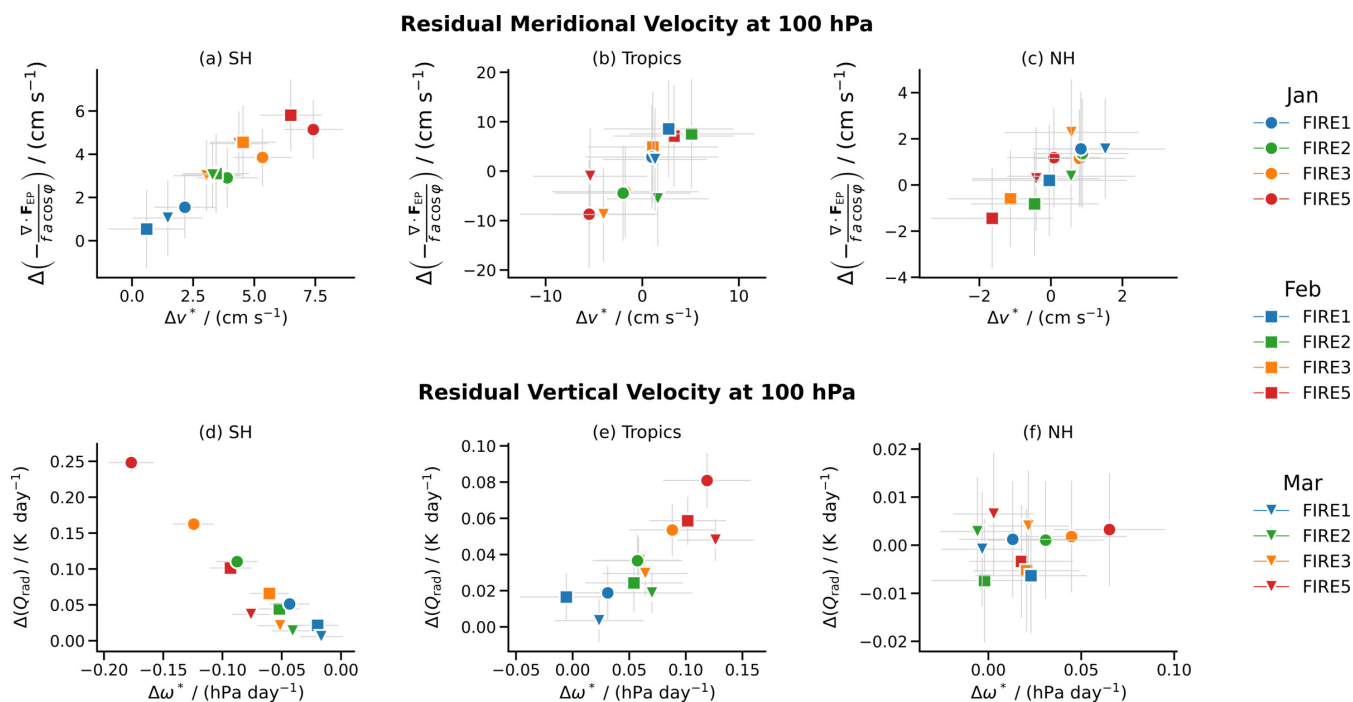
Figure 8. Relationship between components of the residual circulation and the forcing by large-scale waves (1st row) or the radiative heating (2nd row). Symbols mark monthly and regionally averaged anomalies with colors indicating fire strength from FIRE1 (blue) to FIRE5 (red) and symbol style for different months: January (circle), February (square) and March (triangle). Gray error bars indicate the 95% confidence interval. Regions are split by \varphi = 20^\circ\text{S} and \varphi = 20^\circ\text{N} where \varphi represents latitude.
