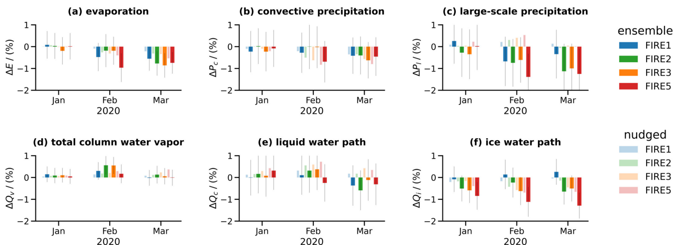
Figure 11. Globally and monthly average perturbations of (a) surface evaporation fluxes, (b) convective precipitation, (c) large-scale precipitation, (d) total column water vapor Q_v , (e) liquid water path Q_c , and (f) ice water path Q_i as function of time. All perturbations are computed relative to the FIRE0 run as reference and presented in %. Colors from blue to red indicated perturbation resulting from fire perturbation runs FIRE1, FIRE2, FIRE3 and FIRE5. Bright colors indicate data from ensemble simulations, whereas light colors represent nudged data shown side-by-side for the respective runs.
