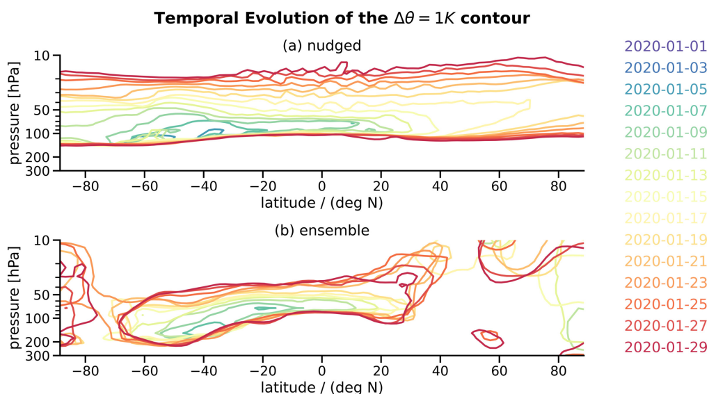
Figure 5. Temporal evolution of the potential temperature perturbation for the FIRE1 case with respect to the FIRE0 case. Shown is the 1-K contour of the average potential temperature perturbation for the (a) nudged simulations and (b) ensemble simulation that is color-coded by time (see legend). Each second day is presented beginning with 1 Jan 2020. Please note that the pressure starts at 300 hPa at the vertical axis.
