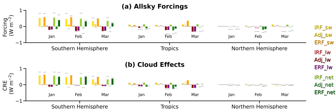
Figure 3. (a) All-sky forcings and (b) cloud effects averaged over specified geographical regions (outer interval on x-axis), over all months (inner interval on x-axis) and over all fire strength perturbations. The different components of the effective radiative forcing (ERF) are represented by differently colored bars. ERF is split into instantaneous radiative forcing (IRF) and adjustments (Adj) and also decomposed into shortwave and longwave components. Each bar represents the average of ensemble mean values for the four normalized fire perturbation experiments. Values for which the standard deviation among the four perturbation experiments is larger than the actual mean value are indicated by light colors. Data from the nudged experiments are shown as small gray horizontal lines for comparison and are also calculated as average over all normalized fire perturbations. Regions are split at \varphi = 20^\circ\text{S} and \varphi = 20^\circ\text{N} where \varphi represents latitude.
