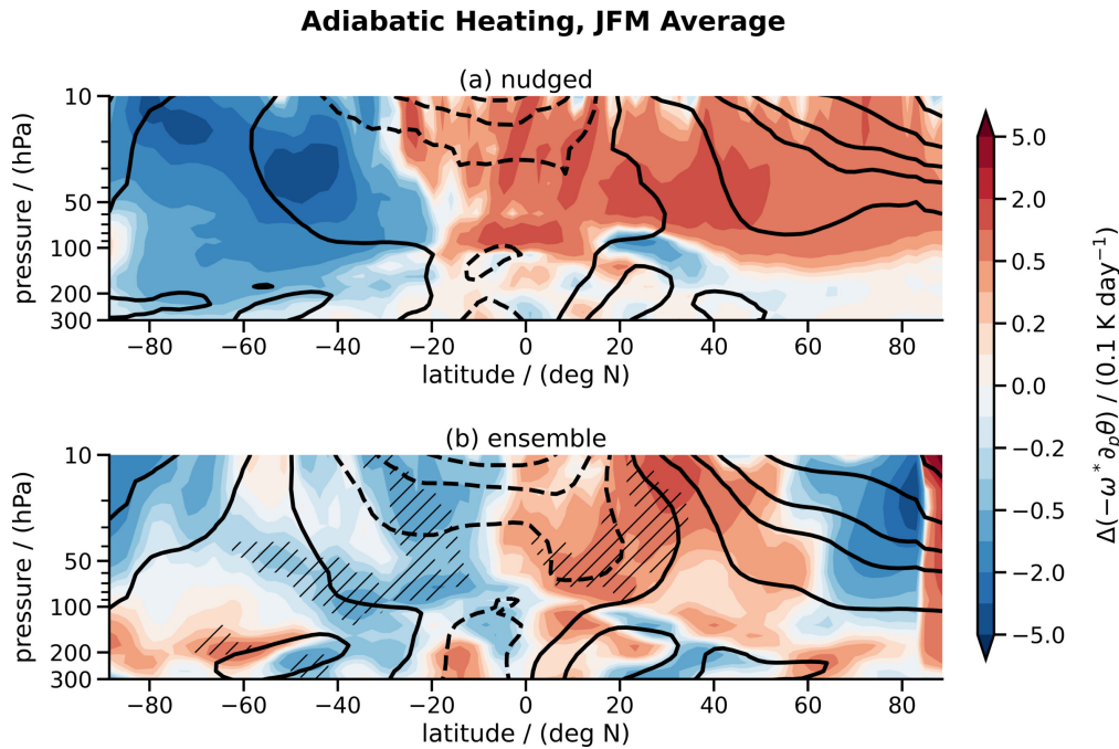
Figure 7. Similar to Fig. 6, but for the average perturbations in adiabatic heating due to circulation changes.
