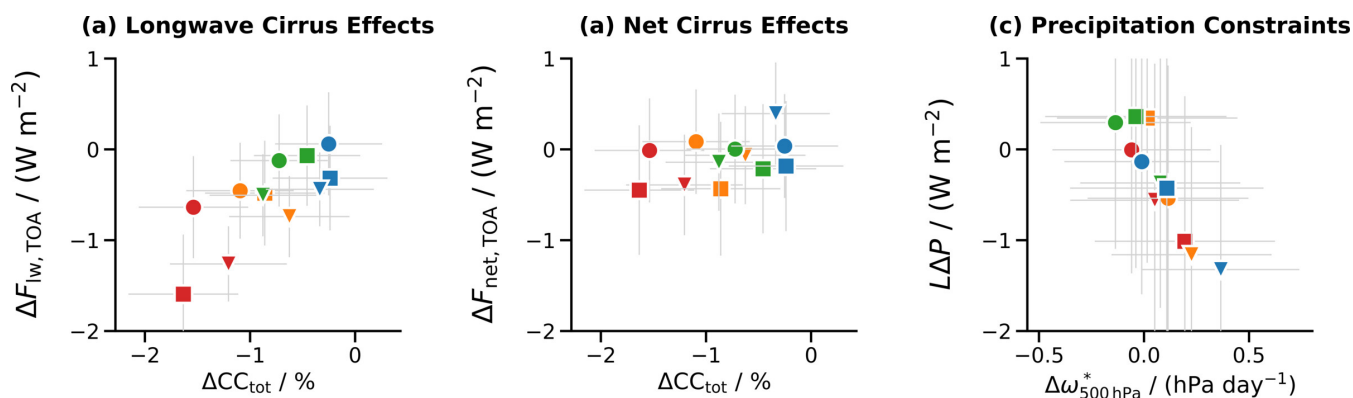
Figure 10. Cirrus effects on TOA radiation and energetic constraints for precipitation changes in the tropical belt set here to \varphi \in (20^\circ\text{S}, 20^\circ\text{N}) . Symbols and colors have the same meaning as in Fig. 8, which provides a legend to decipher the meaning of the symbols.
