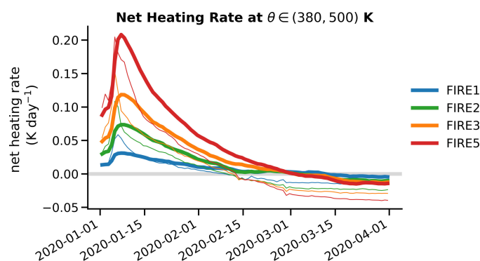
Figure 4. Net heating rate perturbation averaged globally for stratospheric altitudes between 380 < \theta < 500 K as function of time. Colors indicate the different fire strength perturbations similar to Fig. 2. Thick solid lines are ensemble mean values and thin solid line represent averaged nudged data. The light gray horizontal line marks the zero line for orientation.
