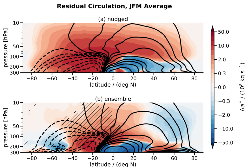
Figure 6. Average perturbations in residual circulation for (a) nudged simulations and (b) ensemble simulation as function of latitude and height. Contour lines indicate the state of the reference simulation FIRE0 with solid lines for positive values and dashed lines for negative values. Perturbations of the residual circulation in FIRE1 are presented in colored shading. Both, contours and shading have logarithmic spacing. Hatched regions have the same meaning as in Fig. 1.
