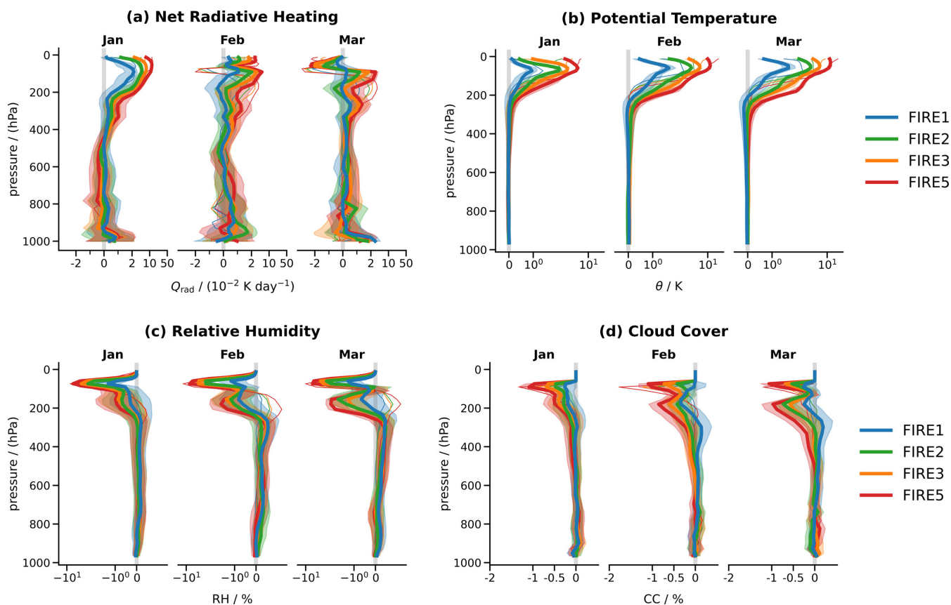
Figure 9. Globally-averaged vertical profiles of anomalies of (a) net radiative heating, (b) potential temperature, (c) relative humidity and (d) cloud cover as function of pressure. Similar to Fig. 4, thick colored lines represent ensemble mean perturbations with respect to the FIRE0 case. Temporal evolution from January 2020 (leftmost sub-panels) to March 2020 (rightmost sub-panels) is plotted. Humidity is shown relative to saturation over liquid water. Please note that the x-scale is non-linear to improve visibility.
