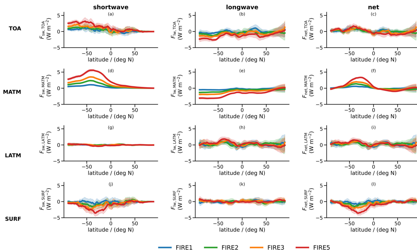
Figure 2. Ensemble and time zonal mean perturbations (JFM average) of radiative fluxes at TOA (1st row) and surface (4th row) and respective flux convergences between TOA and 200 hPa (2nd row), indicated as middle atmosphere (MATM) forcing, and between 200 hPa and surface (3rd row), indicated as lower atmosphere (LATM) forcing, as function of latitude. The colors represent deviations from the reference simulation (FIRE0) with different fire emission strength scaled by a factor of 1 (FIRE1: blue), 2 (FIRE2: green), 3 (FIRE3: orange) and 5 (FIRE5: red). The sum of shortwave (left column) and longwave (middle column) gives the net contribution (right column). Thick lines represent the ensemble mean value, whereas light shadings show the 95% confidence interval.
