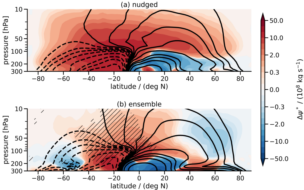
Figure 7. Average perturbations in residual circulation for (a) nudged simulations and (b) ensemble simulation as function of latitude and height. Contour lines indicate the state of the reference simulation FIRE0 with solid lines for positive values and dashed lines for negative values. Perturbations of the residual circulation in FIRE1 are presented in colored shading. Both, contours and shading have logarithmic spacing. Hatched regions have the same meaning as in Fig. 2.
