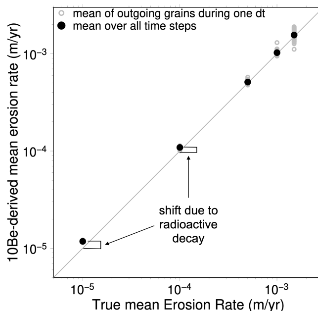
Figure 1. Comparison between the true (calculated from the landscape evolution model in Cidre) and ^{10}\text{Be} -derived erosion rates at dynamic equilibrium ( U = \bar{\epsilon} ) for different values of uplift rates (i.e. different simulations). The overestimation (shift) of the ^{10}\text{Be} -derived erosion rates for a low erosion rate ( 10^{-5} and 10^{-4} m/yr) comes from the absence of radioactive decay in Equation 14 used to infer the ^{10}\text{Be} -derived erosion rates whereas radioactive decay is taken into account in Cidre. Radioactive decay slightly decreases the mean ^{10}\text{Be} concentration calculated by Cidre, and thus the apparent inferred erosion rate neglecting radioactive decay, which is inversely proportional to the ^{10}\text{Be} concentration, is slightly overestimated.
