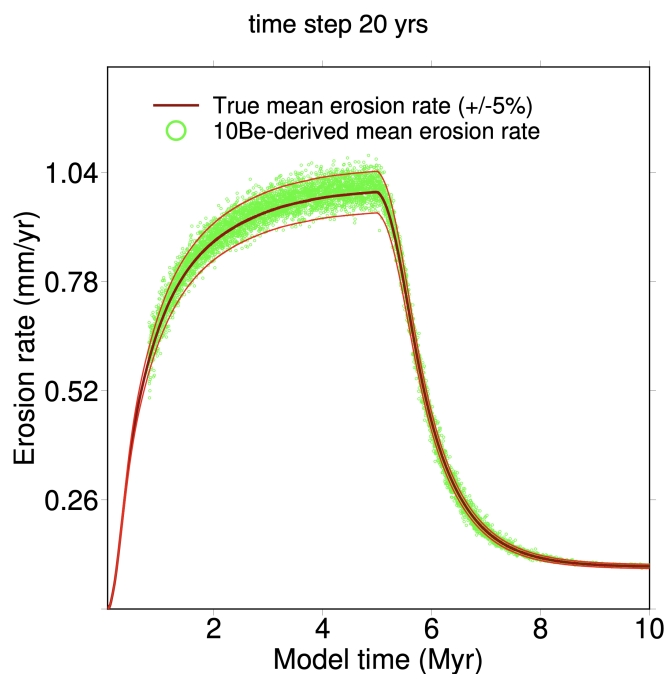
Figure 5. Effect of dividing the calculation time step by 10 on the mean ^{10}\text{Be} -derived erosion rate calculated from the mean ^{10}\text{Be} concentration of outgoing grains. The variability of the mean ^{10}\text{Be} -derived erosion rate increases because there is a smaller number of outgoing grains over a smaller time step.
