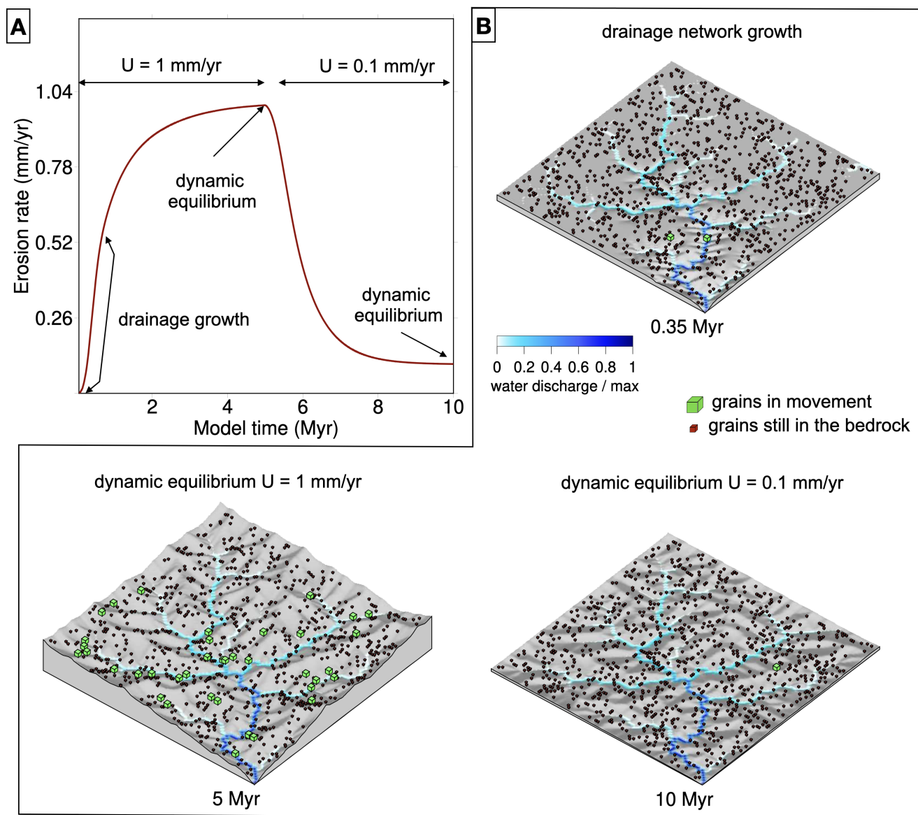
Figure 2. Reference simulation. A- Evolution of the mean erosion rate evolution with two periods of constant uplift rates. B- Snapshot of three stages in the topographic evolution. The number of displayed grains is divided by 10 for easier viewing.
