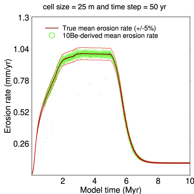
Figure 6. Effect of decreasing the cell size to 25 m (keeping the same number of cells) on the mean ^{10}\text{Be} -derived erosion rate calculated from the mean ^{10}\text{Be} concentration of outgoing grains. The different shape of the denudation curve compared to the reference simulation in Figure 3 comes from the increase in slopes in this simulation due to the smaller cell size, leading to a larger contribution of hillslope processes when the slope approaches the critical slope S_c in Equation 4.
