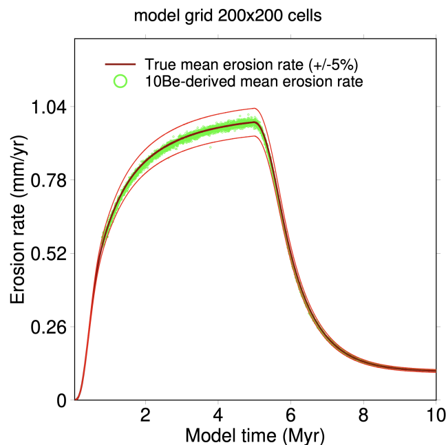
Figure 7. Effect of multiplying the model grid size by four on the mean ^{10}\text{Be} -derived erosion rate calculated from the mean ^{10}\text{Be} concentration of outgoing grains. The number of grains is also multiplied by four to have one grain per cell on average as in the reference simulation.
