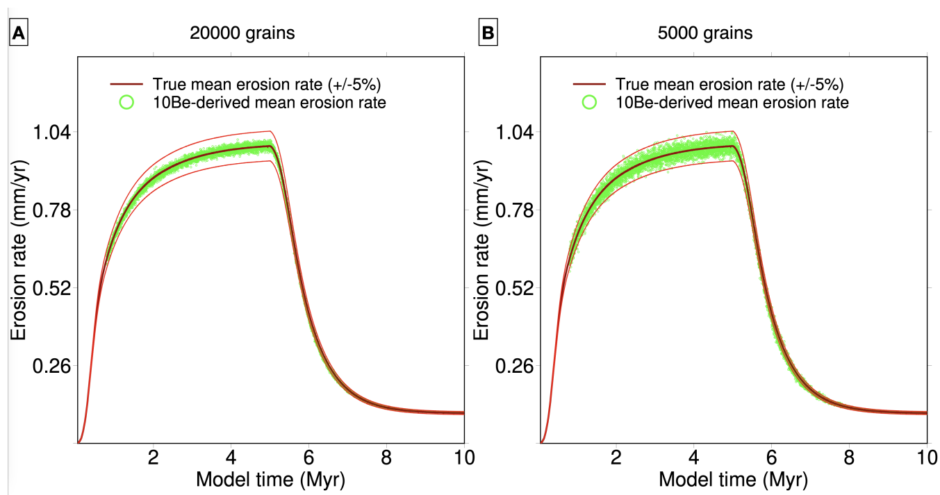
Figure 4. Effect of seeding the model with a different number of grains on the mean ^{10}\text{Be} -derived erosion rate calculated from the mean ^{10}\text{Be} concentration of outgoing grains. A- 20,000 grains (2 per cell in average). B- 5,000 grains (1 out of every 2 cells on average).
