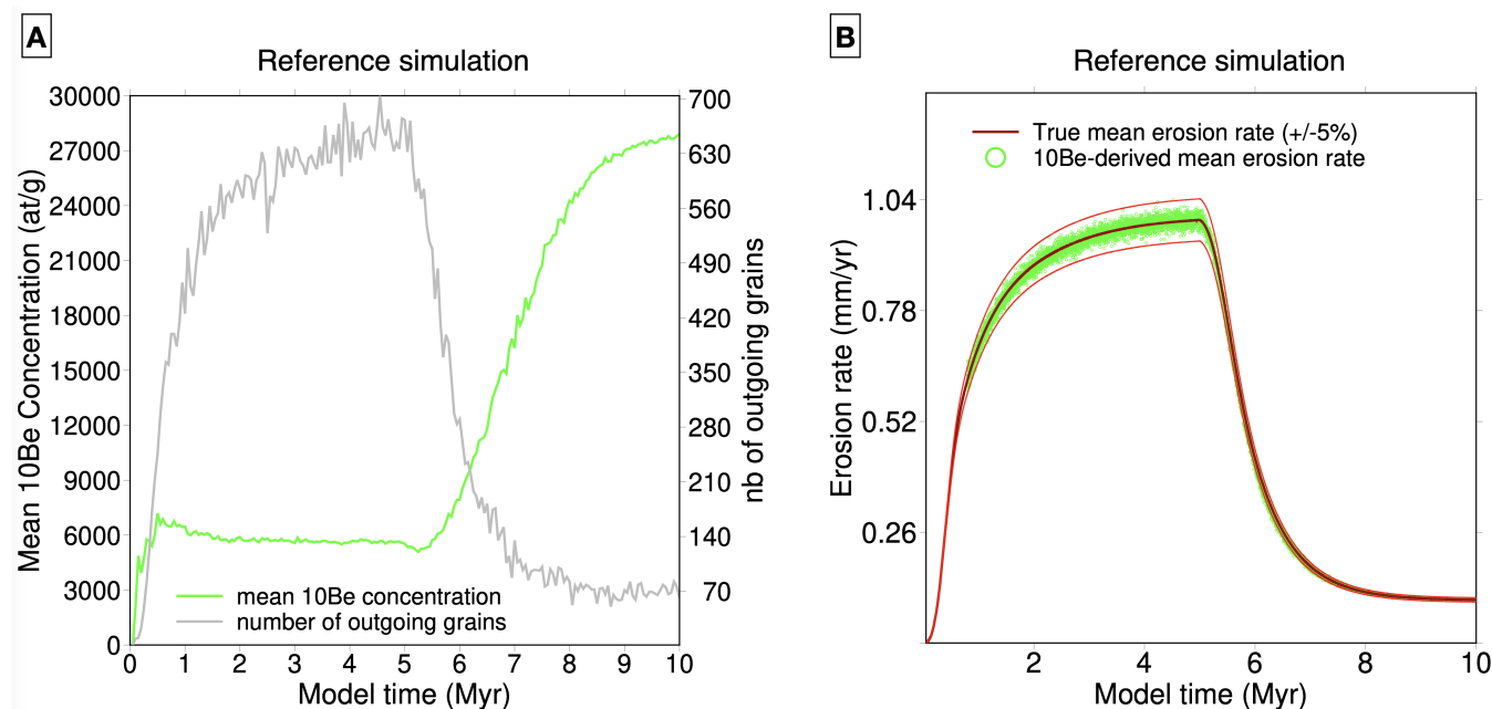
Figure 3. Reference simulation. A- Evolution of the number of outgoing grains during a time step (100 yrs) and the mean ^{10}\text{Be} concentration averaged over the outgoing grains. B- The true mean erosion rate calculated by Cidre and the mean ^{10}\text{Be} -derived erosion rate calculated from the mean ^{10}\text{Be} concentration of outgoing grains.
