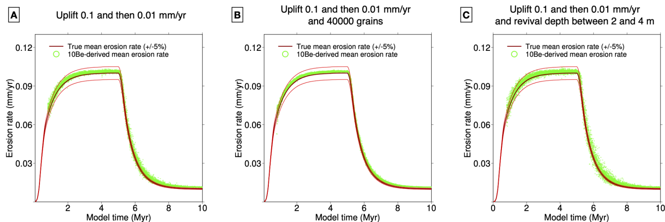
Figure 8. Effect of an uplift rate that is 10 times smaller. A- The number of grains is 10,000 as in the reference simulation. B- The number of grains is 40,000. C- The number of grains is 10,000 but the (revival) depth at which the grains are set back to the model grid is between 2 and 4 m instead of 1 and 2 m. In the three cases, the slight 1-2% overestimation of the ^{10}\text{Be} -derived erosion rate during the first dynamic equilibrium stage (4-5 Myr) comes from the model used to derive erosion rates that neglect the ^{10}\text{Be} radioactive decay, which only matters for low erosion rates. During the second period (6-8 Myr), there is a significant overestimation of the true erosion by approximately 20%. This overestimation comes mainly from the delayed response of the CN concentration for a low erosion rate. In C, the variability is larger because there are fewer grains going out at each model time step.
