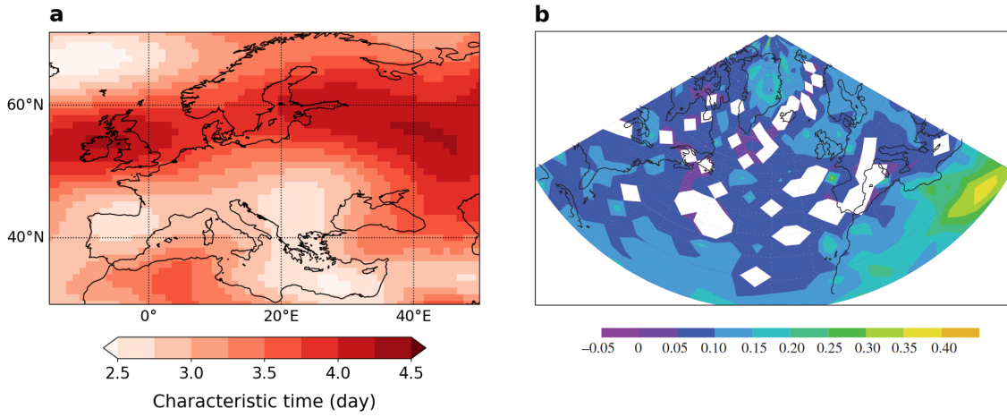
Figure 3. (a) Autocorrelation characteristic time ( T_p^C ; equation (4)) of JJA daily rescaled Z500. (b) Long-range dependence parameter d of unfiltered surface wind speeds. Only those values that are significant at the 5% level are displayed. Reproduced with permission from Franzke (2013).
