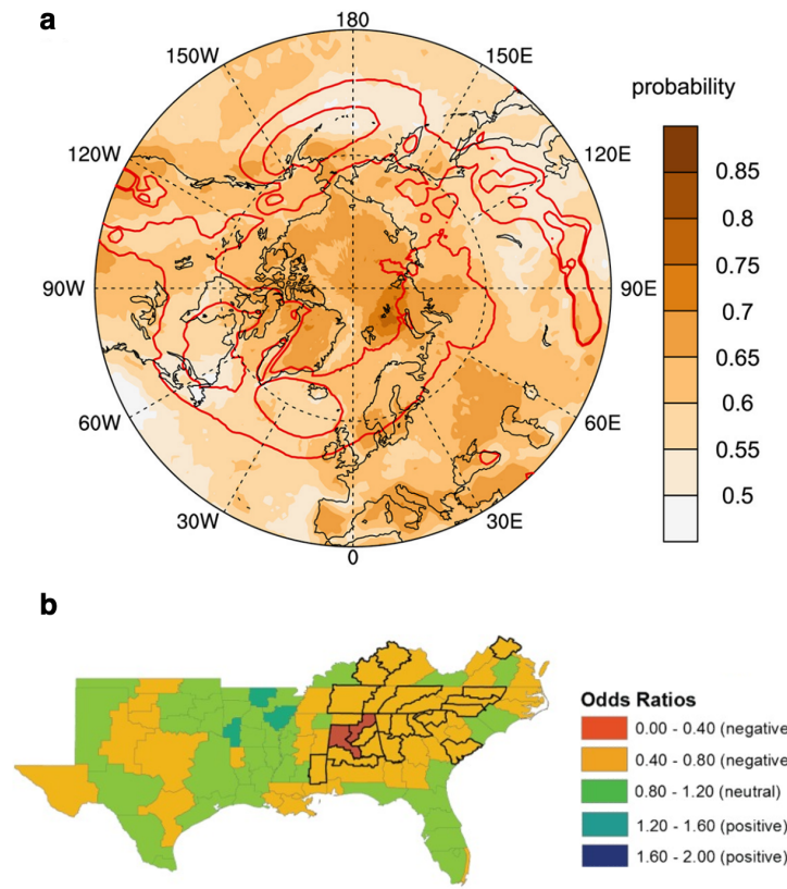
Figure 10. (a) Climatological May–October (MJJASO) hot spell survival probabilities (shaded) in ERA-Interim reanalysis data. Red contours show MJJASO cyclone frequencies of 30% and 40%, respectively. Reproduced with permission from Röthlisberger and Martius (2019). (b) Change in the odds ratio of drought occurrence in spring given a 1-unit increase in winter standardised precipitation index, estimated from logistic regression. Thick black contours indicate statistical significance with 95% confidence. Adapted with permission from Ford and Labosier (2014).
