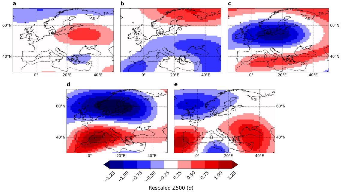
Figure 6. Five quasi-stationary states of JJA 5-day averaged rescaled Z500.
