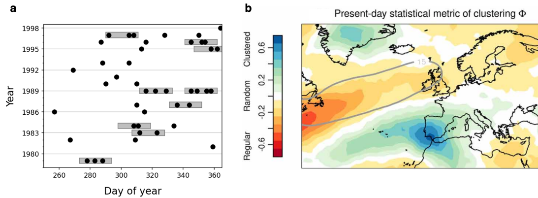
Figure 12. (a) Time-Example of a time series of extreme precipitation events (black dots) and 21-day periods containing more than 2 events (gray shading). Adapted from Kopp et al. (2021) under the terms of the Creative Commons Attribution 4.0 License. (b) Map of dispersion statistic \psi (equation (25)) of DJF cyclones over the 1975–2004 period, averaged across an ensemble of CMIP5 models. Reproduced from Bevacqua et al. (2020) under the terms of the Creative Commons Attribution 4.0 license.
