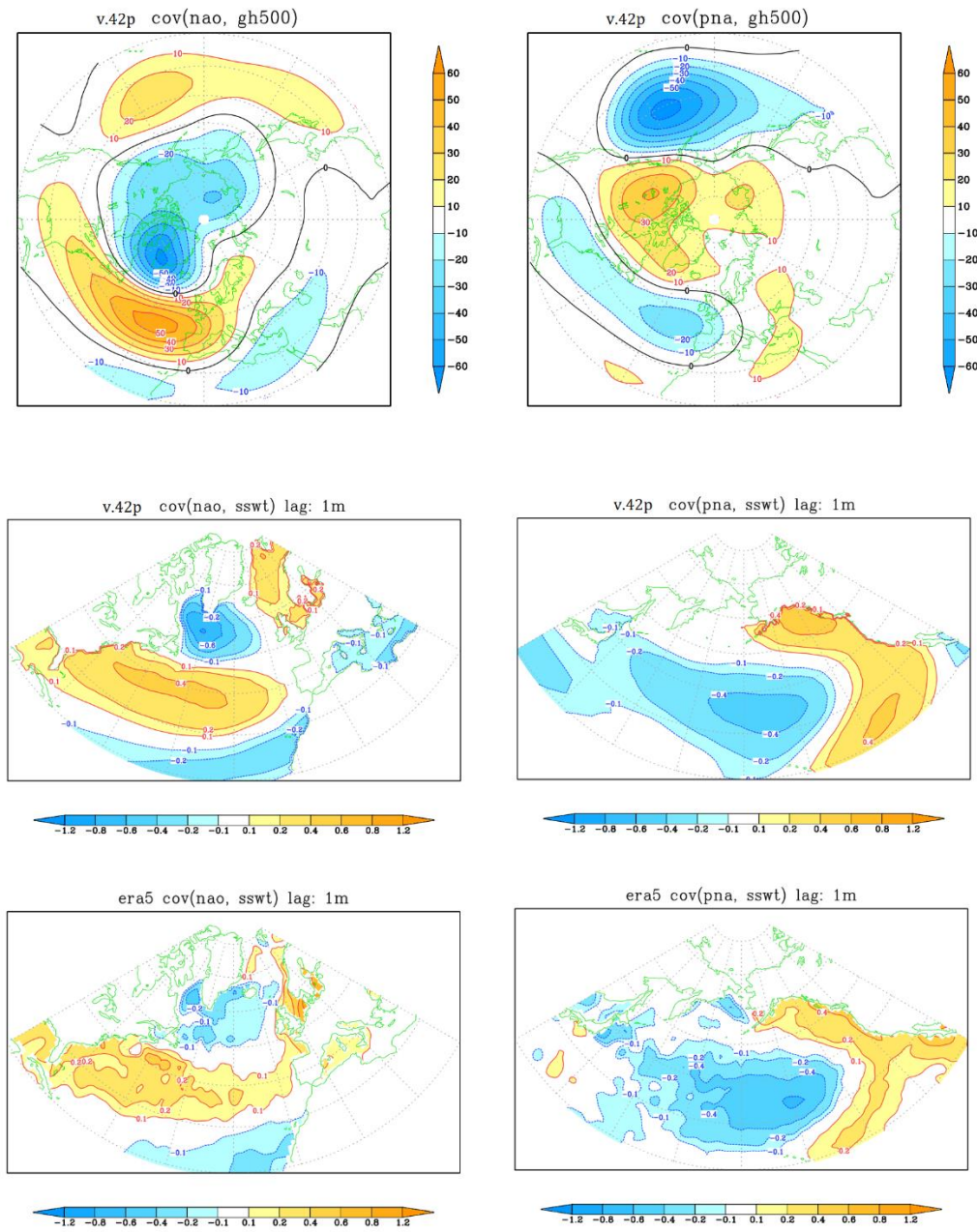
Figure 12: Covariances with the NAO (left) and PNA (right) indices in JF 1981-2020, as defined in Sect. 3.2. Top: covariance with 500-hPa height (in m) in the pacemaker ensemble (v.42p). Centre: 1-month-lag covariance with February-March SSWT (in °K). Bottom: as in central panels, but from ERA5 data.
