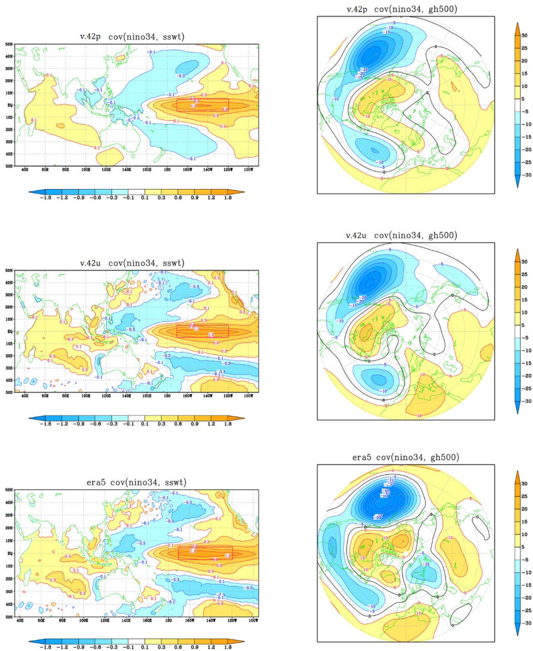
Figure 13: Covariances of SST (left, in °K) and 500-hPa height (right, in m) with the Nino3.4 SST index in JF 1981-2020. Top: from the pacemaker ensemble (v.42p). Centre: from the uncoupled ensemble with prescribed SST (v.42u). Bottom: from ERA5 data. SST covariances from the uncoupled ensemble and ERA5 are identical by definition.
