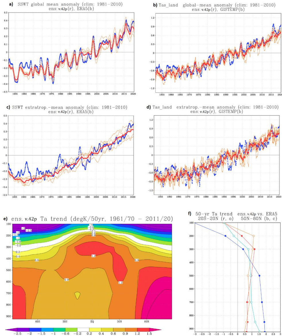
595 Figure 10: Top row: time series of global and annual-mean variability of a) surface sea-water temperature (SSWT), and b) SAT over land, from the SPEEDY-TOM3 pacemaker ensemble for 1951-2020 (v.42p). All data are anomalies from a 1981-2010 climatology, in °K. Red curve: ensemble mean; orange curves: individual ensemble members; blue curve: observational data from ERA5 (for SSWT) and GISTEMPv4 (for land SAT). Middle row: c) and d) as in a) and b) respectively, but only for the extratropical domain (25N-65N, 25S-65S) where no observational constraint is applied. Bottom row: linear trends of atmospheric temperature computed from overlapping 10-yr means, from 1961/70 to 2011/20. Units: °K/(50 yr). e): vertical cross section from the pacemaker ensemble (v.42p); f): vertical profiles of trends integrated in two latitudinal bands, from the ensemble in 20S-20N (red curve) and 50N-80N (blue curve), and from ERA5 in 20S-20N (orange curve) and 50N-80N (cyan curve). 600
