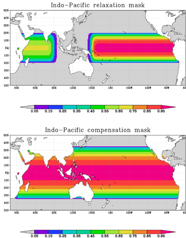
Figure 3: Relaxation mask (top) and compensation mask (bottom) used in the pacemaker experiments described in Sect. 4. See Sect. 2.2.4 305 for further details.
