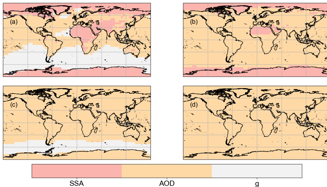
Figure 12: The largest contributor to the uncertainty in each of the three single scattering properties for four different cases: top-of-atmosphere (TOA) Direct Aerosol Radiative Forcing (DARE, panel (a)), TOA Direct Aerosol Radiative Effect (DARE, panel (b)), surface DARE (panel (c)) and surface DARE (panel (d)).
