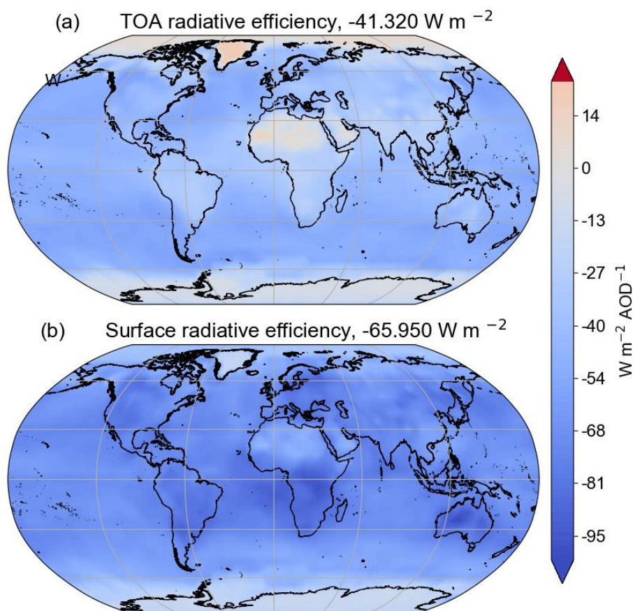
170 Figure 4: TOA (panel a) and surface (panel b) annual-mean Direct Aerosol Radiative Forcing (DARF) efficiency, in \text{W m}^{-2} per unit AOD, as derived from MACv2 and SOCRATES. Global mean values are shown above each panel.
