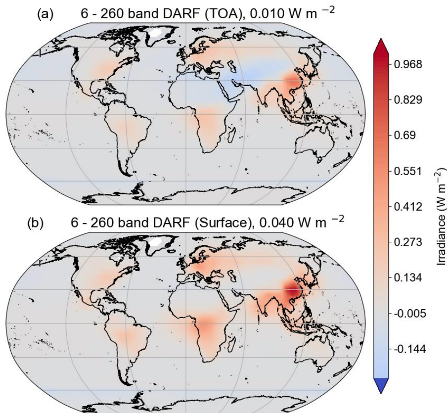
155 Figure 3: Differences in top-of-atmosphere (TOA, upper panel) and surface (lower panel) Direct Aerosol Radiative Forcing (DARF), in \text{W m}^{-2} , between radiative transfer calculations using a 260-band version of SOCRATES, with corresponding higher resolution aerosol optical properties, and the 6-band version used as reference in this work. The numbers in the panel labels are the globally averaged differences.
