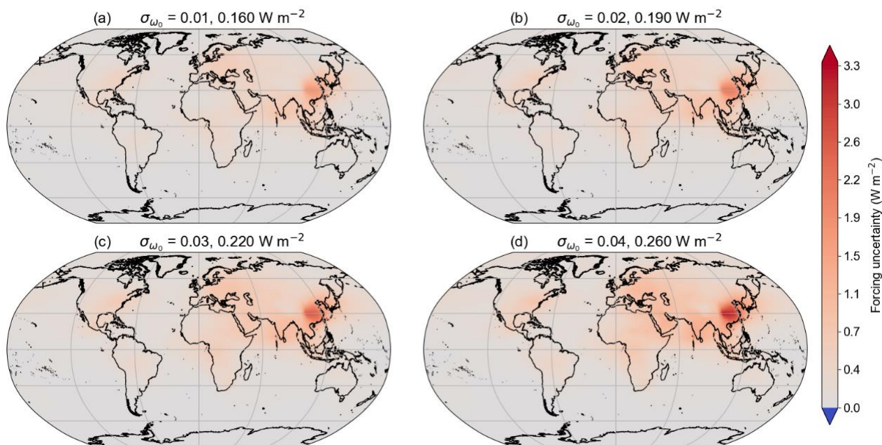
270 Figure 7: Example maps of uncertainty in top-of-atmosphere Direct Aerosol Radiative Forcing (DARF), calculated as the standard deviation in W m^{-2} , generated using 500 Monte Carlo samples for four combinations of optical property uncertainties. Each panel has the same uncertainty in aerosol optical depth and asymmetry factor of \sigma_{AOD} = 0.02 and \sigma_g = 0.03 , respectively, with increasing uncertainty in single-scattering albedo \sigma_{\omega_0} as indicated in the panel titles.
