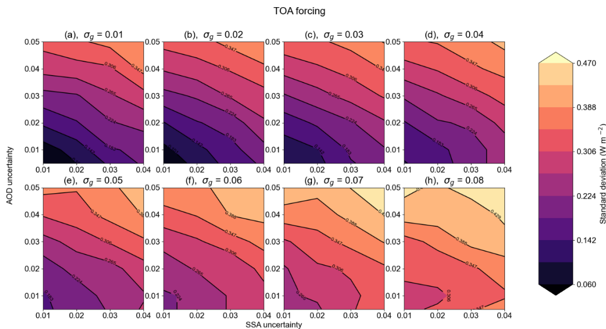
Figure 8: Contour of top-of-atmosphere (TOA) Direct Aerosol Radiative Forcing uncertainty, in W m^{-2} , with respect to SSA (x-axis) and AOD (y-axis) uncertainty. Each panel represents a change in asymmetry factor uncertainty of 0.01, within the 0.01 to 0.08 range.
