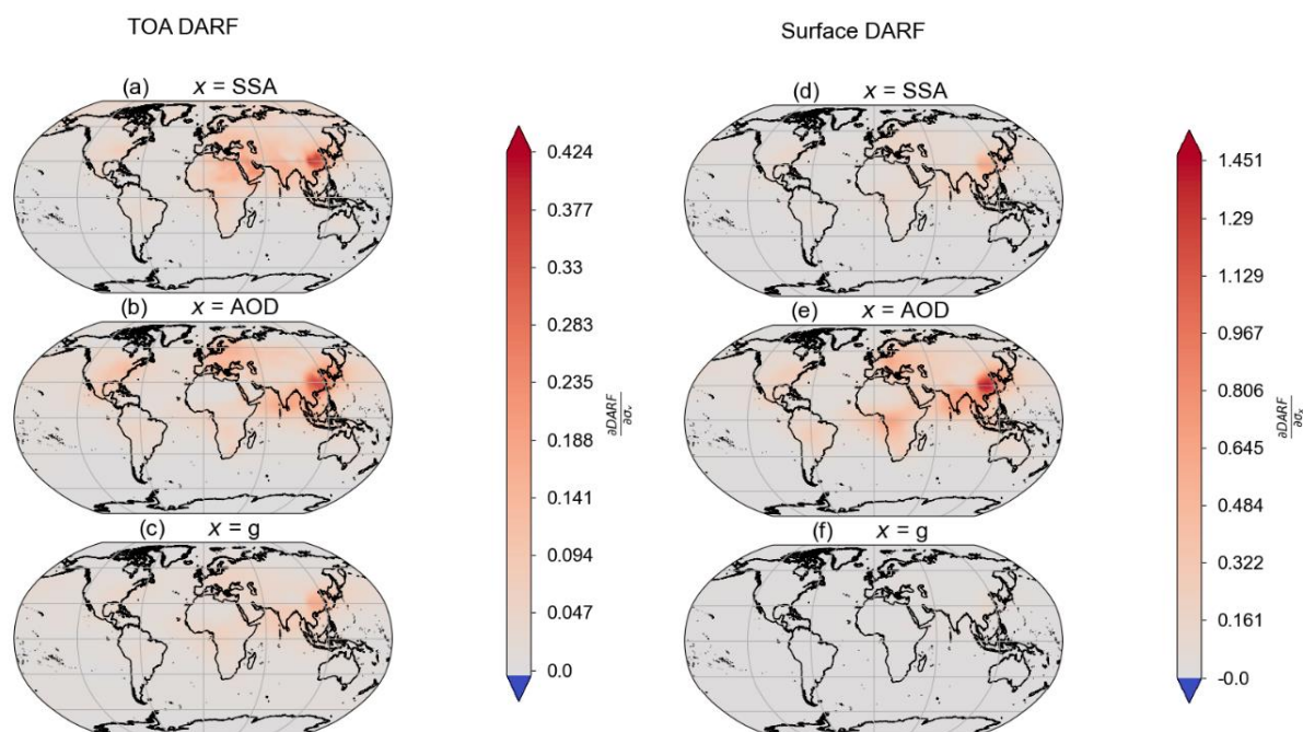
345 Figure 11: Same as Figure 10, but for Direct Aerosol Radiative Forcing (DARF).
