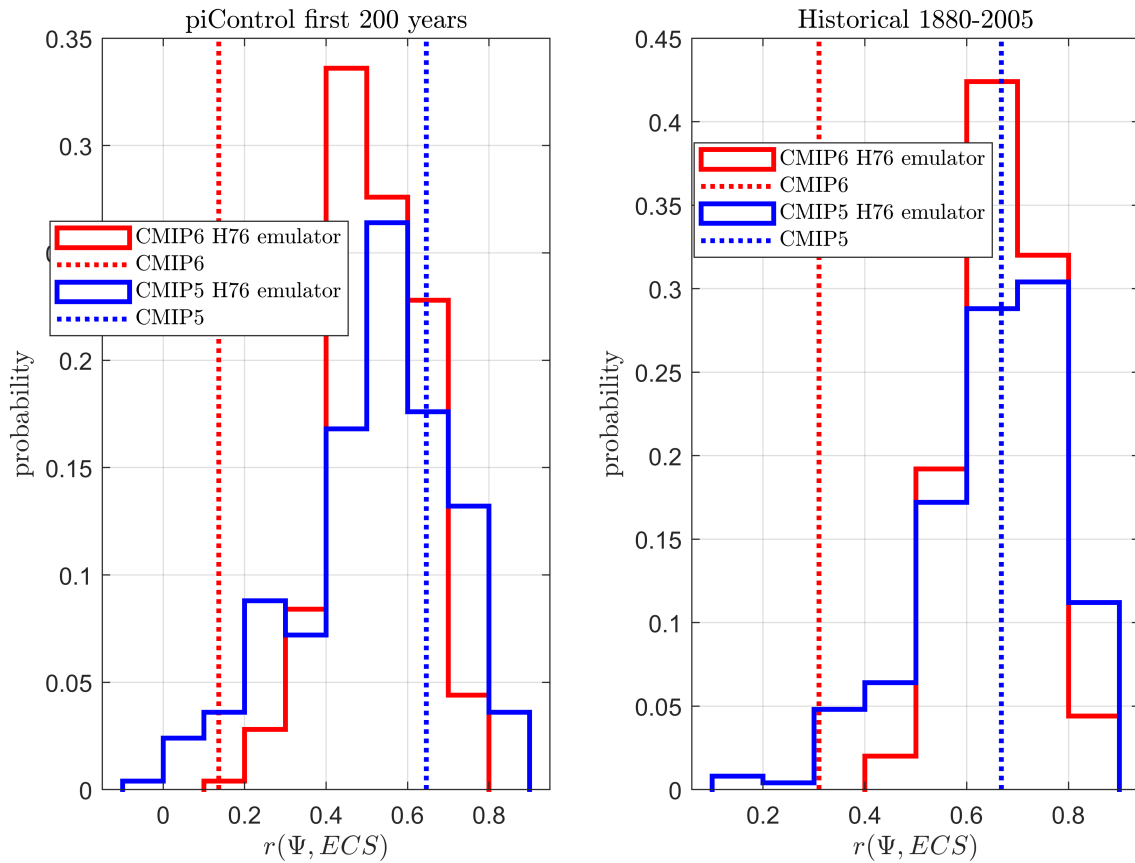
Figure 8. Probability of obtaining r(\Psi, ECS) in the H76 CMIP emulator ensembles performing a piControl (left panel) and historical (right panel) simulation if each two-box emulator is given the same value of \sigma_Q = 0.25 \text{ W m}^{-2} . The CMIP5 emulator ensemble histogram is given in blue, equivalent CMIP6 in red. The full complexity CMIP ensemble results performing the same experiment are the vertical dotted lines.
