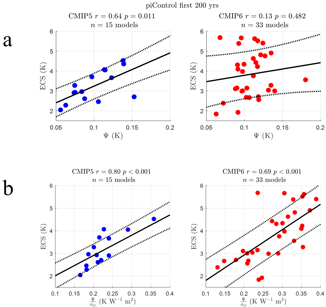
Figure 4. Individual models are plotted as circles (CMIP5 models are blue and CMIP6 models are red). The best fit line in the ordinary least squares sense is shown in black along with the standard deviation of the prediction error (black dotted line). Pearson correlation r and p value are given for each emergent relationship in each subplot title. The first 200 years of each model's timeseries is used to calculate \Psi and \sigma_Q running the piControl experiment (no external forcing). (a) \Psi against ECS in the CMIP5 (left panel) and CMIP6 (right panel) model ensembles. (b) \Psi/\sigma_Q against ECS in the CMIP5 (left panel) and CMIP6 (right panel) model ensembles.
