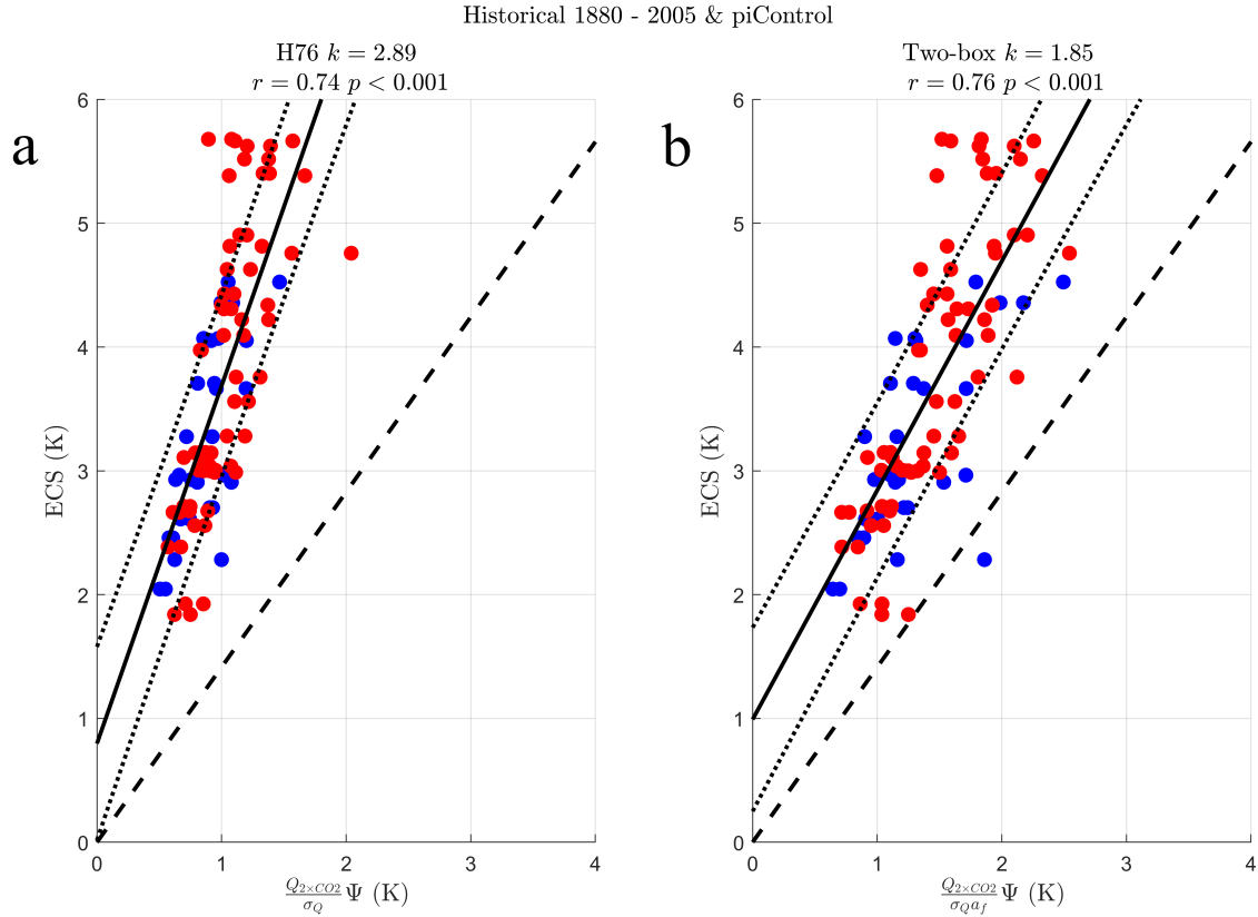
Figure 5. ECS against the theoretical predictor it is used proportional to calculate \Psi in (a) the one-box or H76 model and \sigma_Q (b) the two-box model. Individual models are plotted as circles (CMIP5 models are blue and CMIP6 models are red) running both historical and piControl experiments between 1880-2005 and the first 200 years of the simulation respectively. The best fit line in the ordinary least squares sense is shown in black along with the standard deviation of the prediction error (black dotted line). Pearson correlation r and p value are given for each emergent relationship in each subplot title. The empirically determined constant of proportionality between the x axis variable and ECS, k , is given in each subplot title. The H76 and two-box theoretical values of k = \sqrt{2} are plotted as the dashed black line.
