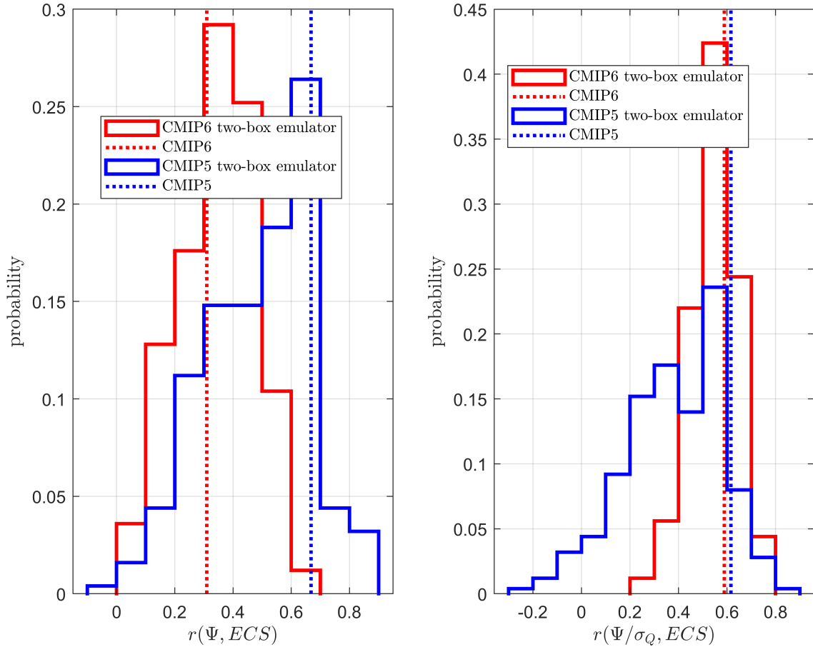
Figure A2. Probability of obtaining r(\Psi, ECS) (left) and r(\Psi/\sigma_Q, ECS) (right) in the two-box CMIP emulator ensembles performing a historical simulation of the period 1880-2005. The CMIP5 emulator ensemble histogram is given in blue, equivalent CMIP6 in red. The full complexity CMIP ensemble results performing the same experiment are the vertical dotted lines.
