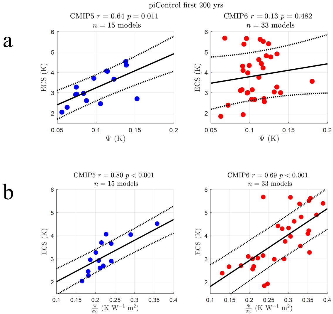
Figure 4. \Psi against ECS in the CMIP5 (left panel) and CMIP6 (right panel) model ensembles running the piControl experiment (no external forcing). The first 200 years of each model's timeseries is used to calculate \Psi . Individual models are plotted as circles (CMIP5 models are blue and CMIP6 models are red). The best fit line in the ordinary least squares sense is shown in black along with the standard deviation of the prediction error (black dotted line). Pearson correlation r and p value are given for each emergent relationship in each subplot title. \Psi/\sigma_Q . The first 200 years of each model's timeseries is used to calculate \Psi and \sigma_Q running the piControl experiment (no external forcing). (a) \Psi against ECS in the CMIP5 (left panel) and CMIP6 (right panel) model ensembles running. (b) \Psi/\sigma_Q against ECS in the piControl experiment CMIP5 (no external forcing left panel). The first 200 years of each and CMIP6 (right panel) model's timeseries ensembles.
