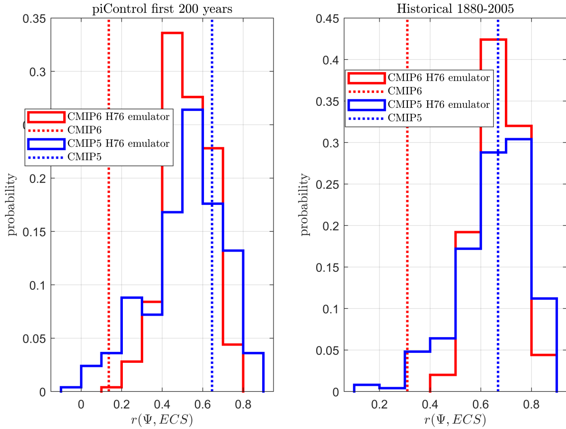
Figure 9. Probability of obtaining r(\Psi, ECS) in the H76 CMIP emulator ensembles performing a piControl (left panel) and historical (right panel) simulation if each two-box emulator is given the same value of \sigma_Q = 0.25 \text{ W m}^{-2} . The CMIP5 emulator ensemble histogram is given in blue, equivalent CMIP6 in red. The full complexity CMIP ensemble results performing the same experiment are the vertical dotted lines.
