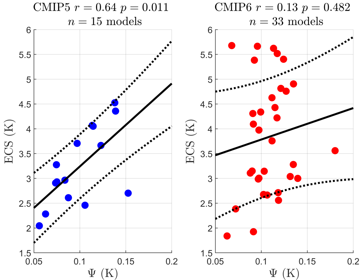
Figure 5. \Psi against ECS in the CMIP5 (left panel) and CMIP6 (right panel) model ensembles running the piControl experiment (no external forcing). The first 200 years of each model’s timeseries is used to calculate \Psi . Individual models are plotted as circles (CMIP5 models are blue and CMIP6 models are red). The best fit line in the ordinary least squares sense is shown in black along with the standard deviation of the prediction error (black dotted line). Pearson correlation r and p value are given for each emergent relationship in each subplot title.
