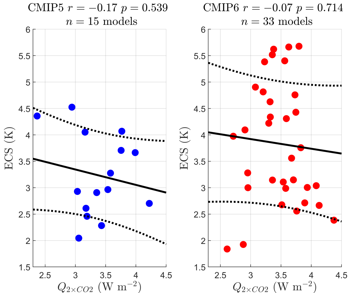
Figure 2. Q_{2 \times CO_2} against ECS in the CMIP5 (left panel) and CMIP6 (right panel) model ensembles. Q_{2 \times CO_2} is inferred from the abrupt4xCO2 experiment using the standard Gregory plot method. Individual models are plotted as circles (CMIP5 models are blue and CMIP6 models are red). The best fit line in the ordinary least squares sense is shown in black along with the standard deviation of the prediction error (black dotted line). Pearson correlation r and p value are given for each emergent relationship in each subplot title.
