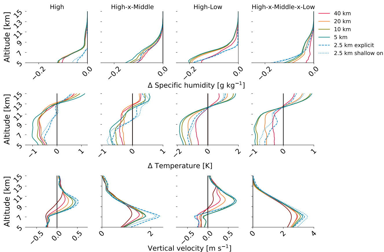
Figure 12. Simulations without convective parameterization exhibit stronger mean vertical velocities. Differences in the upper-tropospheric, time mean, area mean specific humidity (top row) and temperature profiles (middle row) from that of the 80-km simulation. Time mean, area mean vertical velocity profiles for all simulation settings (bottom row). Variables associated with the four cloud classes that include high clouds are shown for the simulations with the two-moment scheme only with all model settings as in Fig. 5.
