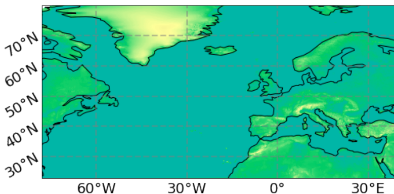
Figure 1. The NAWDEX simulation domain covers the entirety of the North Atlantic as well as the northeastern Canadian seaboard, Greenland, and Europe. The domain runs from 78°W to 40°E longitude and from 23°N to 80°N latitude.
