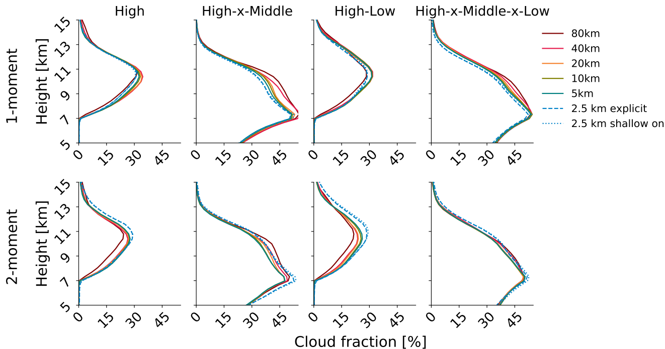
Figure S4. Cloud fraction does not change much with grid spacing across all classes with high clouds. Cloud fraction from one- (top panels) and two-moment (bottom panels) simulations for the four cloud classes that include high clouds with all model settings as in Fig. 5.
