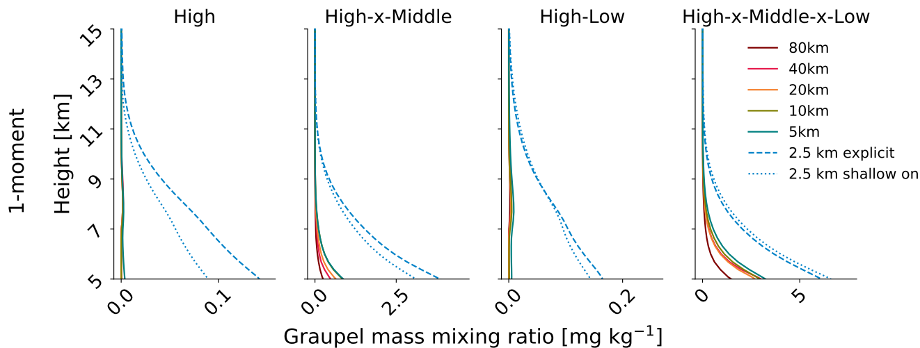
Figure S5. Grid spacing dependence for the one-moment microphysics simulations is concentrated in a radiatively inactive species. Graupel mass mixing ratios from the one-moment simulations for the four cloud classes that include high clouds with all model settings as in Fig. 5.
