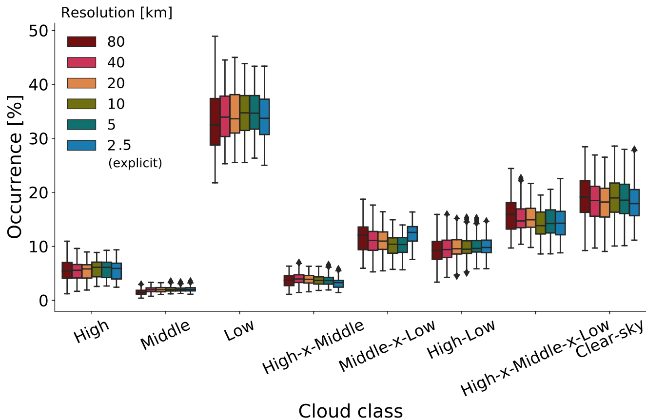
Figure S3. There are no systematic changes in cloud class occurrence with grid spacing. Area-weighted occurrence probability for eight cloud classes across grid spacings for the simulations with one-moment microphysics. The box shows 25th (Q1), 50th (Q2), and 75th (Q3) percentiles, while the whiskers show Q1-1.5(Q3-Q1) up to Q3+1.5(Q3-Q1) . Diamonds indicate outliers. Thresholds of 62%, 67%, and 30% are used for high, middle, and low clouds, but mean occurrence is not sensitive to these thresholds (Fig. S1). The 2.5-km simulation uses neither a deep nor shallow convective parameterization (explicit).
