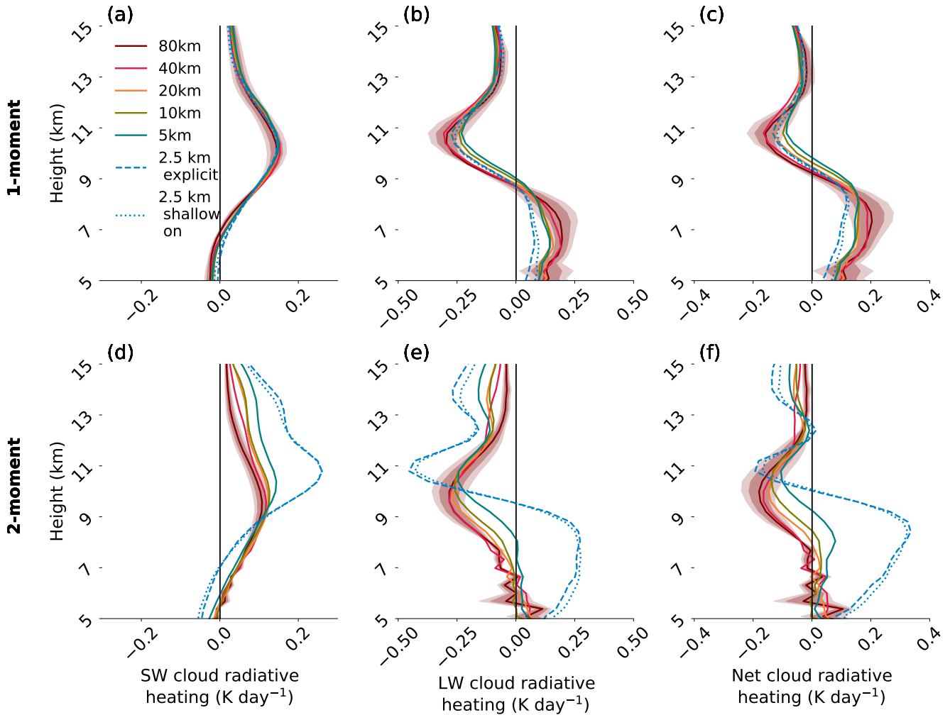
Figure S2. Dependency of net, shortwave, and longwave cloud-radiative heating on grid spacing, convective scheme, and microphysics is robust to simulation duration. Upper-tropospheric, time mean, area mean shortwave (left panels), longwave (middle panels), and net (right panels) cloud-radiative heating with all model settings as in Fig. 5. One- (top panels) and two-moment (bottom panels) microphysics scheme are shown. Note the different x-axis limits on each set of panels. The standard deviation and standard error over daily means are depicted as light and dark red shades atop the 80-km profile.
