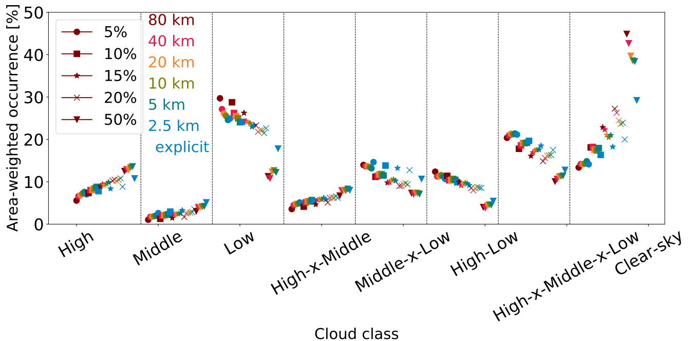
Figure S1. Occurrence probability is relatively insensitive to the cloud fraction threshold used to define various classes. Mean, area-weighted occurrence probabilities for eight cloud classes across grid spacings for the simulations with two-moment microphysics. Different symbols indicate different cloud fraction thresholds for Low, Middle, and High altitudinal ranges to qualify as cloudy. Different colors are grid spacings from 80 km down to 2.5 km, as in Fig. 7.
