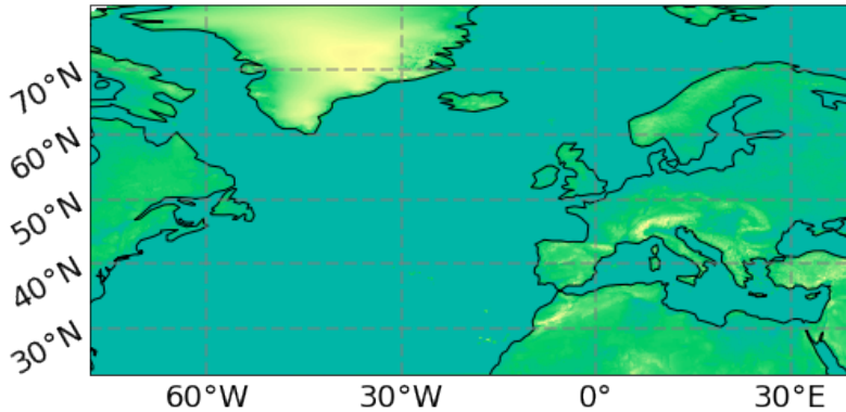
Figure 1. The NAWDEX simulation domain covers the entirety of the North Atlantic as well as the northeastern Canadian seaboard, Greenland, Northern Africa, and Europe. The domain runs from 78°W to 40°E longitude and from 23°N to 80°N latitude.
