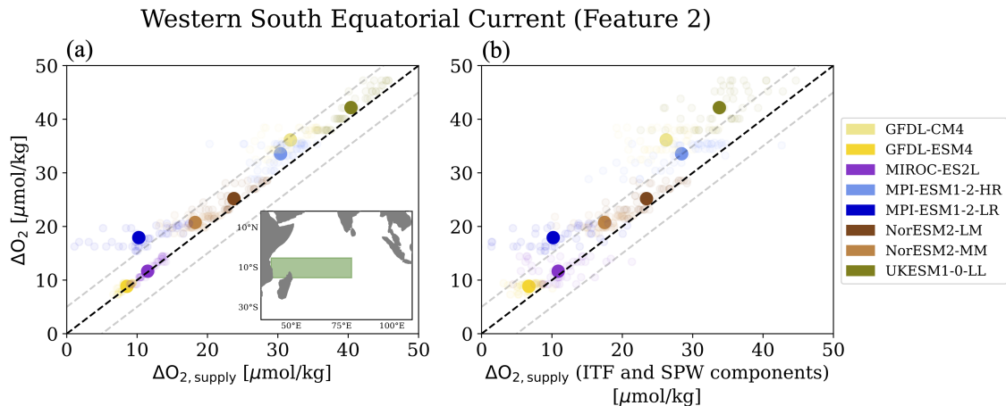
Figure 7. Dissolved oxygen changes computed from water mass composition changes, \Delta O_{2,supply} , versus total simulated dissolved oxygen changes in the western South Equatorial Current (indicated by inset in panel (a)). (a) \Delta O_{2,supply} from all source water changes. (b) \Delta O_{2,supply} only from contributions of Indonesian Throughflow and Southern Pathway Waters. Solid markers are mean of all samples (faded markers).
