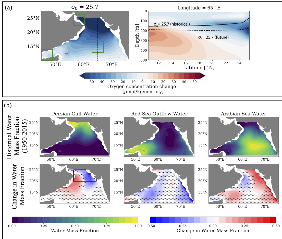
Figure 8. Multi-model mean (MMM) results of Optimum Multiparameter (OMP) analysis in the Arabian Sea. (a) Oxygen changes along the \sigma_0 = 25.7 surface and the historical (solid) and end-of-century (dashed) depth of \sigma_0 = 25.7 indicated over MMM oxygen changes in depth space at 65^\circ\text{E} . Green boxes mark source water regions. (b) Historical distribution of Persian Gulf, Red Sea Outflow, and Arabian Sea Water fractions, and changes in water mass fractions between historical and end-of-century states. Historical states calculated as 1950-2015 mean, and end-of-century states calculated as historical mean plus linear trends over 2015-2100. Solid black box in (b) show region of northern Arabian Sea over which we report changes. Stippling where less than 75% (6/8) of models agree on sign of change
