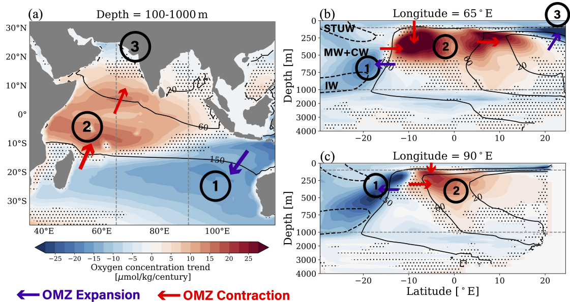
Figure 4. Multi-model mean (MMM) dissolved oxygen trends under SSP5-8.5 scenario forcing (2015-2100). Dissolved oxygen trends (a) between 100 and 1000m, (b) at 65°E and (c) at 90°E. Dashed gray lines mark (a) 65°E and 90°E, and (b,c) 100 and 1000m. Solid black contours represent 20, 60 and 150 \mu\text{mol/kg} oxygen. Dashed black contours highlight salinity signatures of Subtropical Underwater (STUW) and Intermediate Water (IW), with Central Water (CW) and Mode Water (MW) between. Main features of dissolved oxygen trends numbered, with effect on OMZ volume indicated by purple and red arrows. Results are stippled where less than 75 % (6/8) of models agree on sign of trend.
