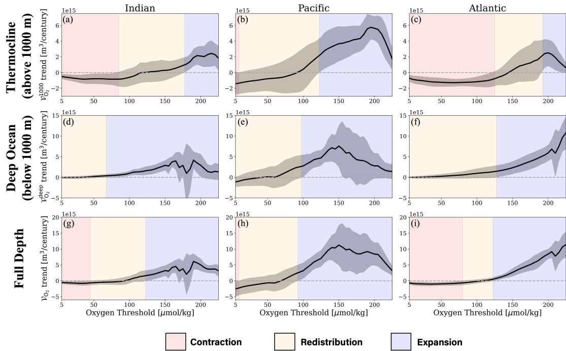
Figure 12. Multi-model mean thermocline OMZ volume trends (above 1000 m) under SSP5-8.5 scenario forcing (2015-2100) as a function of oxygen threshold for the tropical (30° S - 30° N) (a) Indian, (b) Pacific and (c) Atlantic Oceans. Deep ocean (below 1000 m) OMZ volume trends for the tropical (d) Indian, (e) Pacific and (f) Atlantic Oceans. Full depth OMZ volume trends for the tropical (g) Indian, (h) Pacific and (i) Atlantic Oceans. Shading represents one standard deviation of model spread from the mean. Panel a is the same as Fig. 3a
