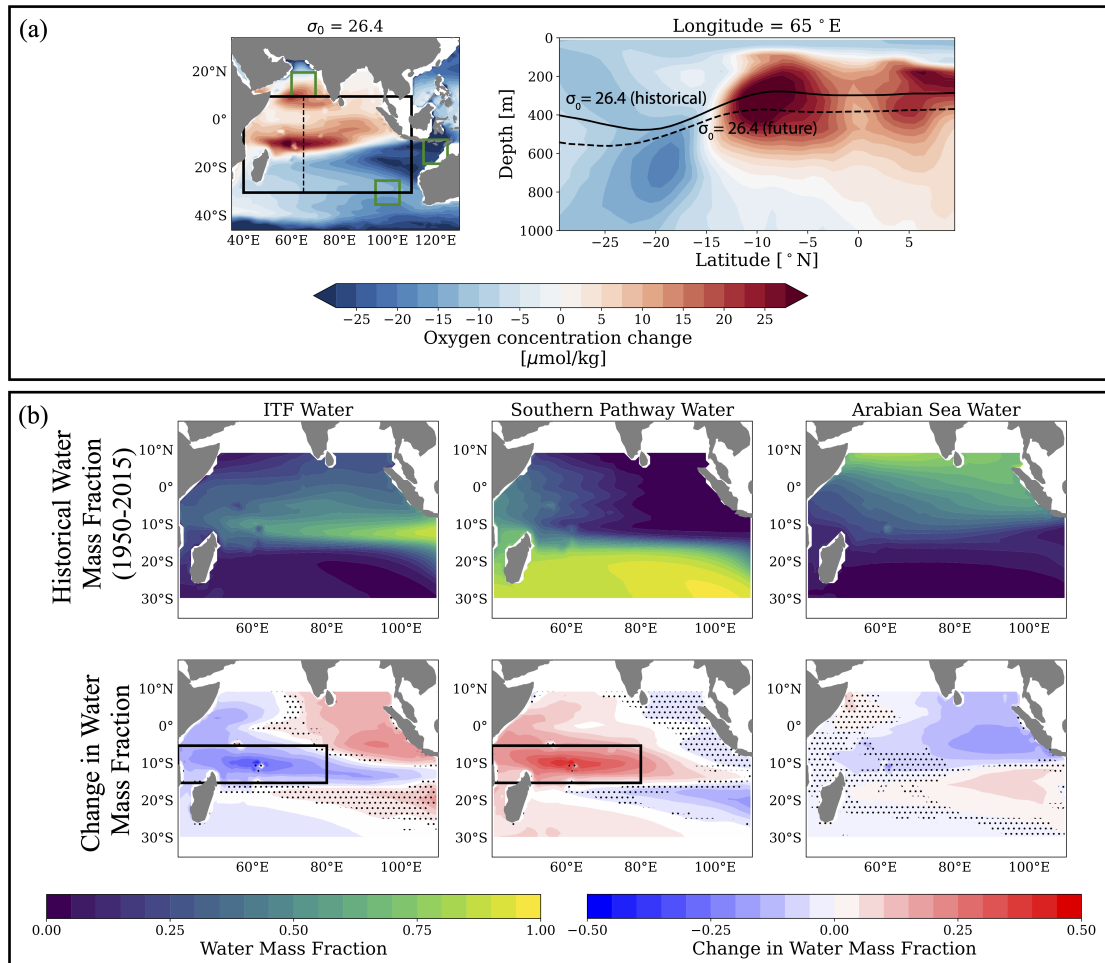
Figure 6. Multi-model mean (MMM) results of Optimum Multiparameter (OMP) analysis in the South Equatorial Current (SEC). (a) Oxygen changes along the \sigma_0 = 26.4 surface and the historical (solid) and end-of-century (dashed) depth of \sigma_0 = 26.4 indicated over MMM oxygen changes in depth space at 65^\circ\text{E} . Green boxes mark source water regions and solid black box represents region for which water mass fractions are solved. (b) Historical distribution of Indonesian Throughflow, Southern Pathway, and Arabian Sea Water fractions, and changes in water mass fractions between historical and end-of-century states. Historical states calculated as 1950-2015 mean, and end-of-century states calculated as historical mean plus linear trends over 2015-2100. Solid black boxes in (b) show region of western SEC. Stippling where less than 75% (6/8) of models agree on sign of change.
