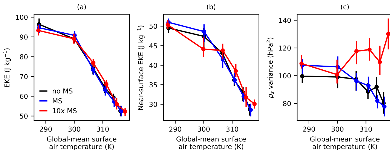
Figure 3. Vertically-integrated EKE (a), near-surface EKE (b), and surface pressure variance (c) averaged over midlatitude baroclinic zones and plotted as a function of global-mean surface air temperature. Vertical lines indicate 95% confidence intervals computing using block bootstrap resampling as described in the text. Horizontal lines indicating 95% confidence intervals for global-mean surface temperature are also included but are too small to be visible.
