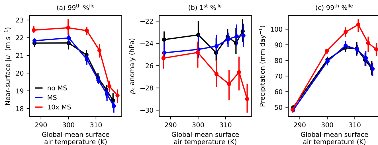
Figure 4. Extreme near-surface wind speeds (a), surface pressure anomalies (b), and precipitation (c) calculated over midlatitude baroclinic zones and plotted as a function of global-mean surface air temperature. 99th percentiles in panels a and c highlight particularly strong near-surface wind and precipitation; 1st percentiles shown in panel (b) highlight particularly strong surface lows. Vertical lines indicate 95% confidence intervals computed using block bootstrap resampling as described in the text. Horizontal lines indicating 95% confidence intervals for global-mean surface temperature are also included but are too small to be visible.
