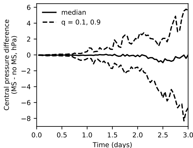
Figure 10. Transient evolution of pairwise differences in cyclone central pressure over the first 3 days of TC world restart experiments. The median and q = 0.1 and = 0.9 quantiles are calculated over the entire population of cyclones, and corresponding cyclones in experiments with and without the mass sink are matched as described in the text.
