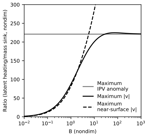
Figure 7. Ratios of maximum IPV anomalies (gray), azimuthal wind speeds (solid black), and near-surface azimuthal wind speeds (dashed black) produced by latent heating and the mass sink in inversions with varying Burger number B = L_D^2/L^2 .
