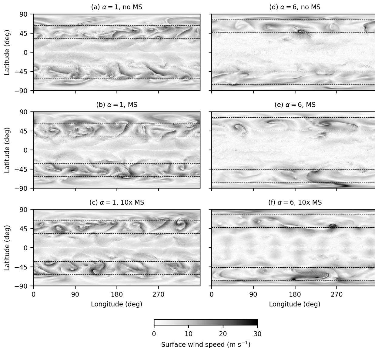
Figure 2. Wind speed in the lowest model level from the last saved snapshot of simulations in the control climate with \alpha = 1 (a,b,c) and the warmest climate with \alpha = 6 (d,e,f) with no mass sinks (a,d), realistic mass sinks (b,e), and mass sinks exaggerated by a factor of 10 (c,f). Midlatitude baroclinic zones defined based on the meridional eddy potential temperature flux are delimited by dashed lines.
