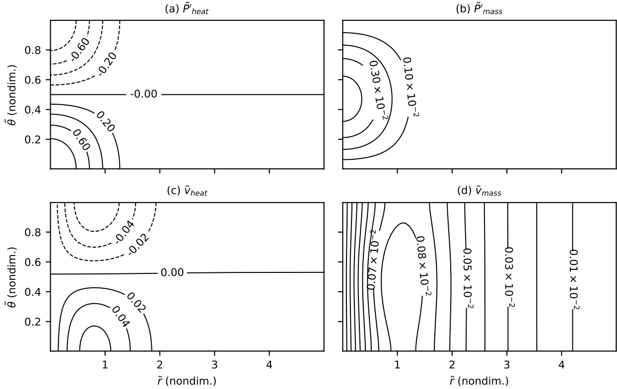
Figure 6. Short-time IPV anomalies produced by latent heating (a) and mass sinks (b), and azimuthal velocity fields induced by latent heating (c) and mass sinks (d) from a linearized inversion with B = 1 .
