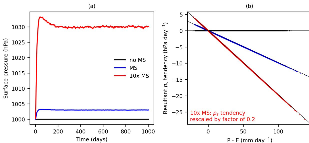
Figure A1. Time series of global-mean surface pressure (a) and relationship between precipitation minus evaporation ( P - E ) and the component of the surface pressure tendency from the mass sink (b) in T42 simulations at \alpha = 1 . Points in panel (b) are for different grid boxes and instantaneous times at all latitudes, and diagonal lines in panel (b) show the expected relationship based on hydrostatic balance (see text). Surface pressure tendencies for the 10x-MS simulation are rescaled by a factor of 0.2 in panel (b) to make surface pressure tendencies for MS and no-MS simulations more easily visible.
