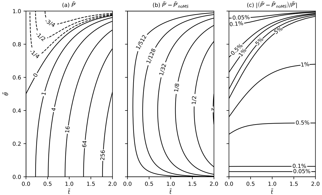
Figure 5. Evolution of IPV in a precipitating column and the contribution from the precipitation mass sink. Panel (a) shows the IPV anomaly \tilde{P}' that develops in response to latent heating, mass sinks, and vertical advection. Panel (b) shows the difference between \tilde{P}' and the IPV anomaly \tilde{P}'_{noMS} that develops with only latent heating and vertical advection included. This difference quantifies the influence of the mass sink on \tilde{P}'_{both} . Panel (c) shows the magnitude of the relative difference between IPV anomalies that develop with and without the mass sink.
