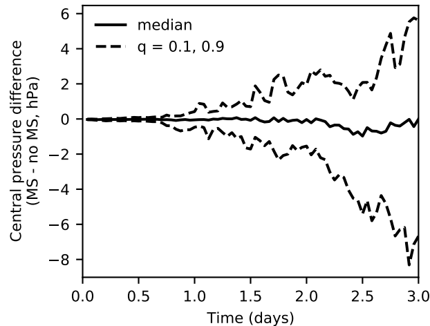
Figure 11. Transient evolution of pairwise differences in cyclone central pressure over the first 3 days of TC world restart experiments. The median and q = 0.1 and = 0.9 quantiles are calculated over the entire population of cyclones, and corresponding cyclones in experiments with and without the mass sink are matched as described in the text.
