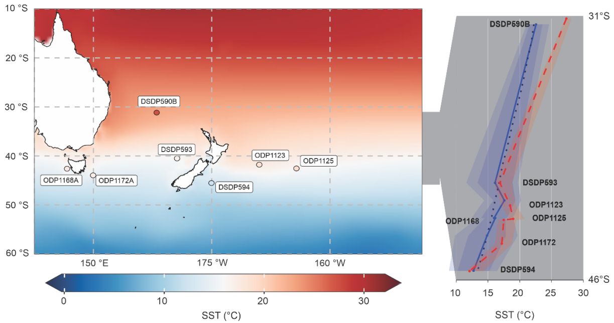
Figure 5: Ensemble mean regional Sea Surface Temperature (SST) from core PlioMIP experiments with mid-Pliocene Warm Period (mPWP) site mean interglacial SST plotted using the same temperature scale. a) absolute SST between 31–46°S for PlioMIP latitudinal mean (blue dotted), PlioMIP site specific (blue solid) with transparent blue shading for minima-maxima and heavier blue shading for \pm 1 standard deviation of the PlioMIP ensemble and mPWP site specific (red dashed) with mean-maxima shaded in red.
