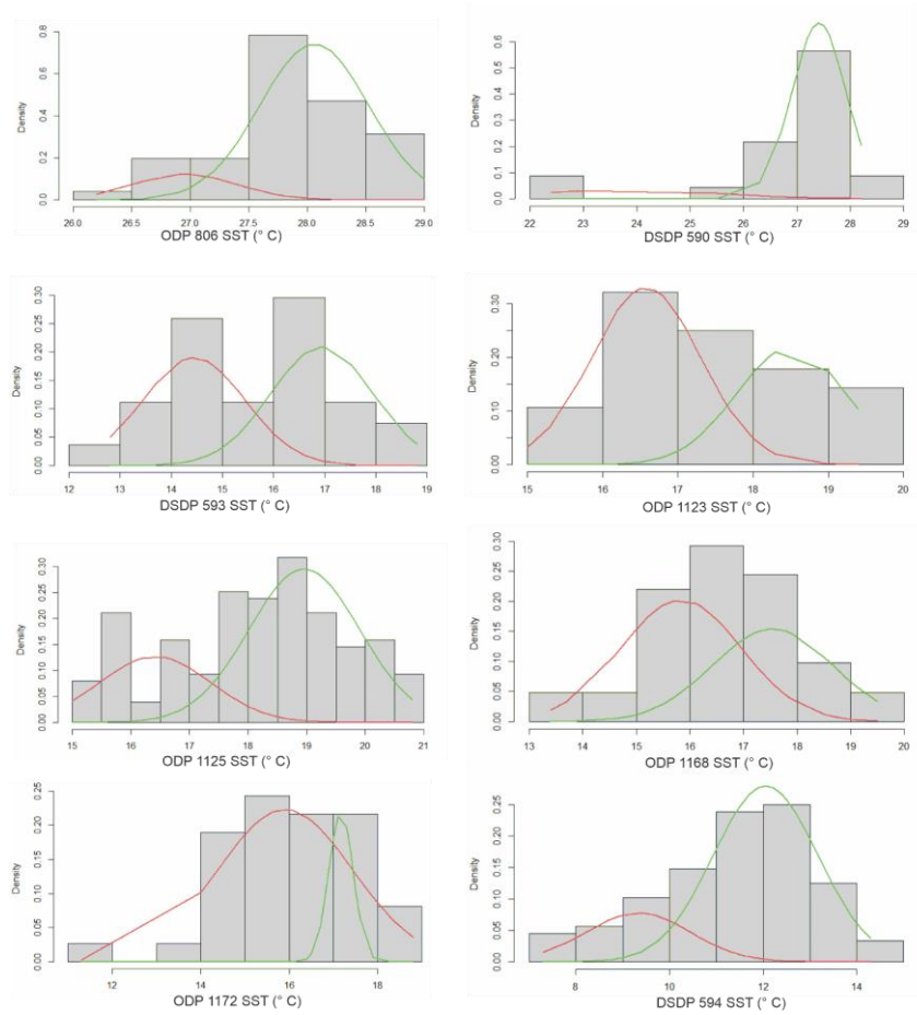
735 Figure B1. Bimodal analysis for each site after Benaglia et al. , (2010), excluding ANDRILL as it only represents interglacial conditions, displaying density curves with calculated bimodal distributions interpreted as glacial distributions (red) and interglacial (green). Code is available.
