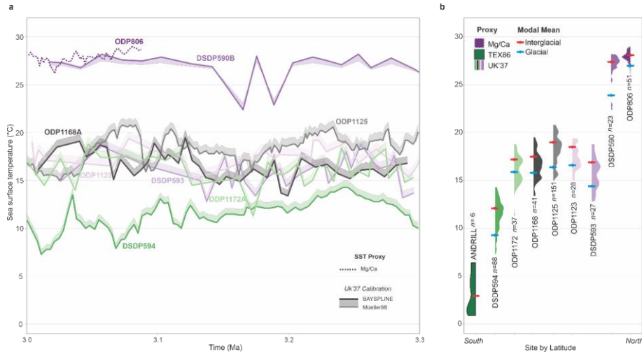
380 Figure 4: Time series and SST distribution for mid-Pliocene Warm Period (3.3 – 3.0 Ma) records. a) U_{37}^{K'} -SST calibrations of BAYSPLINE (solid; Tierney and Tingley, 2018) with the difference to Müller et al. (1998) shaded are plotted for all timeseries, with ODP 806 (Mg/Ca SST derived) and excluding ANDRILL (not plotted due to poor age control). b) Probability distributions ('violin plots') of the SST timeseries. Interglacial (red) and glacial (blue) modal means are also shown (Table 2; Fig. B1). Data for this plot are provided in Table S1 and Table S2.
