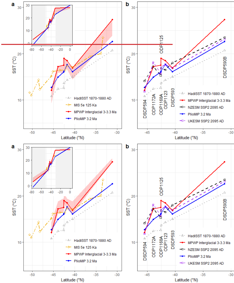
Figure 7: Absolute Sea Surface Temperatures as a latitudinal transect of the Southwest Pacific with a) HadISST (NCAR, 2022), mid-Pliocene Warm Period interglacial (solid red with the red ribbon showing mean to maximum SSTs), PlioMIP multi-model mean (solid blue) and Marine Isotope Stage (MIS) 5e (~125 ka) (dashed yellow; Cortese et al. , 2013), and b) HadISST (dotted grey; NCAR, 2022), mid-Pliocene Warm Period interglacial modal mean (solid red), NZESM (dashed black) and UKESM (dashed purple) for SSP2-4.5 2090–2099 AD (Williams et al. , 2016; Sellar et al. , 2019).
