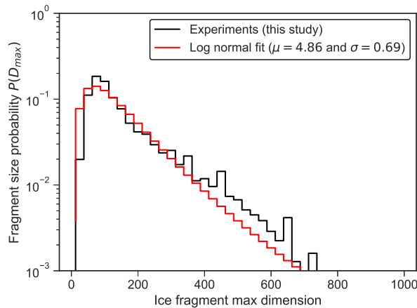
Figure 13. Parameterization for fragment size distribution from our collision experiments. Integrated log-normal probability density function in red and initial data from experiments in black.
