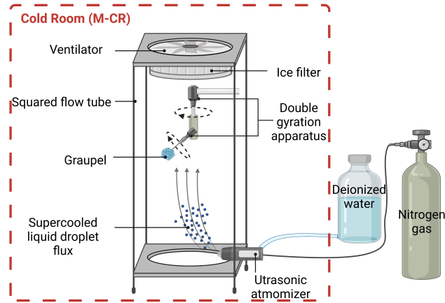
Figure 1. The apparatus GEORG used for the generation of nature-like lump graupel (Theis et al., 2022, modified after). The flow tube was placed inside the M-CR at -15 \text{ }^\circ\text{C} , while the gas and water bottles were kept outside the cold room.
