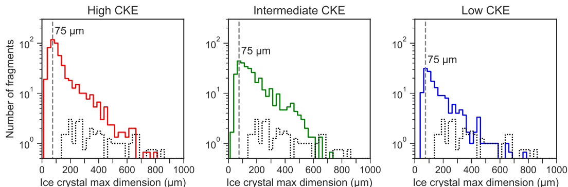
Figure 12. Average fragment size distributions as solid line for different CKE ranges of graupel-graupel with dendrites collisions at high supersaturation ( S_{ice} \approx 23\% ) : blue: low; green: intermediate; and red: high CKE. Average size distribution of crystals on graupel surface as black dotted line.
