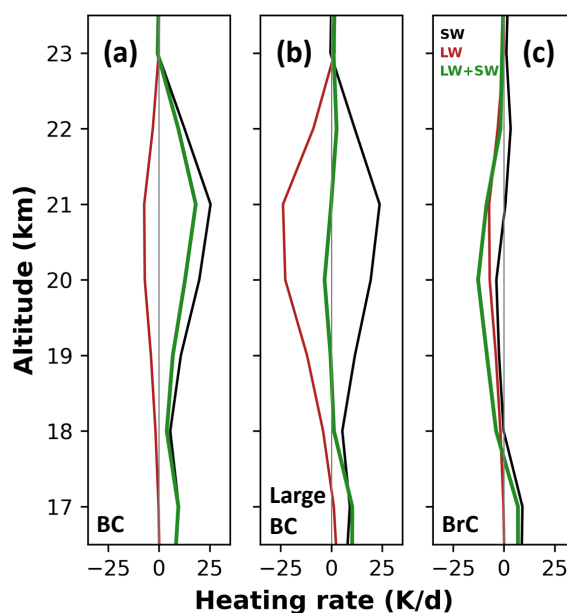
325 Figure 6: In-vortex SW, LW and net SW+LW HR for the CALIOP overpass of the main vortex on 11 January 2020 (CALIOP overpass shown in Fig. 3), with 3 assumed scenarios for the unmeasured aerosol properties: Black carbon (BC, SW SSA: 0.80, SW g: 0.5-0.7, LW SSA: 0.20, LW g: 0.3, panel a), Large black carbon (Large BC, SW SSA: 0.80, SW g: 0.7, LW SSA: 0.20, LW g: 0.5, panel b) and Brown carbon (BrC, SW SSA: 0.90-0.95, SW g: 0.7, LW SSA: 0.20, LW g: 0.5, panel c). These 3 cases are defined in a consistent manner as in S22.
