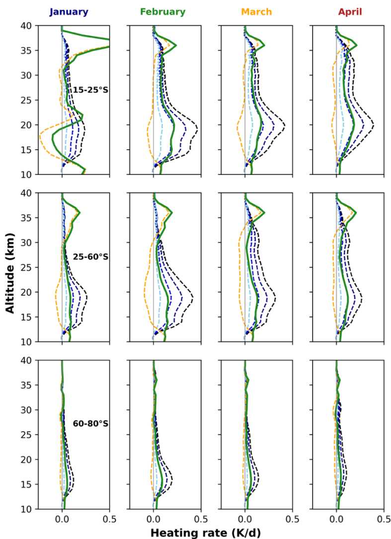
290 Figure 4: Monthly mean regional equinox-equivalent daily-average), SW (shades of blue and black lines), LW (orange lines) and net SW+LW (green lines) HR, from January to April 2020 (different columns), in three latitude ranges (15-25, 25-60 and 60-80°S, upper to bottom lines). Following the Mie calculations discussed in the text, different assumptions are made for SSA and g. SSA (SW component): sky blue lines: 0.95, medium blue lines: 0.90, dark blue lines: 0.85, black lines: 0.80. SSA (LW component): orange lines: 0.20. G (LW component): dashed lines: 0.5, dotted lines: 0.3. G (SW component): dashed lines: 0.7, dotted lines: 0.5.
