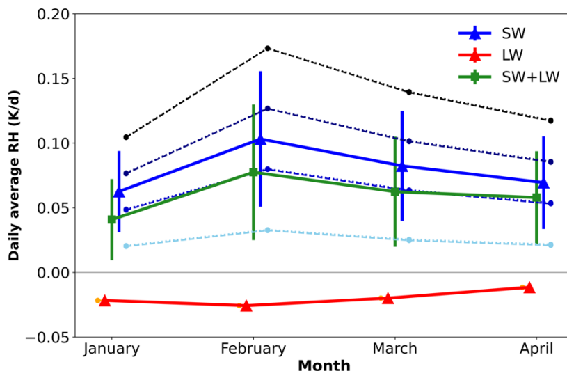
Figure 5: Time series, from January to April 2020, of the monthly mean area-weighted Southern-Hemispheric HR, based on equinox-equivalent daily-average HR of Fig. 4), for the UTLS perturbation of Australian fires in 2019–2020. The radiative heating profiles are averaged in the altitude range 12–25 km. Different shades/types of blue dots and lines are for different SSA and g values – the darker the shade the smaller the SSA, dashed/dotted lines for larger and smaller g, see caption of Fig. 4 for details.
