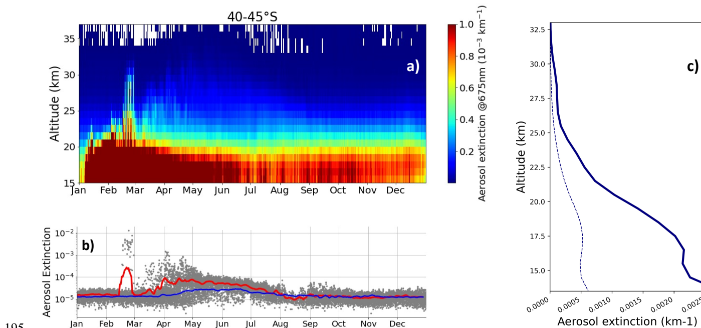
Figure 2: OMPS-LP observations at 675 nm in the latitude interval 40\text{-}45^\circ\text{S} : time series of the zonal average vertical profiles of the aerosol extinction in 2020 (panel a), individual aerosol extinction coefficient observations at 28 km altitude (panel b), monthly mean aerosol extinction coefficient profiles in February 2020 (perturbed profiles, solid lines) and February 2019 (background profiles, dashed lines) (panel c). In panel b, temporally smoothed time series for 2020 (red curve) and 2019 (blue curve) are also shown.
