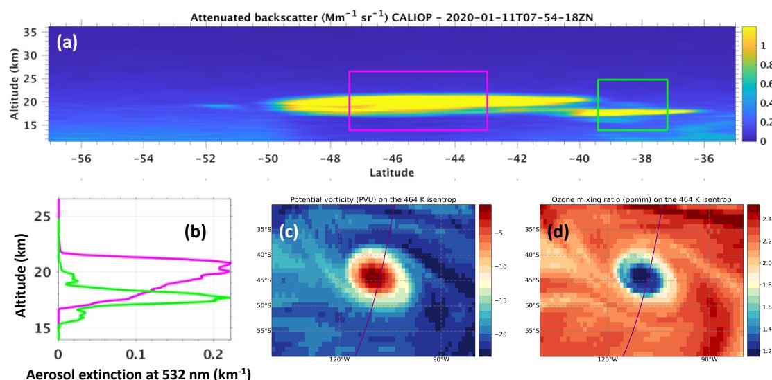
Figure 3: CALIOP attenuated backscatter observations at 532 nm for the main vortex overpass of 11 January 2020 (panel a) and aerosol extinction profiles averaged in the magenta and green boxes individuated in panel a, in respective colours (panel b). The
