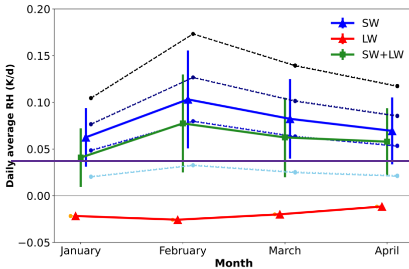
335 Figure 5: Time series, from January to April 2020, of the monthly mean area-weighted Southern-Hemispheric HR, based on equinox-equivalent daily-average HR of Fig. 4), for the UTLS perturbation of Australian fires in 2019–2020. The radiative heating profiles are averaged in the altitude range 12–25 km. Different shades/types of blue dots and lines are for different SSA and g values – the darker the shade the smaller the SSA, dashed/dotted lines for larger and smaller g, see caption of Fig. 4 for details. Different types of orange dots and lines are for different g values – dashed/dotted lines for larger and smaller g, see caption of Fig. 4 for details. The HR values, averaged over all SSA and g scenarios, for different spectral ranges are also in different colours: SW: 340 blue triangles with error bars and lines, LW: red triangles with error bars and lines, net SW+LW: green squares with error bars and lines. The error bars are representative of the variability of the average SW, LW and SW+LW monthly means radiative heating due to SSA and g variability.
