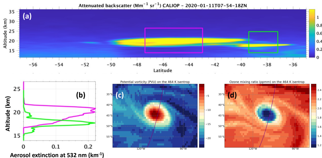
260 Figure 3: CALIOP attenuated backscatter observations at 532 nm for the main vortex overpass of 11 January 2020 (panel a) and aerosol extinction profiles averaged in the magenta and green boxes individuated in panel a, in respective colours (panel b). The CALIOP overpass of the vortex, individuated-identified by means of ECMWF-IFS potential vorticity and ozone mixing ratio anomalies (at 464 K isentropic level, about 18 km altitude) , is shown as the violet track in panel c and d, respectively.
