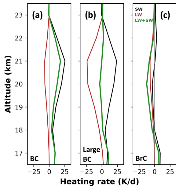
Figure 6: In-vortex SW, LW and net SW+LW HR for the CALIOP overpass of the main vortex on 11 January 2020 (CALIOP overpass shown in Fig. 3), with 3 assumed scenarios for the unmeasured aerosol properties: Black carbon (BC, SW SSA: 0.80, SW g: 0.5-0.7, LW SSA: 0.20, LW g: 0.3, panel a), Large black carbon (Large BC, SW SSA: 0.80, SW g: 0.7, LW SSA: 0.20, LW g: 0.5, panel b) and Brown carbon (BrC, SW SSA: 0.90-0.95, SW g: 0.7, LW SSA: 0.20, LW g: 0.5, panel c). These 3 cases are defined in a consistent manner as in S22.
