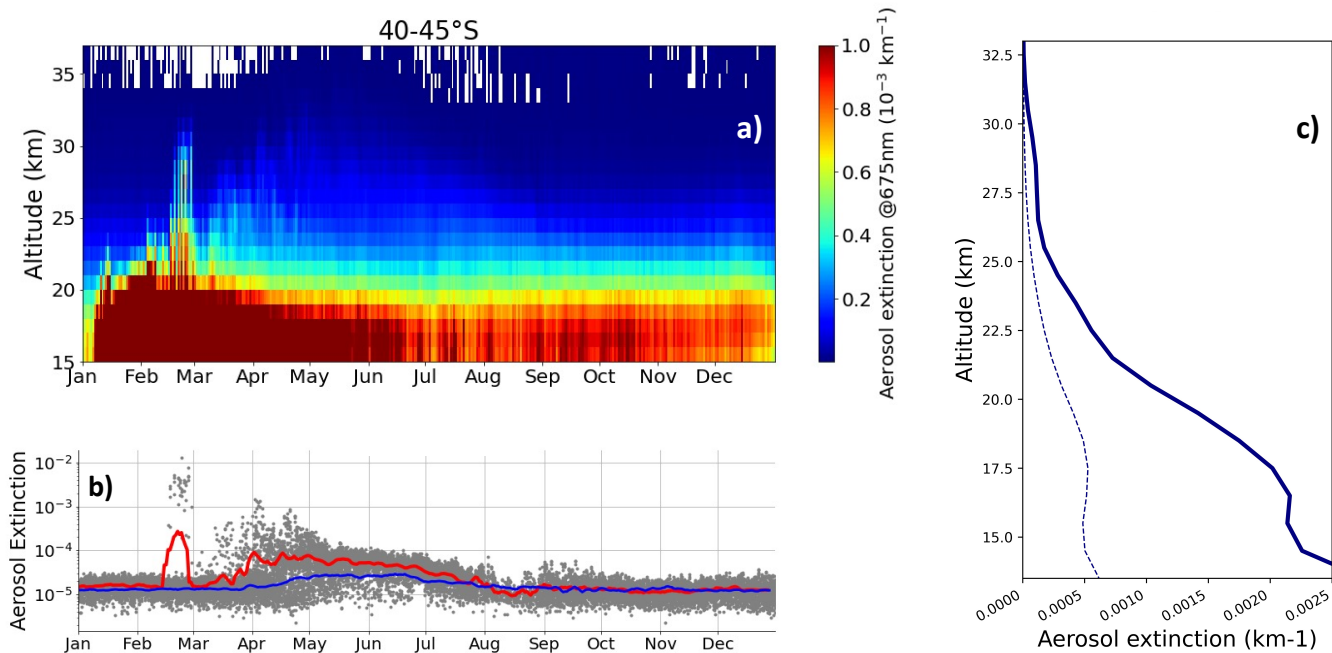
225 Figure 2: OMPS-LP observations at 675 nm in the latitude interval 40-45°S: time series of the zonal average vertical profiles of the aerosol extinction in 2020 (panel a), individual aerosol extinction coefficient observations at 28 km altitude (panel b), monthly mean aerosol extinction coefficient profiles in February 2020 (perturbed profiles, solid lines) and February 2019 (background profiles, dashed lines) (panel c). In panel b, temporally smoothed time series for 2020 (red curve) and 2019 (blue curve) are also shown.
