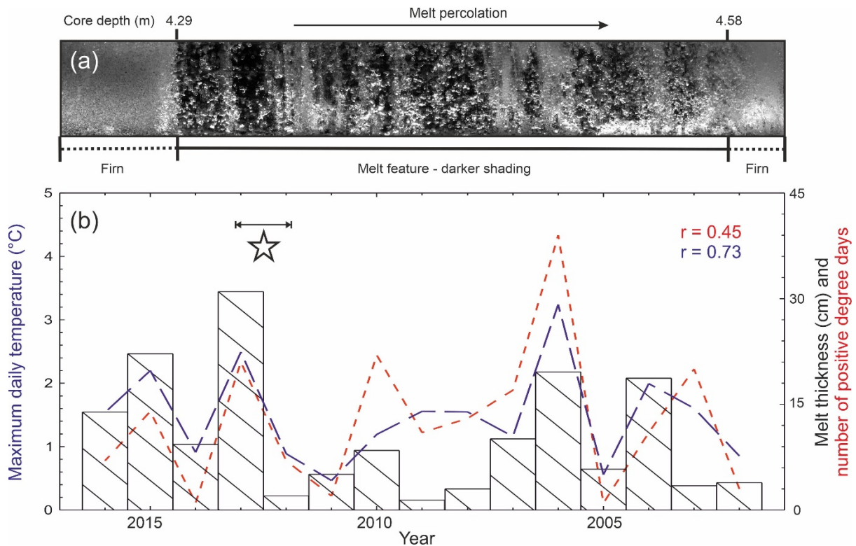
210 Figure 4. (a) Line scanned image of the Peter 1 st firn core. Highlighting the prominent melt feature, observed as a dark area (higher density) between 4.29-4.58 m depth, compared to the lighter shaded (lower density) areas corresponding to firn. (b) Comparison of the annual melt thickness (black bars, cm) in the firn core with the number of positive degree days (red, temperature > 0.5°C) and the maximum daily temperature (blue, °C) from ERA5. Star highlighting the location of the melt feature (a), which is observed in the 2012 layer, but assigned to 2013 due to the 215 downward percolation of meltwater generated during January 2013.
