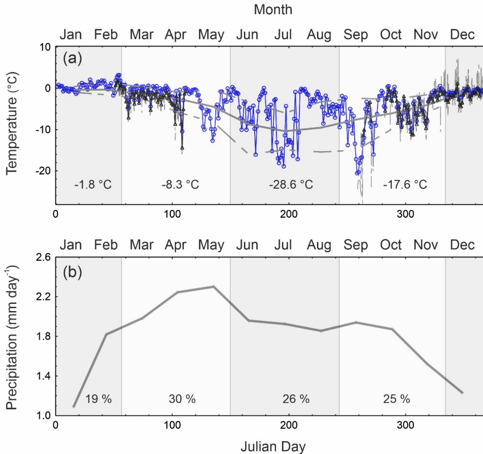
Figure 5: Seasonal cycle in temperature (a) and precipitation (b) at Peter 1 st Island from ERA5 reanalysis (grey curve) (2002-2016 CE). Dashed grey curve represents 2.5 % and 97.5 % percentiles for temperature (a). Daily average temperatures during 2006 CE from ERA5 (blue circle) and AWS (black triangle), with hourly AWS temperature shown in thin grey curve. Grey shading highlights the seasons, with the corresponding average temperature and percentage of precipitation shown. AWS data available from University of Wisconsin-Madison Automatic Weather Station Program.
