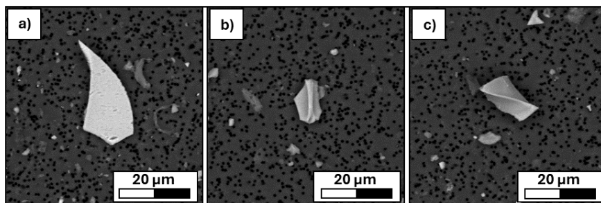
195 Figure 3: Shards identified from the interval 4.6-4.9 m depth, displaying typical cryptotephra morphology. The images were obtained using a Quanta-650F scanning electron microscope (SEM) at the Earth Sciences Department of the University of Cambridge. Each filter was imaged at x800 magnification using backscattered electron imagery (BSEI) in a low-pressure mode.
