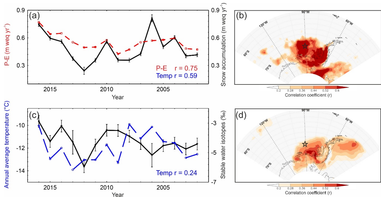
Figure 6: (a) Peter 1 st annual average snow accumulation (solid black), compared with precipitation-evaporation (P-E) (dashed blue) from ERA5 reanalysis data (2002-2016). Corresponding correlation coefficients (r) for snow accumulation and P-E (red) and snow accumulation with 2m temperature (blue). (b) Spatial correlation plot of annual snow accumulation with annual ERA5 P-E (all coloured areas p>0.05). (c) Annual average stable water isotope ( \delta^{18}\text{O} ) (solid black), compared with annual average 2 m temperatures from ERA5 (blue dashed). Correlation coefficient (r) between annual \delta^{18}\text{O} and annual average 2 m temperature (blue). (d) Spatial correlation plot of annual \delta^{18}\text{O} with annual ERA5 2m temperature (all coloured areas p.0.05). All annual averages calculated as December to November. Uncertainty bars are one standard error ( \sigma ), for all years except 2006 and 2012, where 2\sigma are applied to account for additional uncertainties relating to melt.
