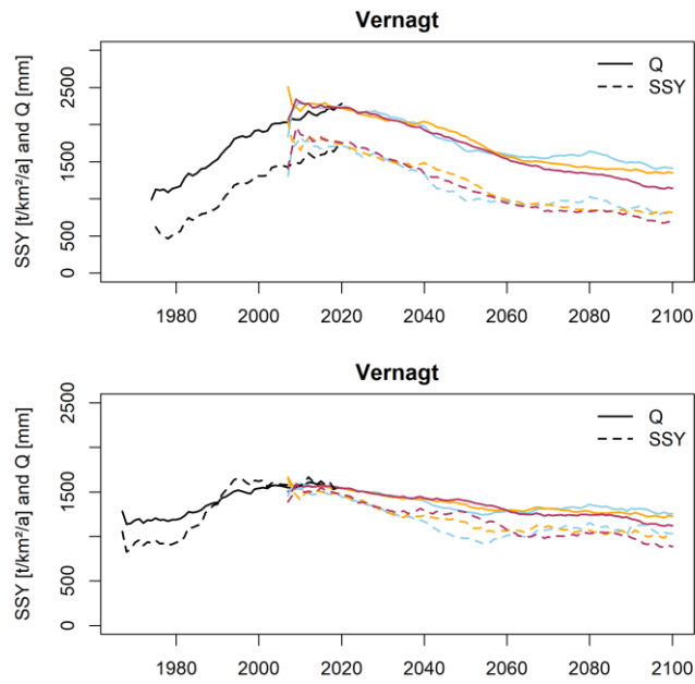
This will be the new figure 11, showing the estimated timings of peak water and peak sediment. Black lines indicate past mean annual Q from measurements and mean annual SSY estimates of QRF model; colored lines correspond to different RCPs (compare to Figure 10). Underlying data have been smoothed using a 15-year moving average.
