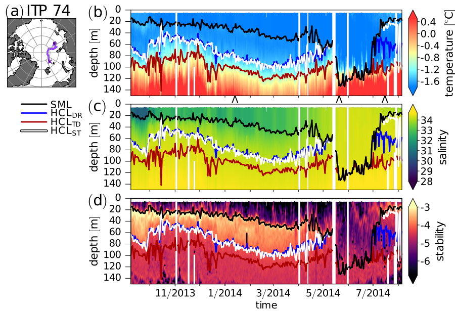
Figure 2. ITP-74 location of measurements (a) and time series of temperature (b), salinity IP (in the practical salinity scale) (c), and vertical stability IP ( L , unitless, see Sect. 2.1.3) (d). The circle and the cross in (a) mark the beginning and the end of the ITP-74 track, respectively. The colored lines in (b–d) are the base of the SML (black) and the halocline (HCL) base depths derived by the DR method (blue), the TD method (red) and the ST method (white). IP Salinity is given in the practical salinity scale. Individual profiles at the location of the wedge symbols ( \wedge ) below the x-axis in (b) are shown in Fig. 3. Profiles that started below 15 m were excluded (only) in this figure (but nowhere else), because this increased readability by reducing the effect of noise in determining the SML base without affecting the overall result.
