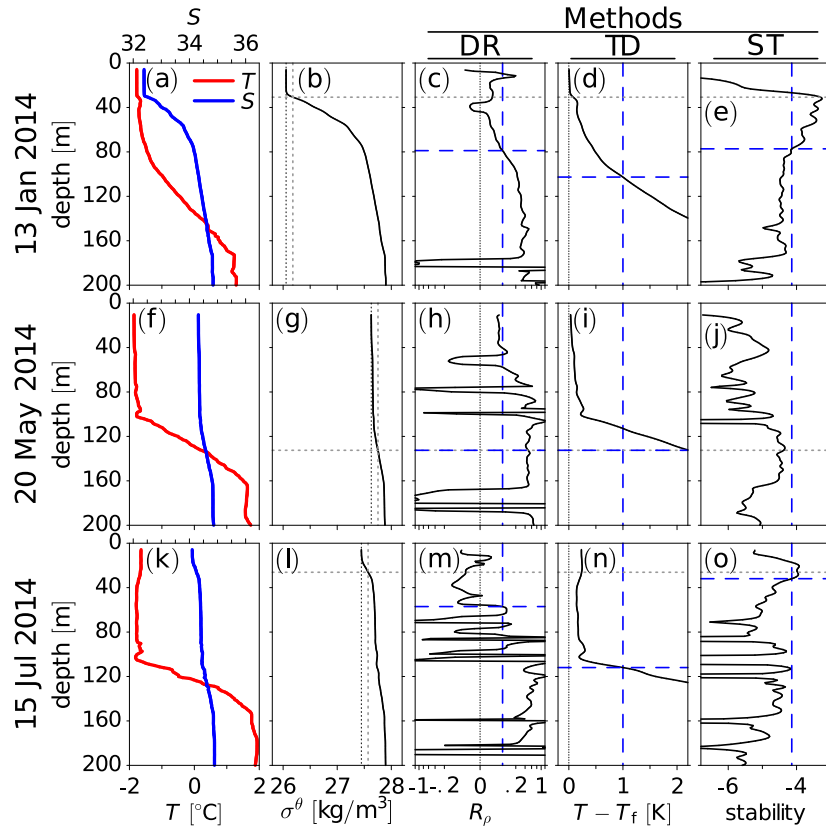
Figure 3. Please note: Added profiles of potential density anomaly and fixed overlapping labels. Temperature T and salinity S^{\text{M.A and LP}} (a, f, k), potential density anomaly \sigma^\theta = \rho^\theta - 1000 \text{ kg m}^{-3} , where \rho^\theta is potential density (b, g, l), density ratio R_\rho (please note the cubic scaling of the x-axis) (c, h, m), temperature difference T - T_f , where T_f is the freezing temperature (d, i, n), and stability L (e, j, o) from ITP-74 before winter convection on 13 January 2014 (a–e)–(a–d), during winter convection on 20 May 2014 (f–j)–(e–h) and after winter convection on 15 July 2014 (k–o)–(i–l). M.A and LP Vertical dotted lines in b, g, l indicate the surface density anomaly and the threshold for determining the SML base (i.e. surface density plus 0.125 \text{ kg m}^{-3} ). Horizontal dotted lines indicate the SML base. Vertical dashed lines indicated threshold values for determining the halocline base. Horizontal dashed lines indicate the halocline base determined by the three different methods. M.A and LP Dotted lines indicate the SML base. LP Dashed lines overlying dotted lines in h(f) and j(k) indicate that a threshold for identifying the halocline base was exceeded at the SML base.
