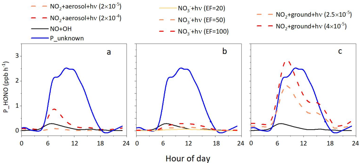
Figure 6: HONO production rates by different HONO formation pathways with different parameter settings. (a) photo-induced NO 2 conversion on the aerosol surface; (b) heterogeneous particulate nitrate photolysis; (c) photo-induced NO 2 conversion on the ground surface.
