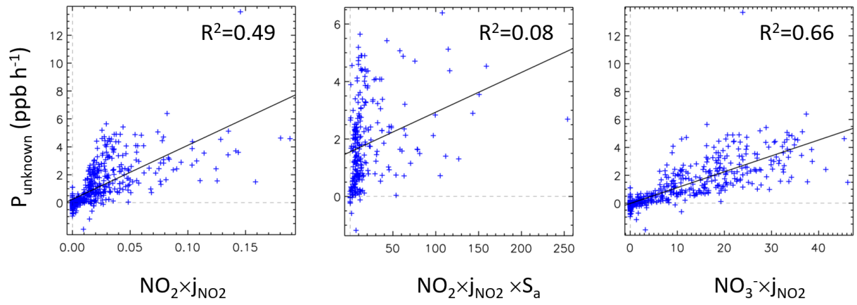
1025 Figure 5: The unknown source strength ( P_{\text{unknown}} , 8:00-18:00) plotted against \text{NO}_2 \times j_{\text{NO}_2} , \text{NO}_2 \times j_{\text{NO}_2} \times S_a and \text{NO}_3^- \times j_{\text{NO}_2} .
