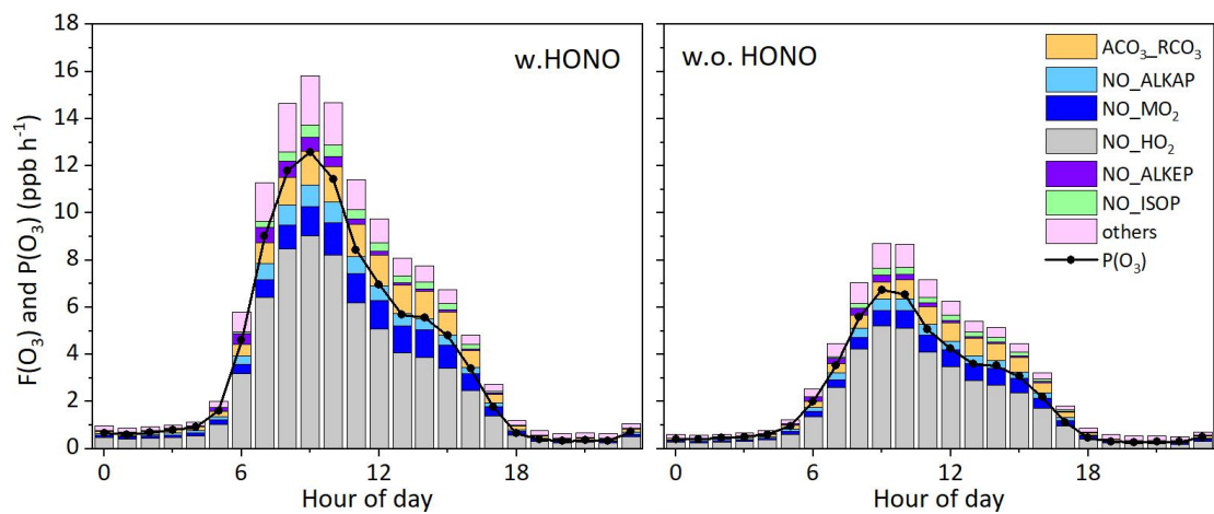
Figure 12: Model-calculated total and net O 3 production rate with and without observed HONO as a model constraint. According to different type of VOC precursors, organic peroxy radicals (RO 2 ) can be classified into seven categories, including methyl peroxy radicals (MO 2 =CH 3 O 2 ), first-generation peroxy radicals from alkanes (ALKAP), 1165 alkenes except isoprene (ALKEP), isoprene (ISOP), aromatics (AROP), OVOC (OVOCP) and acyl peroxy radicals (ACETYLP=ACO 3 +RCO 3 ).
