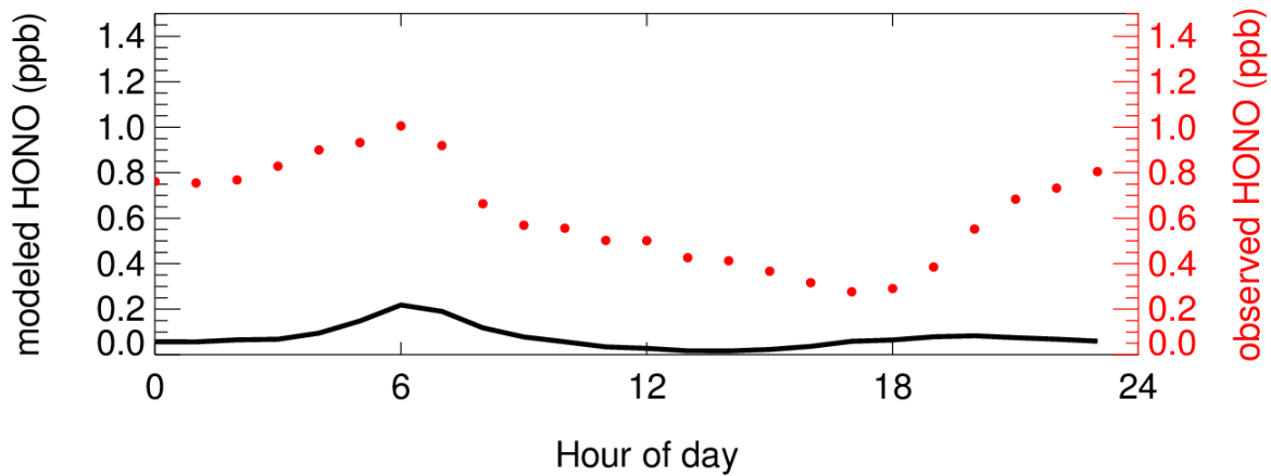
Figure 4: The modeled HONO concentration with only default HONO source (OH+NO).
