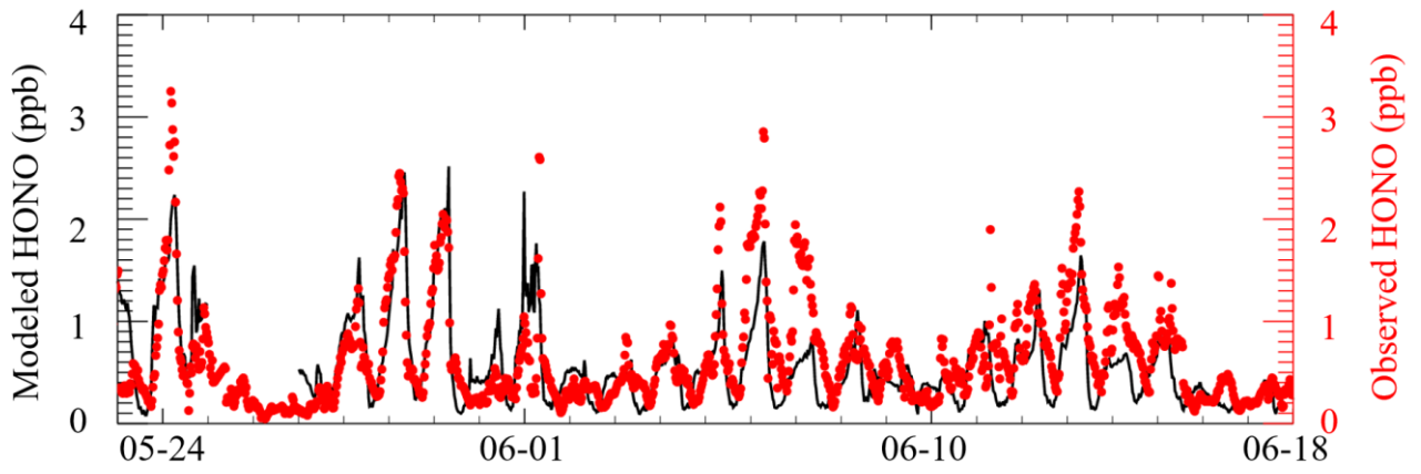
1110 Figure 9: Time series of modeled and observed HONO concentrations from 05-23 to 06-18.
