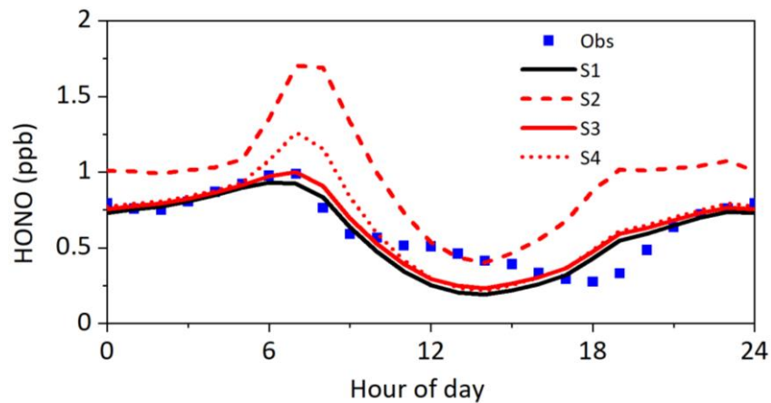
1085 Figure 8: Results from sensitivity tests compared with observed HONO concentrations. S1: parameters were listed in Table 1; S2: \gamma_{\text{ground+hv}} was changed to 6 \times 10^{-5} compared to S1; S3: \gamma_{\text{aerosol+hv}} was changed to 2 \times 10^{-4} compared to S1; S4: EF was changed to 120 compared to S1.
