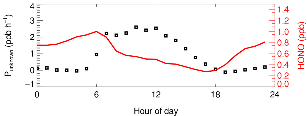
Figure 3: The diurnal profiles of calculated HONO unknown source ( P_{\text{unknown}} ) strength and observed HONO.
