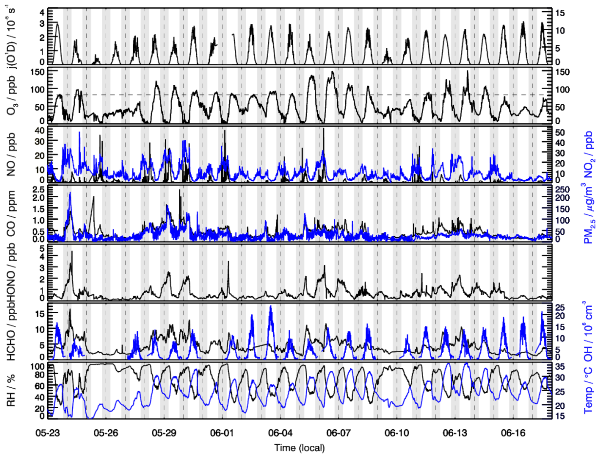
955 Figure 1: Time series of HONO, O 3 , CO, PM 2.5 , OH, HCHO, NO x , relative humidity (RH), temperature and j(O 1 D) during the EXPLORE-YRD campaign.
