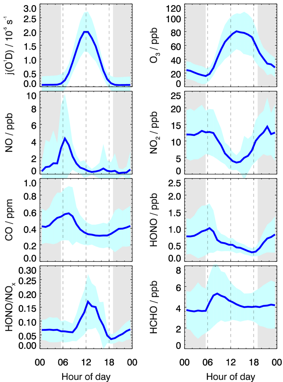
Figure 2: The diurnal patterns of HONO, HONO/NO x , NO, NO 2 , CO, O 3 , HCHO and j(O 1 D).
