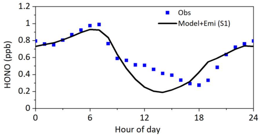
1060 Figure 7: Modeled HONO concentrations with additional HONO sources compared to the observations. Model+Emi 1065 represents the sum of modeled HONO and vehicle HONO emission.
