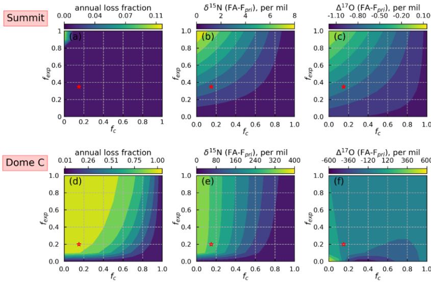
Figure 8. Model sensitivity test results of two parameters f_{\text{exp}} and f_c for Summit (a-c) and Dome C (d-f). The annual nitrate loss fraction is defined as 1-FA/F_{\text{pri}} following Jiang et al. (2021). Red stars represent the values of f_{\text{exp}} and f_c used in model simulations.
