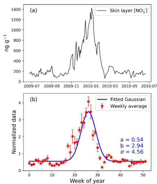
895 Figure D1. (a) Observed annual variations of skin layer nitrate concentration at Dome C (Erbland et al., 2013). (b) Normalized skin layer nitrate concentration by its arithmetic mean and the fitted Gaussian curve, with the shape parameters ( a , b , \sigma ) 900 labeled in blue text.
