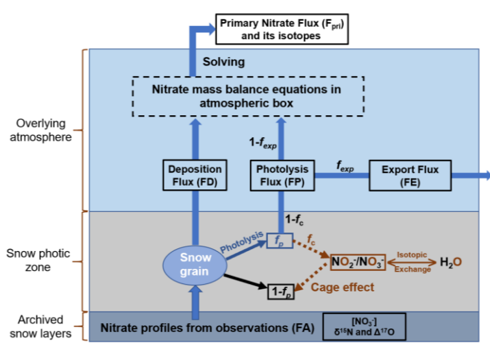
170 Figure 1. Schematic plot of the model domains of the inverse model including the atmospheric box, the snow photic zone and the archived snow layers, where f_{exp} represents the fraction of nitrate exported from the site of photolysis. The nitrate isotopic and mass balance relationships on snow grains during photolysis are also shown, where f_p represents the fraction of snow nitrate being photolyzed, and f_c 175 represents the fraction of photolyzed nitrate experiencing the cage effect (i.e., exchange of oxygen isotopes with snow water). FA represents the archived nitrate flux.
