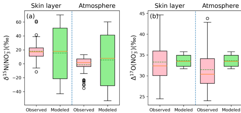
605 Figure 6. Comparison between the observed and modeled annual averages of \delta^{15}\text{N}(\text{NO}_3^-) and \Delta^{17}\text{O}(\text{NO}_3^-) in the atmosphere and snow skin layer at Dome C. The solid line in the box plot indicates the median value, while the dash line represents the average value.
