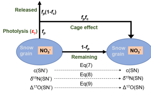
Figure A1. Sketch of the mass and isotopic transfer relationship during nitrate 850 photolysis in snow grains. The black italic variables near the arrows indicate the fractional change in each subprocess.
