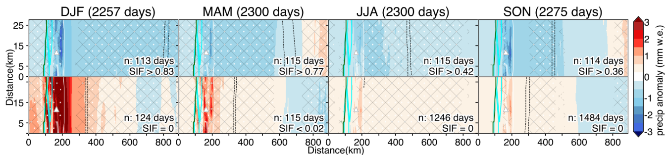
575 Figure 9. Composite of precipitation (precip in mm w.e.) anomalies from RACMO corresponding to zonally (overall grid cells) averaged (median) SIF over the Greenland Sea for entire daily measurements for the given season (1996–2020). The upper and lower panels represent precipitation anomaly corresponding to high and low SIF days i.e., n number of days when SIF exceed and is less than or equal to the indicated SIF values, respectively, for each season. The figure is the zoomed-in version of the black rectangle in Fig. 1 encompassing the ZR; the location of the stations (triangle), the land-sea border (white contour), peripheral glacier (cyan contour), and the GrIS (green contour) are indicated. The average sea-ice extent (dashed black line) for the given condition is also shown; the outer line represents 0.25 SIF and the inner line 0.3. The white dots and areas within the black mesh indicate statistically significant differences between high and low composite anomalies at the 0.05 and 0.1 significance levels, respectively
