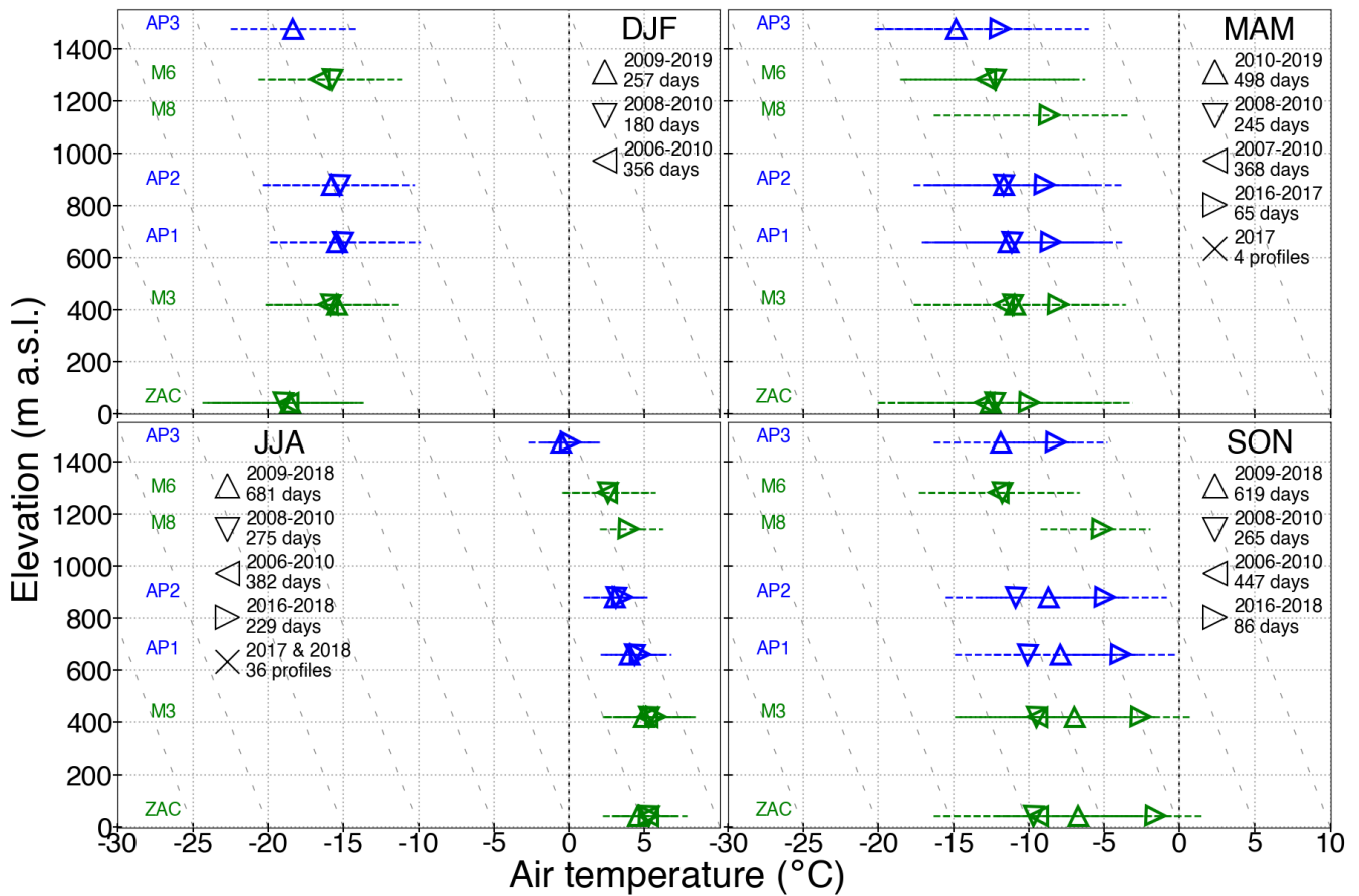
205 Figure 3. Mean air temperature measurements from AWSs and UAV against the elevation. Each marker (except for the cross) represents the daily mean temperature of a station for temporally overlapping periods, as shown in the legend, with other AWSs measurements for each season. The 25th and 75th percentiles of air temperature are indicated by the dashed horizontal line passing across the marker. Blue and green colors represent stations on ice and ice-free surface, respectively. The mean vertical temperature profile measurements from UAV taken in 2017 (black line) and 2018 (solid grey line) are shown (in MAM and JJA panel) after applying Savitzky Golay low-pass filter to remove the high-frequency fluctuation of air temperature due to the high temporal resolution of UAV. The shaded area around the line represents the 25th and 75th percentiles of the temperature at the given elevation from all vertical profiles. The ‘X’ marker represents the sub-daily temperature of a station temporally overlapping with the UAV flight period. In each panel the mean environmental lapse rate (dashed grey line) of 6.5\text{ °C km}^{-1} is plotted for reference 210
