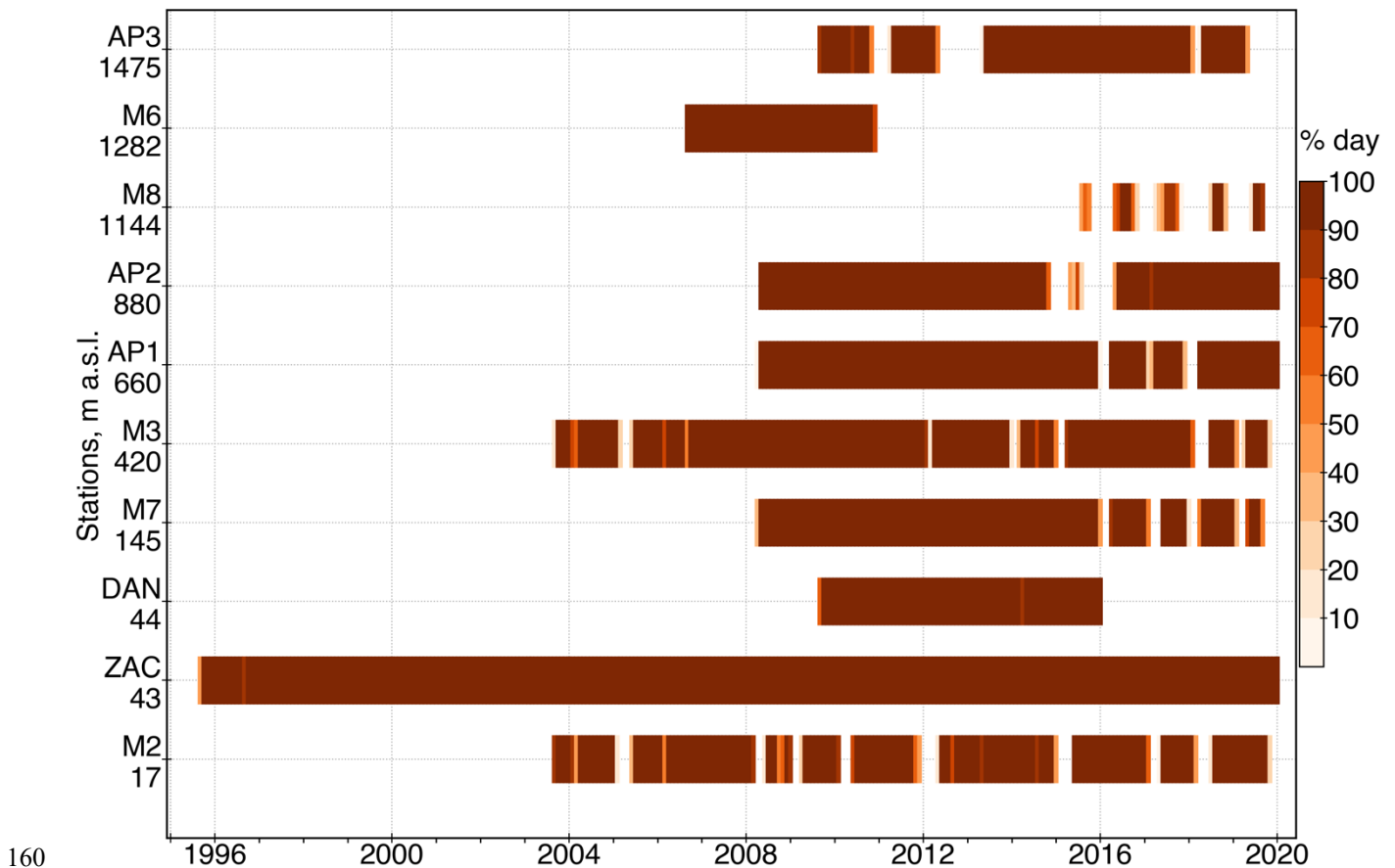
Figure 2. Temporal coverage of all AWSs located in the ZR and on the APO and the elevation of each station in meters above mean sea level (m a.s.l.). The color bar indicates the percentage of days with air temperature data during a respective month for each AWS after screening
