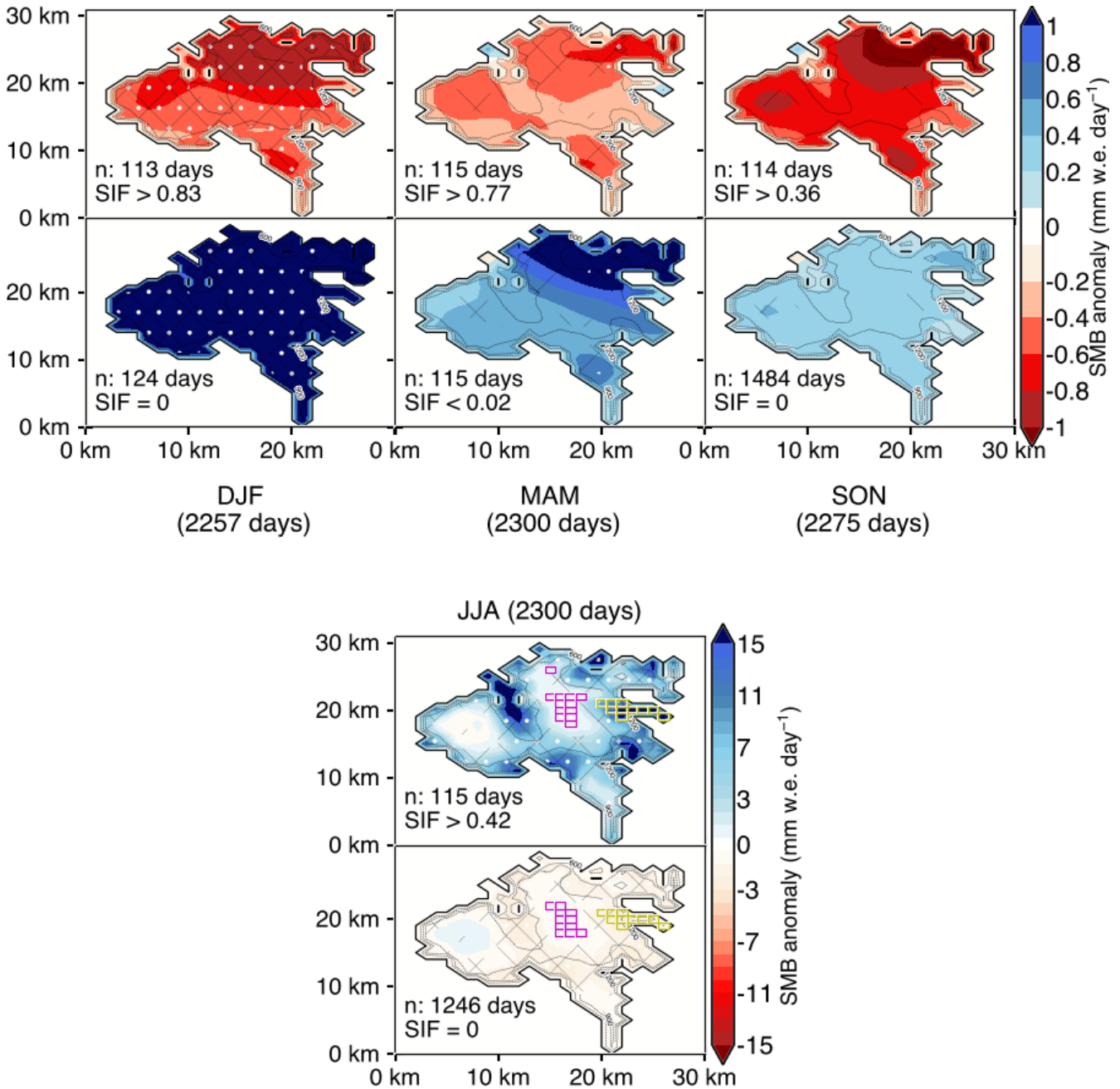
605 Figure 11. Idem as Fig. 9, but for the composite of daily surface mass balance (SMB in mm w.e. day -1 ) anomalies of A.P. Olsen Ice Cap (APO), (location in Fig. 1) from RACMO. In JJA panel, the magenta and yellow rectangles indicate the grid cells whose values are used for the calculation of the average SMB anomaly on accumulation (>1100 m a.s.l.) and ablation (<1100m a.s.l.; only the southeastward flowing outlet glacier) area, respectively, of the APO. Note the use of a separate color bar for summer composite due to large mass overturn
