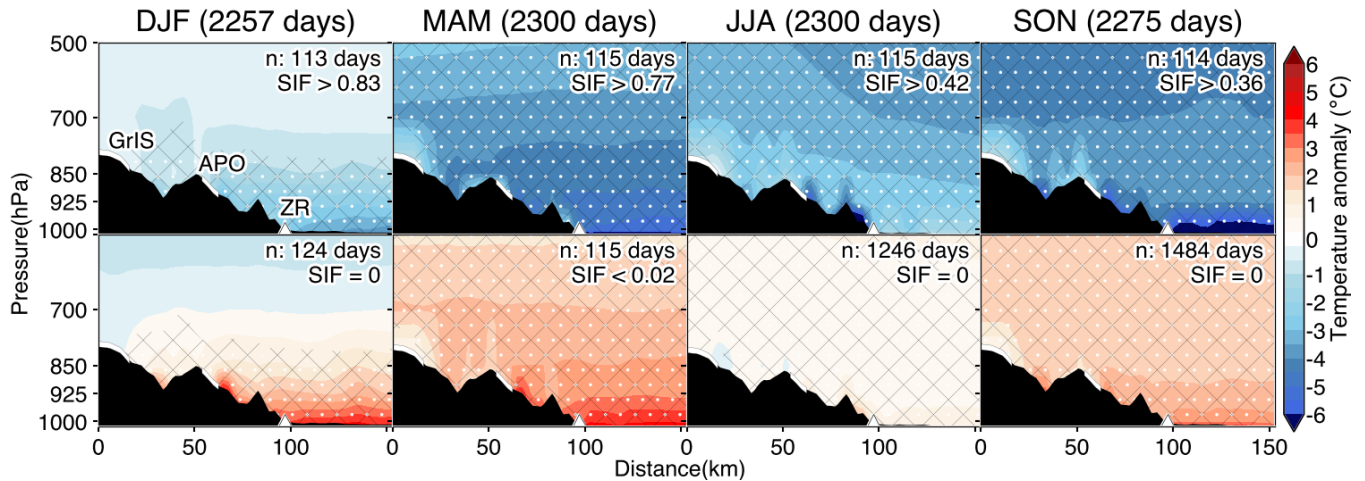
590 Figure 10. Idem as Fig. 9, but for the composite of the cross-sectional transect (XY as shown in Fig. 1) of vertical air temperature (T in °C) anomalies profile. The portions of the Greenland Ice Sheet (GrIS), A. P. Olsen Ice Cap (APO), and the Zackenberg region (ZR) passing through the transect are labelled in the upper panel of DJF season.
