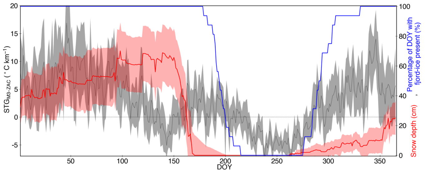
435 Figure 5. Annual cycle of STG between ZAC and M3 ( STG_{M3-ZAC} in ^{\circ}\text{C km}^{-1} ) and snow depth (in cm) measured at ZAC for 2004–2019. The black and red lines denote the daily mean STG_{M3-ZAC} and snow depth, and the grey and red shaded areas denote a 95 % confidence interval around the given mean, respectively. The blue line represents the percentage of the respective day of the year (DOY) during observation period (2004–2019) with fjord-ice present in Young Sound. The leap year day 29 February is excluded
