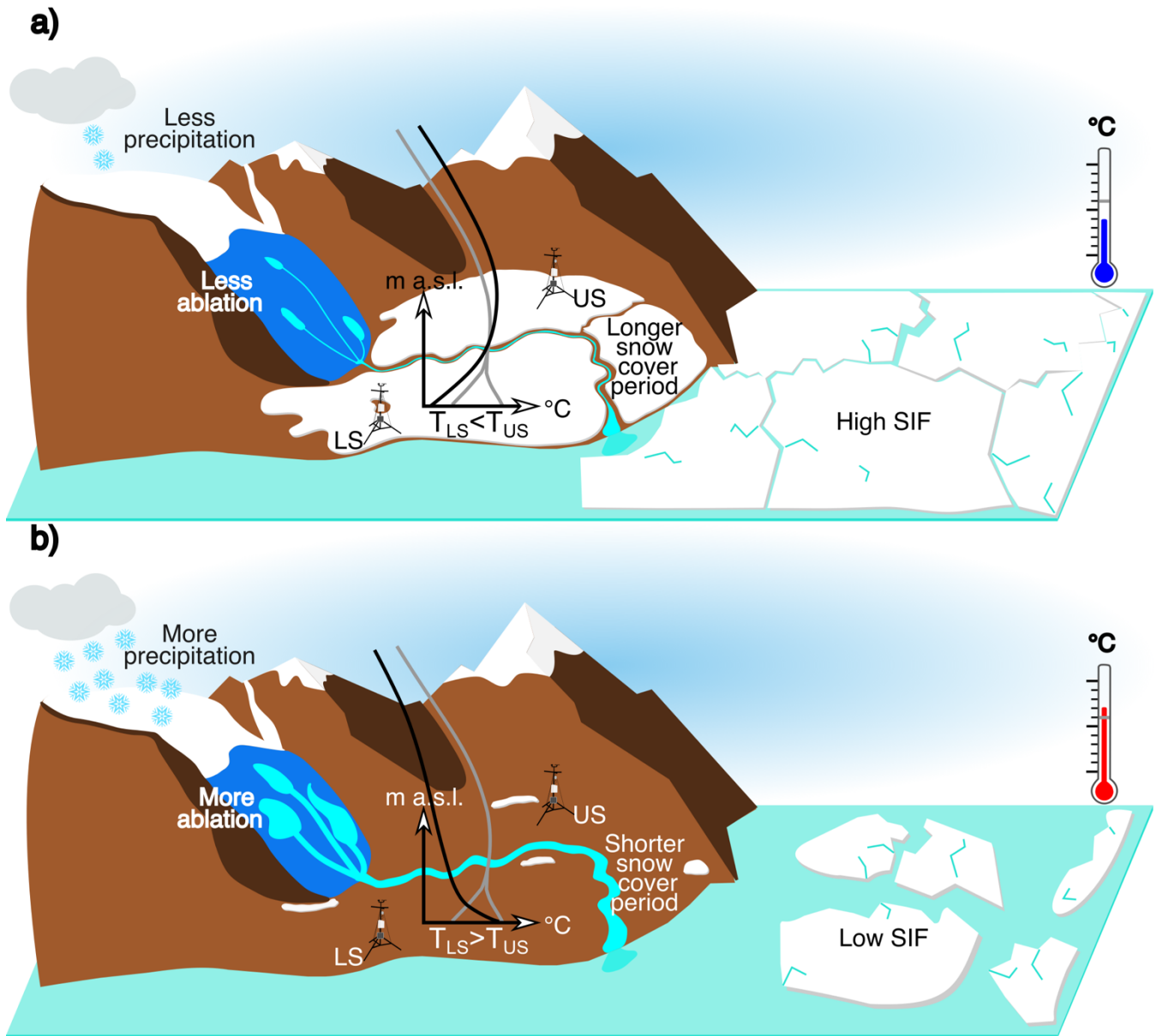
680 Figure 12. A schematic representation of some important linkages in the Zackenberg region (ZR), fractional sea-ice cover (SIF) in the Greenland Sea, and surface condition of A. P. Olsen Ice Cap (APO) especially for the summer season. The temperature at the 685 lower station (LS), T_{LS} , can be higher or lower than the temperature at the upper station (US), T_{US} . (a) The upper panel shows the conditions when STG_{US-LS} is shallow ( T_{LS} is less than T_{US} ; less negative or positive (inversion) STG_{US-LS} ), when there is more snow in the valley, when SIF is high, along with low precipitation amounts, and little snow/ice ablation at APO. (b) The lower panel shows the opposite conditions when STG_{US-LS} is steep ( T_{LS} is more than T_{US} ; more negative or less positive STG_{US-LS} ), when there is less snow in the valley, when SIF is low, along with high precipitation amounts, and strong snow/ice ablation at APO. The solid grey line represents a climatological mean of the temperature profile in the ZR and the corresponding solid black lines represent the mean temperature profile in each condition
