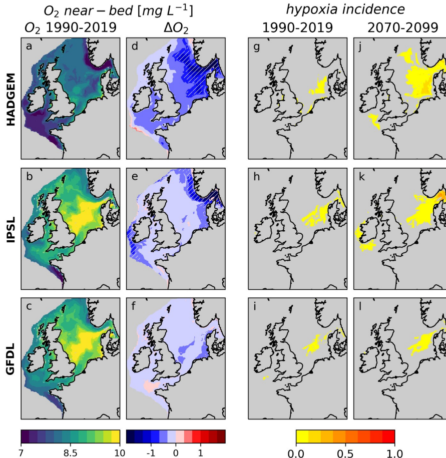
340 Fig. 3. Near-bed O 2 concentration, present state (average of 1990-2019) and change (difference of the 2070-2099 and 1990-2019 averages) and fraction of year with average near-bed Oxygen < 6 mg L -1 under present day and future conditions, calculated on bias-corrected data. Hatched regions in d, e, f are deoxygenation hotspots.
