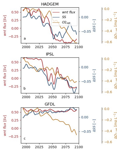
440 Fig. 9. Temporal evolution of \Delta SS and \Delta O_{2,sat} in the Norwegian Trench and Western Norwegian Trench current flux; monthly average data are smoothed with a Gaussian filter. Positive values of the current are entering the North Sea.
