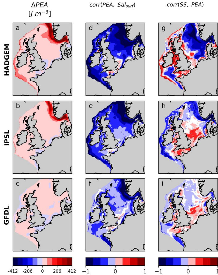
Fig. 6. Change in potential energy anomaly (PEA) and correlation between PEA and surface salinity and PEA and SS. 390 White areas on the shelf indicate non-significant correlation.
