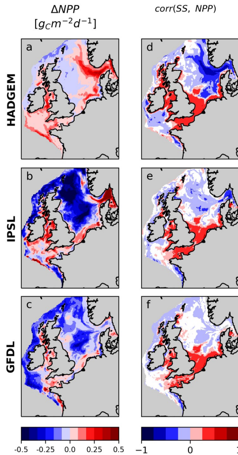
Fig. 7. Change in depth integrated net primary production (NPP) and correlation between NPP and SS. w White areas on the shelf indicate non-significant correlation.
