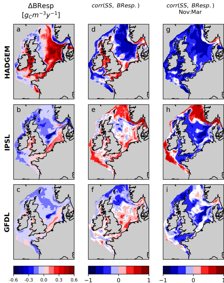
425 Fig. 8. Change in near-bed BResp and correlation between BResp and SS for all months and for months from November to March alone. White areas on the shelf indicate non-significant correlation.
