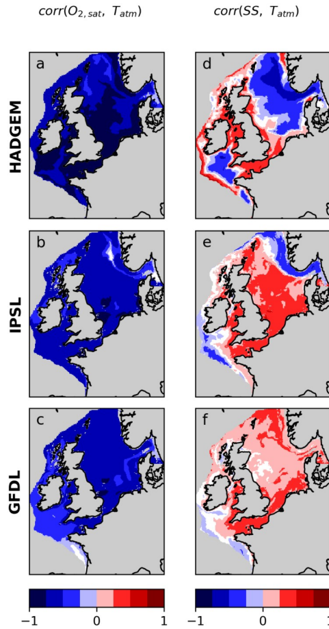
375 Fig. 5. Correlation between temperature atmospheric forcing and near-bed O_{2,sat} and SS. White areas on the shelf indicate non-significant correlation.
