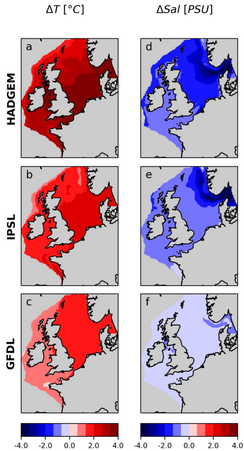
325 Fig. 2. Surface temperature and salinity, difference between future (2070-2099) and present (1990-2019) periods.
