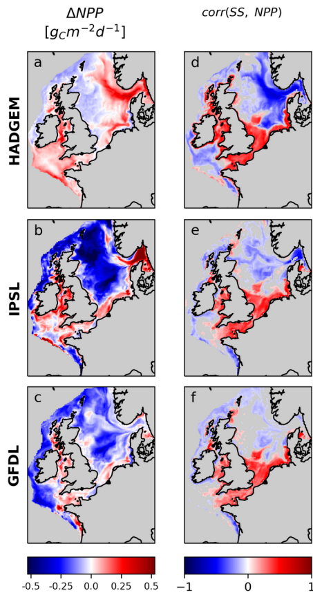
Fig. 98. Change in depth integrated net primary production (NPP) and correlation between NPP and SS_{O_2} .
