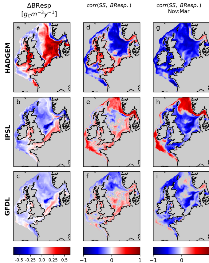
Fig. 109. Change in near-bed bacterial respiration and correlation between BResp and SS_{O_2} for all months and for months from November to March alone.
