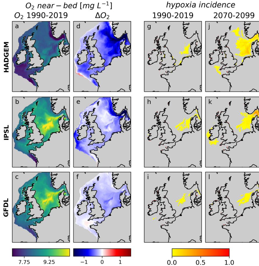
Fig. 4. Near-bed O_2 concentration, present state (average of 1990-2019) and change (difference of the 2070-2099 and 1990- 400 2019 averages) And fraction of year with average near-bed Oxygen < 6 \text{ mg L}^{-1} under present day and future conditions, calculated on bias-corrected data.
