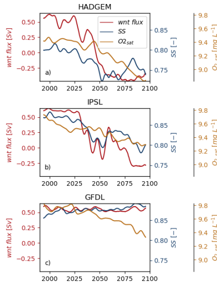
520 | Fig. 140. Temporal evolution of SS_{e2} and O_{2,sat} in the Norwegian Trench and Western Norwegian Trench current flux; monthly average data are smoothed with a Gaussian filter. Positive values of the current are entering the North Sea.
