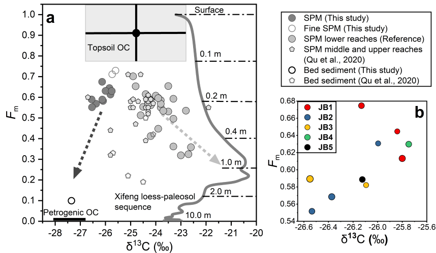
400 401 Figure 5: (a) ^{14}\text{C} activity (expressed as Fm) vs. \delta^{13}\text{C} for a compilation of POC data collected over the 2011-2016 period in 402 the lower Huanghe, including samples from this study and previous studies at Huayuankou, Lijin, and Kenli (Hu et al., 403 2015; Tao et al., 2015; Yu et al., 2019a; and Ge et al., 2020); SPM and bed sediment (BS) collected by Qu et al., 2020 at 404 Toudaoguai (most downstream location of the upper reaches) and Longmen in the middle reaches (Table S1). The grey 405 curve corresponds to \delta^{13}\text{C}_{\text{org}} of the top 10 m of the Xifeng loess-paleosol (Ning et al., 2006), and the corresponding Fm was 406 calculated from ^{10}\text{Be} -derived ages following 'Age = -8033 \cdot \ln(\text{Fm}) '. The soil depth is marked above the dot-dash line (Zhou 407 et al., 2010). Topsoil OC represents OC from the upper 10 cm of the loess-paleosol sequence with standard deviation marked
