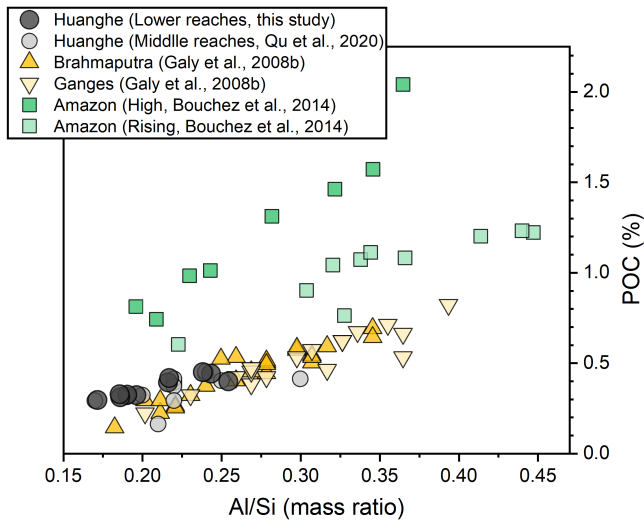
333 334 Figure 4: "POC loading" of river SPM of large rivers. The POC loading is estimated from the slope of the relationship 335 between POC content and the Al/Si ratio of each fluvial system (Galy et al., 2008b). All SPM samples were collected along 336 depth profiles except for the middle Huanghe (Qu et al., 2020).
