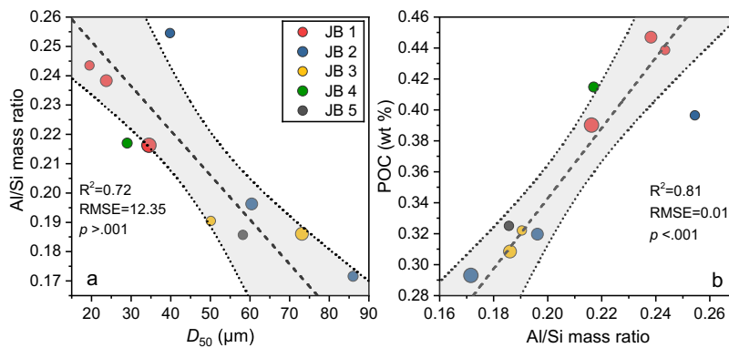
291 Figure 3: Relationships between (a) particle size D_{50} and Al/Si mass ratio; (b) Al/Si mass ratio and POC content for the 292 Luokou cross-section on the Huanghe (July 17, 2016). The symbol size indicates the sampling depth in the water column, 293 with symbol size increasing with depth. The shaded area represents the 95% confidence area of the linear best-fit (black 294 dashed line), the upper and lower bound are marked by grey dotted lines. 295
