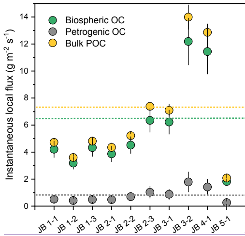
706 Figure 8: Estimates of instantaneous “local” fluxes of Huanghe bulk POC, \text{OC}_{\text{bio}} and \text{OC}_{\text{petro}} , calculated for each sample of 707 the Luokou cross-section. The three dotted lines marked in orange, green, and grey represent the corresponding 708 instantaneous, cross-section integrated fluxes. The error bar represents 1 standard deviation. 709
