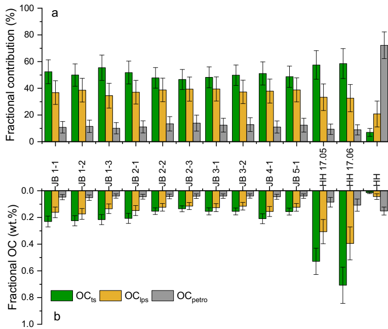
538 Figure 7: (a) Relative contributions of the three different sources of Huanghe POC, (b) fractional OC weight percentage 539 Huanghe POC at the Luokou cross-section, as inferred from a mixing model. OC ts is the topsoil-derived OC, OC lps 540 represents the loess-paleosol sequence OC excluding topsoil, and OC petro is the rock-derived OC eroded from the Huanghe 541 middle reaches. 542
