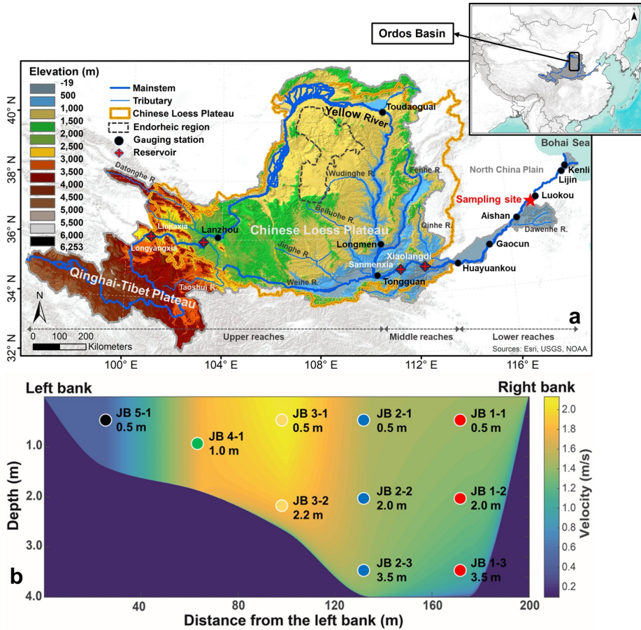
135 136 Figure 1: (a) Elevation map of the Huanghe drainage basin showing the main reservoirs and gauging stations along the 137 main stem as well as our sampling site (36.75°N, 117.02°E, near the Luokou gauging station); and (b) channel cross-section 138 sampled for this study showing the depth and lateral distribution of suspended particulate matter (SPM) samples and 139 modeled velocity distribution based on the "law of the wall", using the point velocity data measured by a current velocity 140 meter attached to the sampler.
