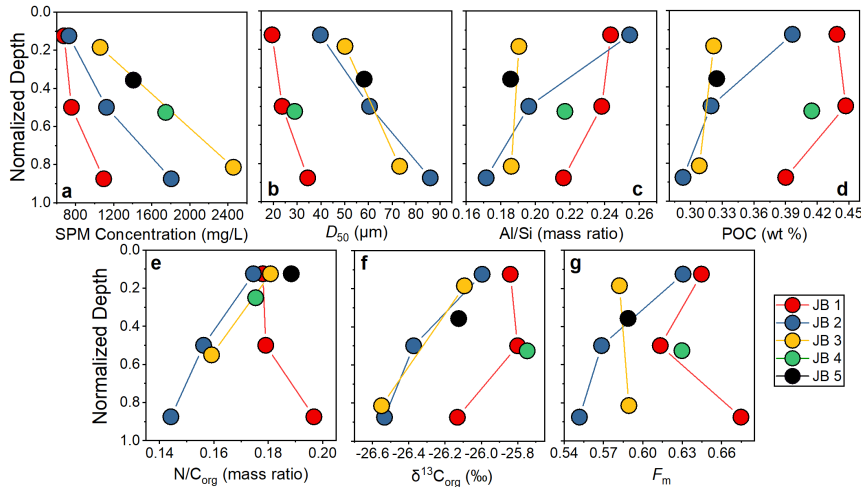
269 270 Figure 2: Variation of physical and chemical parameters in the river cross-section, shown as a function of sampling depth 271 normalized to total depth of the water column at the location of the considered depth-profile, for the Luokou cross-section 272 on the Huanghe (June 16, 2017). (a) SPM concentration; (b) particle size distribution (shown as D50); (c) Al/Si mass ratio; 273 (d) POC content (weight %); (e) N/C org mass ratio; (f) stable carbon isotope ratio \delta^{13}C_{org} (‰); (g) radiocarbon activity F_m .
