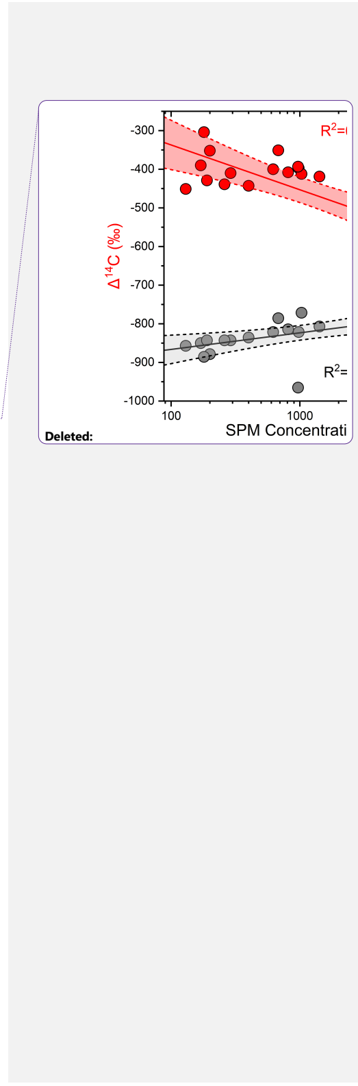
Figure 6: ^{14}\text{C} activity (expressed as Fm; red circles) and \delta^{13}\text{C} (grey circles) of POC vs. SPM concentration for surface samples from the Huanghe collected from 2011 to 2016 (average SPM concentration of surface samples in this study and from Hu et al. (2015), Tao et al. (2015), Yu et al. (2019a), and Ge et al. (2020)). These paired dual carbon isotope data corresponds to the group 'SPM lower reaches' in Figure 5. Straight lines correspond to best-fit logarithmic curves, and shaded areas represent the 95% confidence interval.
